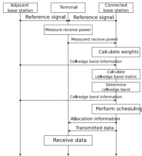
Fig. 57: Sequence diagram of Distributed Frequency Reuse Scheme
