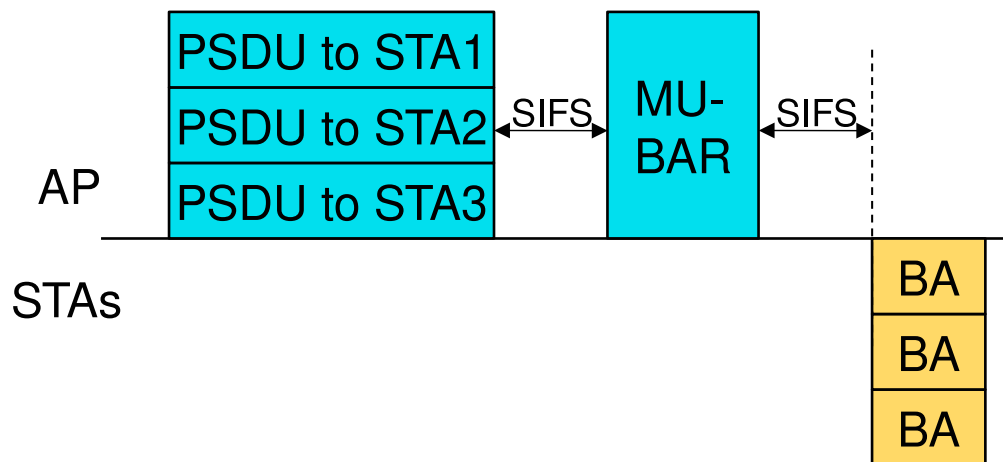
Fig. 10: Acknowledgment of DL MU frames via MU-BAR Trigger Frame sent as single-user frame
