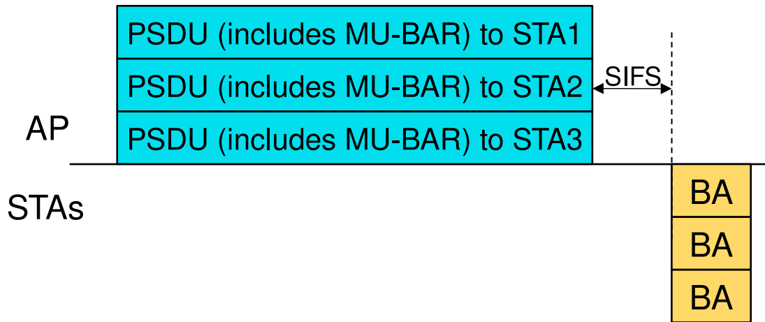
Fig. 11: Acknowledgment of DL MU frames via aggregated MU-BAR Trigger Frames
