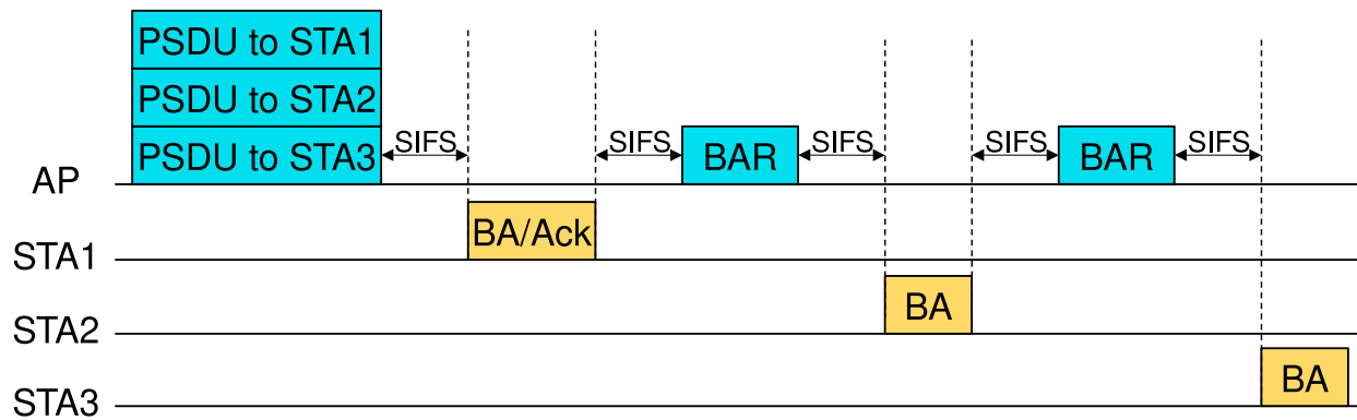
Fig. 9: Acknowledgment of DL MU frames in single-user format
