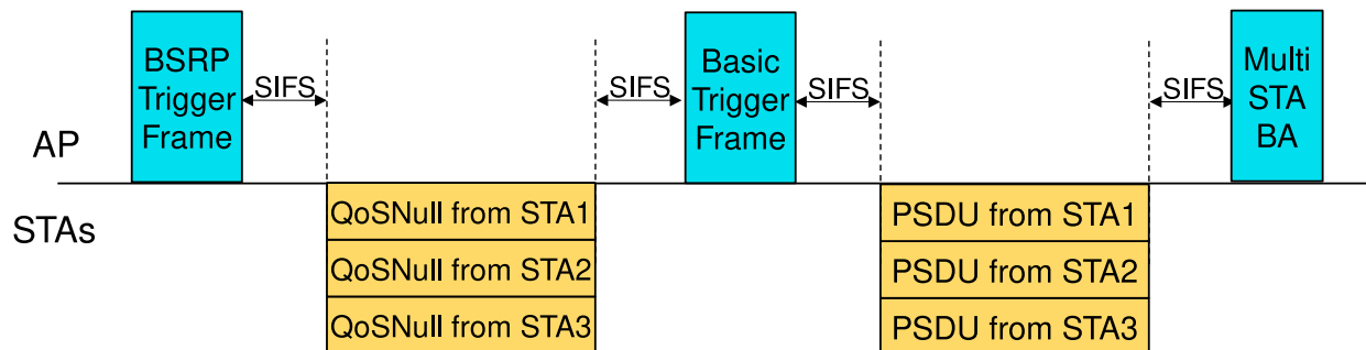
Fig. 12: Frame exchange sequences using UL OFDMA
