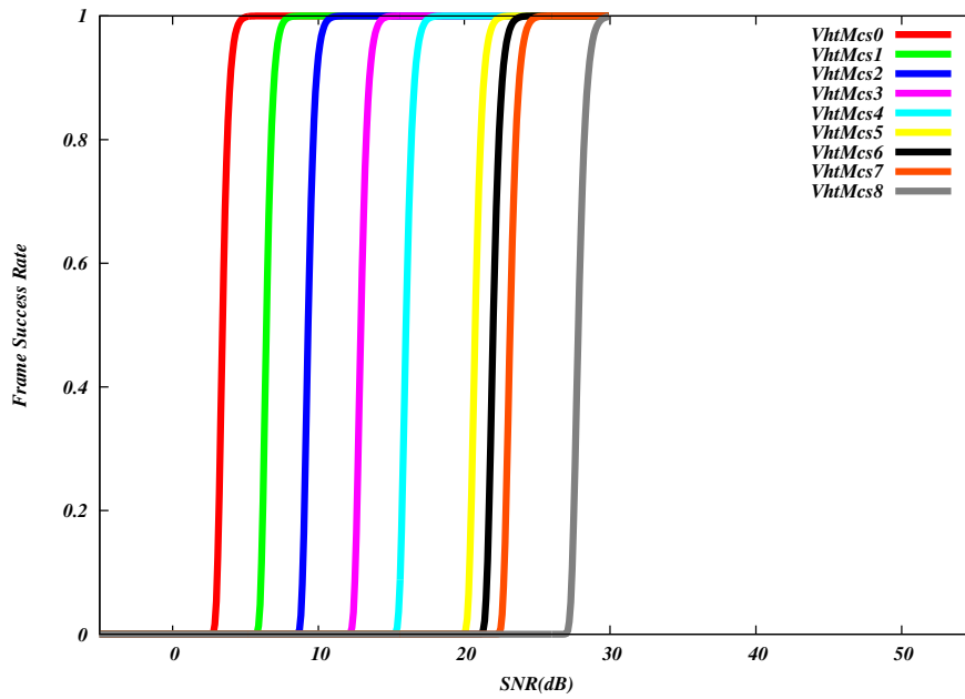
Fig. 16: Frame error rate (NIST model) for 802.11ac (VHT OFDM) Wi-Fi
