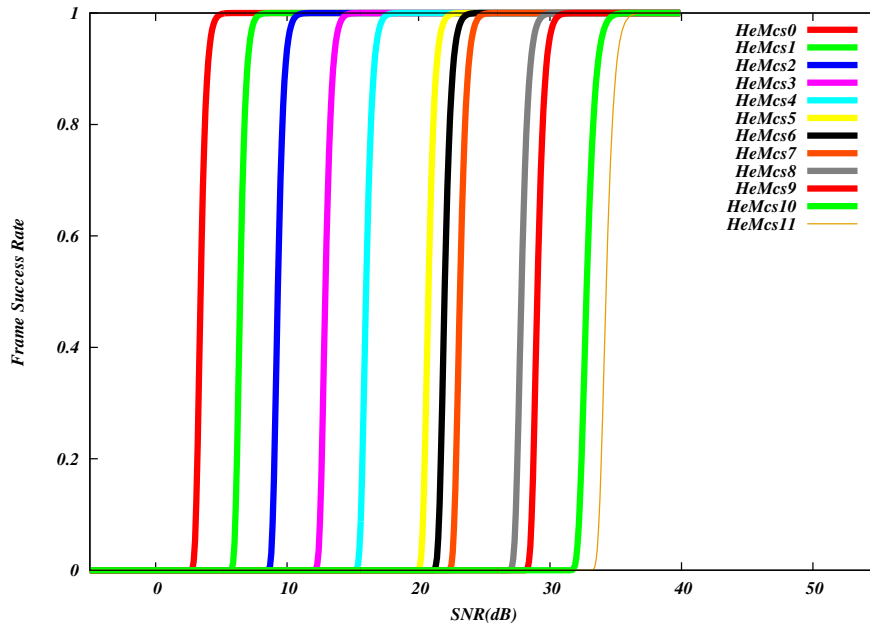
Fig. 17: Frame error rate (NIST model) for 802.11ax (HE OFDM) Wi-Fi
