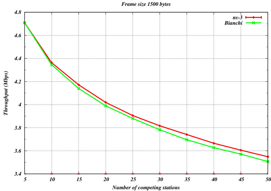
Fig. 19: Bianchi throughput validation results for 802.11g 6 Mbps in infrastructure configuration
