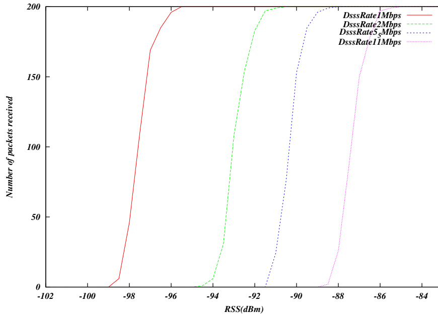
Fig. 13: Clear channel (AWGN) error model for 802.11b
