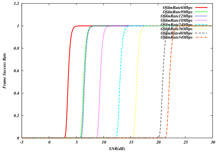
Fig. 14: Frame error rate (NIST model) for 802.11a/g (OFDM) Wi-Fi
