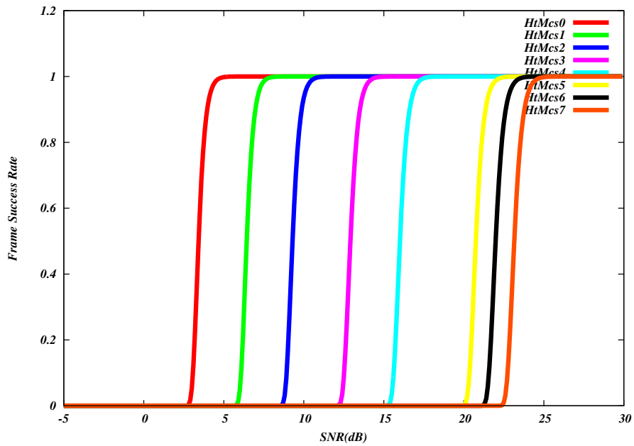
Fig. 15: Frame error rate (NIST model) for 802.11n (HT OFDM) Wi-Fi
