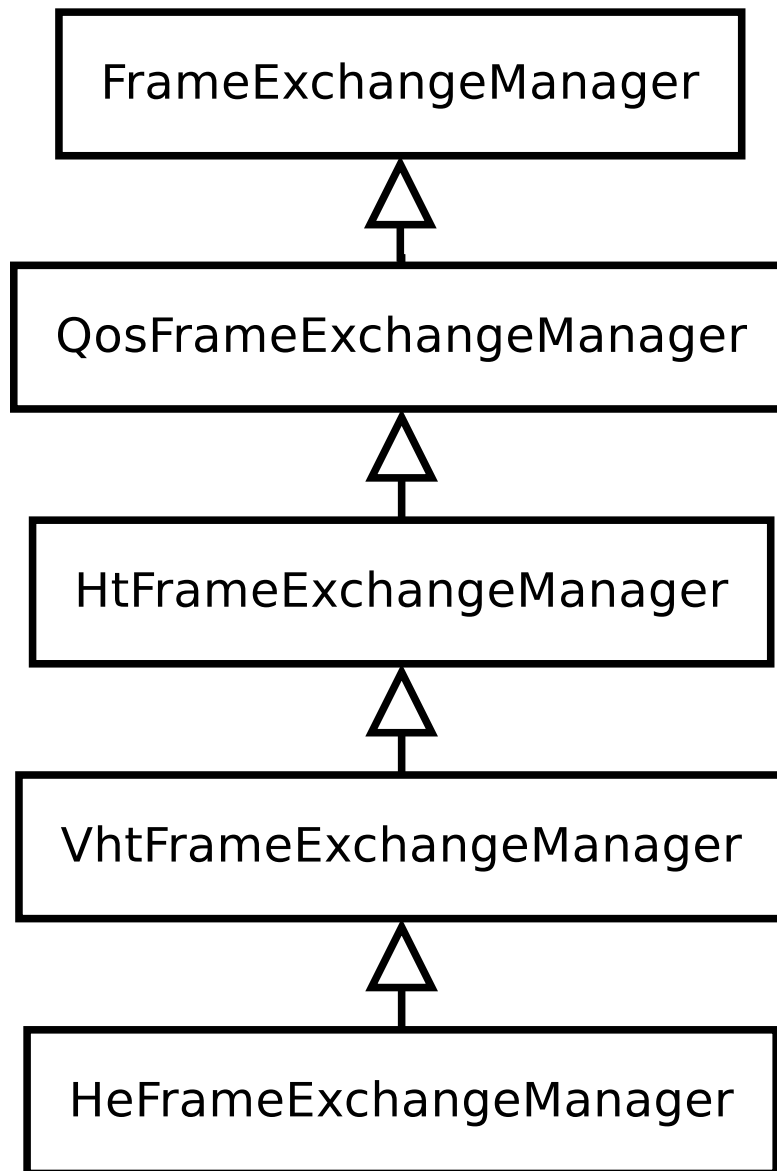
Fig. 8: FrameExchangeManager hierarchy
