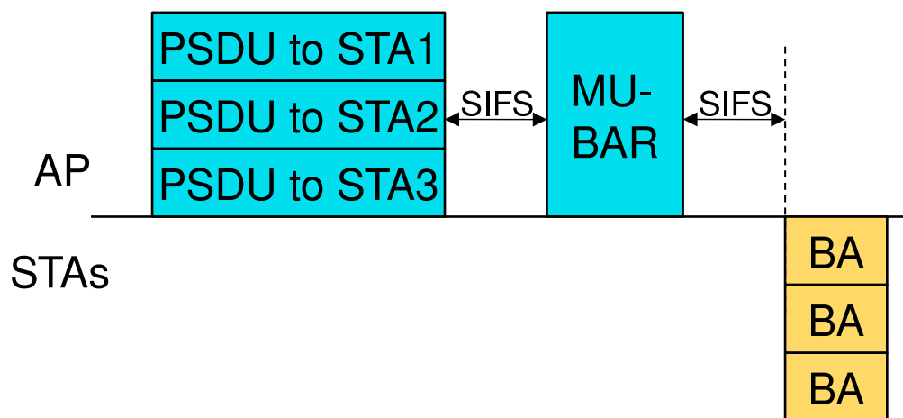
Fig. 10: Acknowledgment of DL MU frames via MU-BAR Trigger Frame sent as single-user frame
