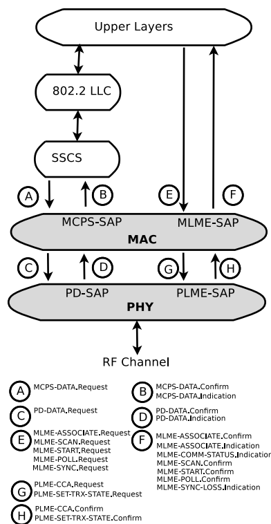
Fig. 1: Architecture and scope of Ir-wpan models
