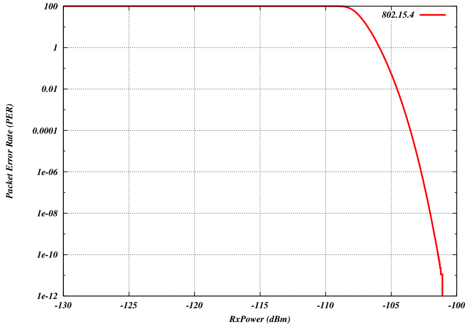
Fig. 4: Packet error rate vs. signal power
