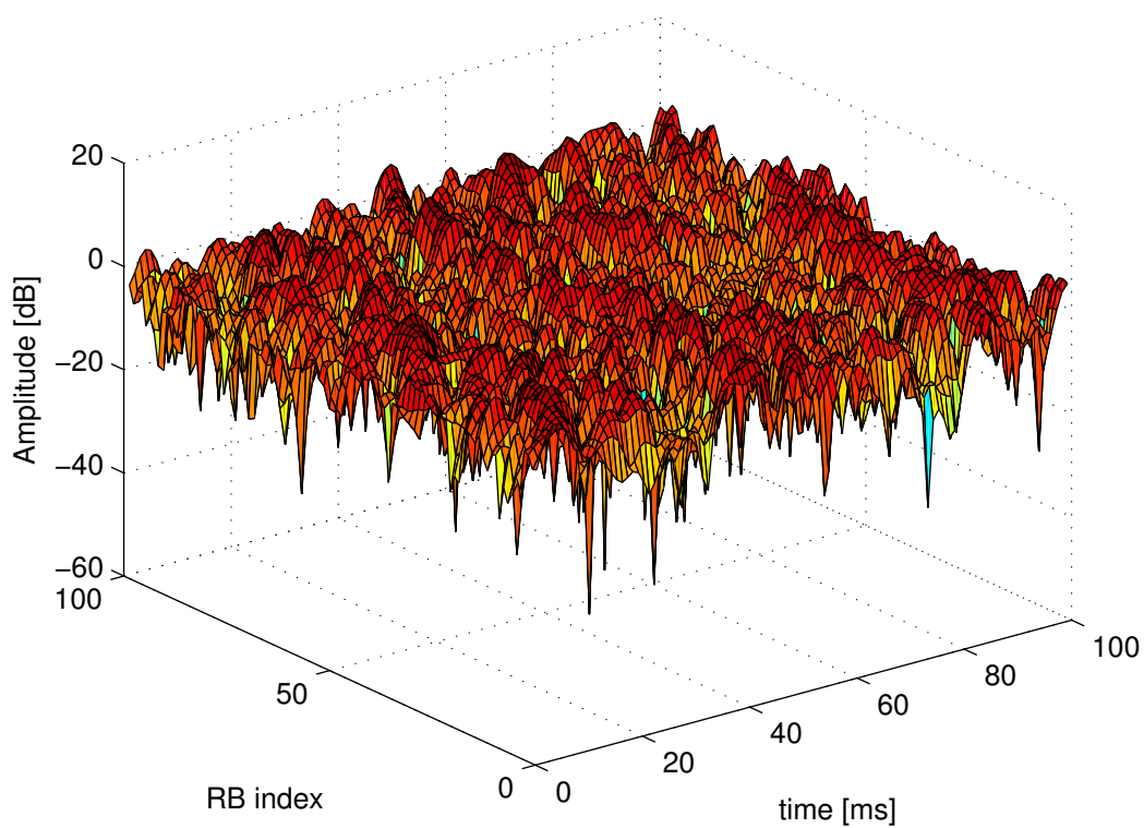
Fig. 72: Excerpt of the fading trace included in the simulator for a vehicular scenario (speed of 60 kmph).
