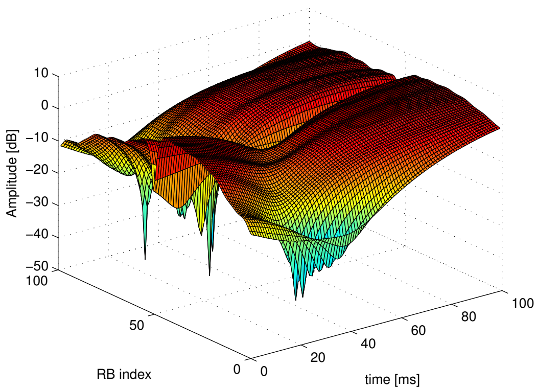
Fig. 71: Excerpt of the fading trace included in the simulator for a pedestrian scenario (speed of 3 kmph).
