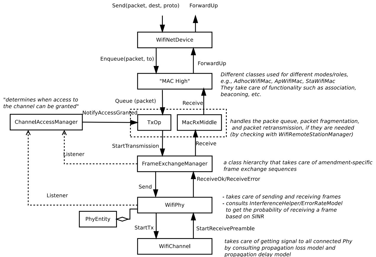
Fig. 1: WifiNetDevice architecture
