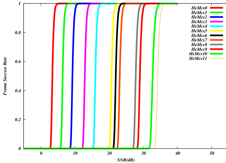
Fig. 16: Frame error rate (NIST model) for 802.11ax (HE OFDM) Wi-Fi
