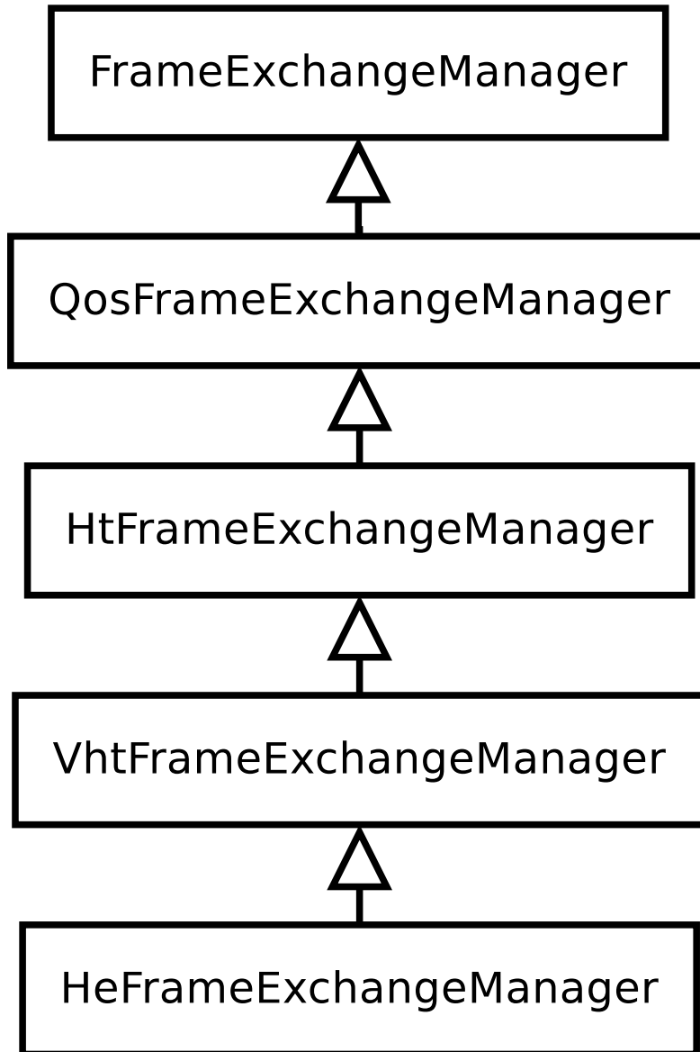
Fig. 7: FrameExchangeManager hierarchy
