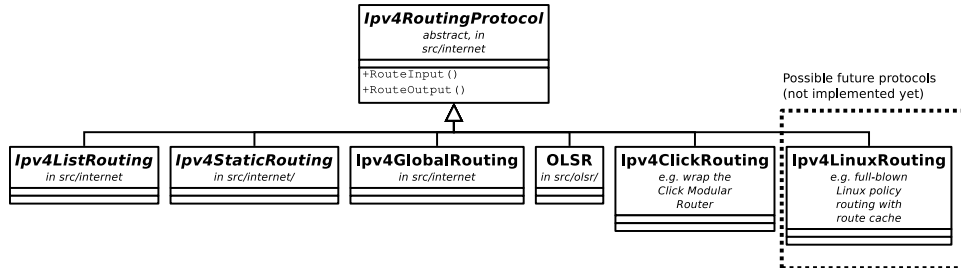
Fig. 4: Ipv4Routing specialization.
