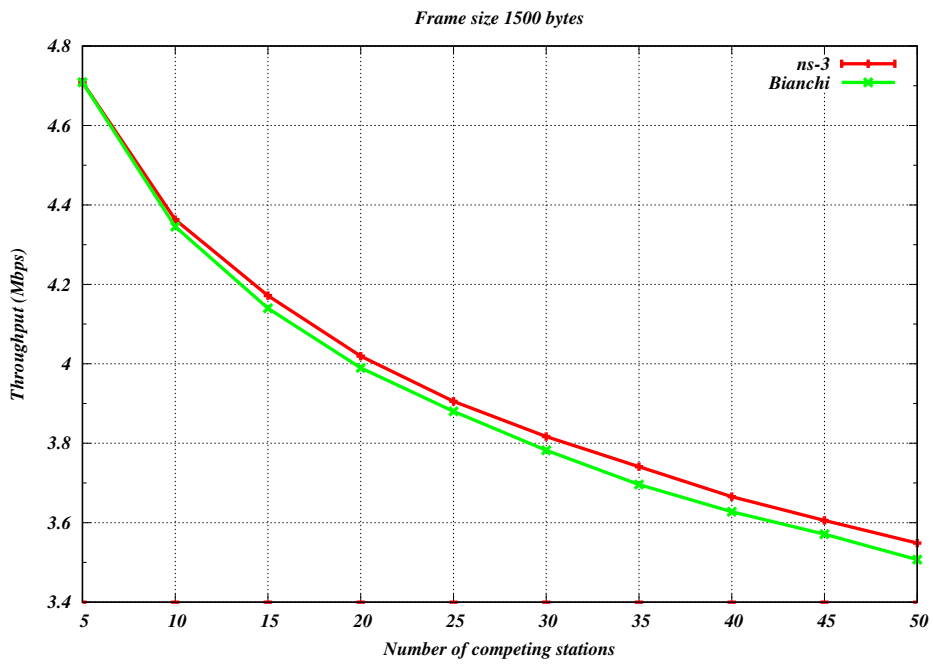
Fig. 9: Bianchi throughput validation results for 802.11g 6 Mbps in infrastructure configuration
