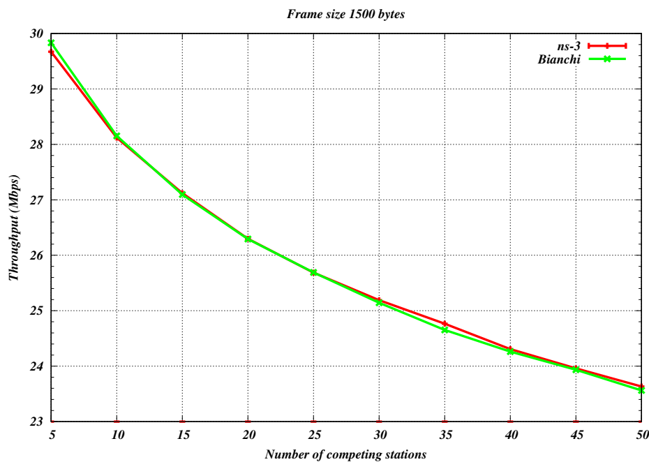
Fig. 8: Bianchi throughput validation results for 802.11a 54 Mbps in adhoc configuration
