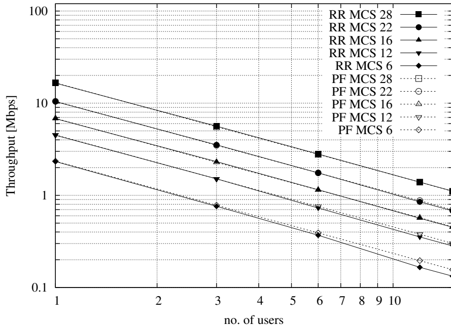
Figure 19.85: Test vectors for the RR and PF Scheduler in the downlink in a scenario where all UEs use the same MCS.
