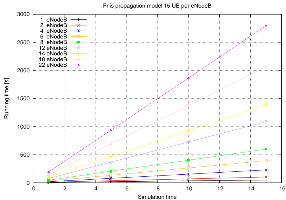
Figure 19.96: Simulation time
