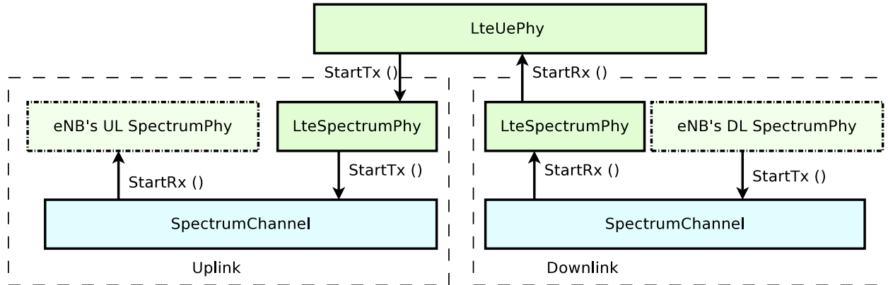
Figure 19.4: PHY and channel model architecture for the UE
