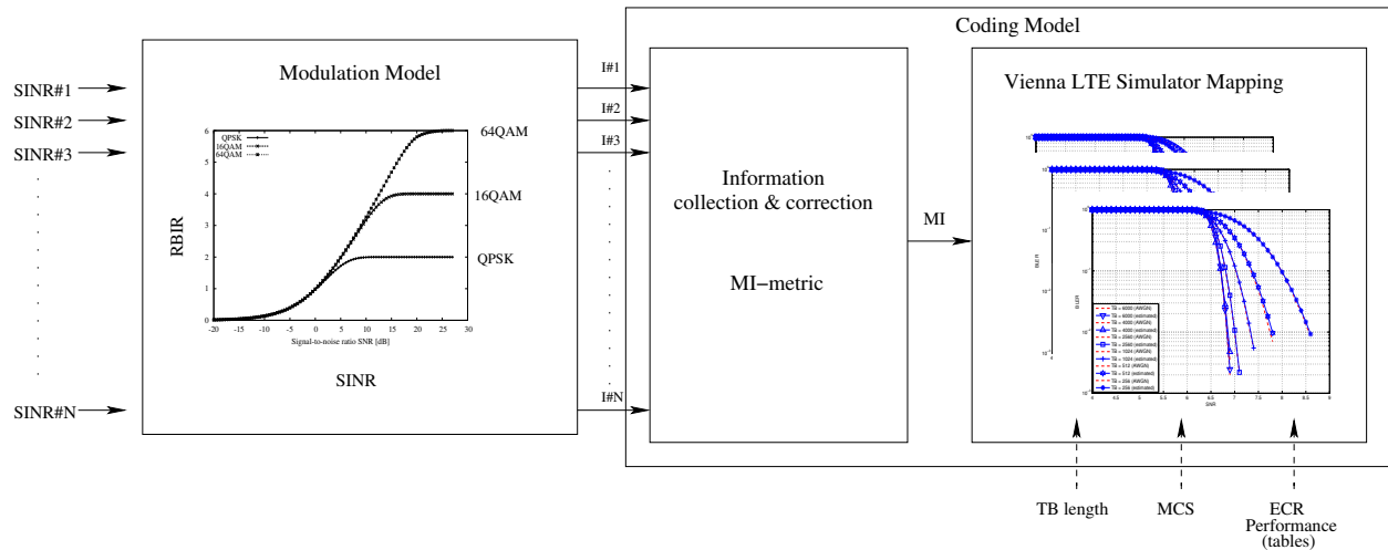
Figure 19.12: MIESM computational procedure diagram
