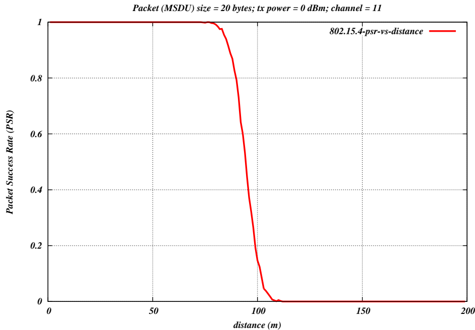
Figure 18.5: Default output of the program lr-wpan-error-distance-plot.cc
