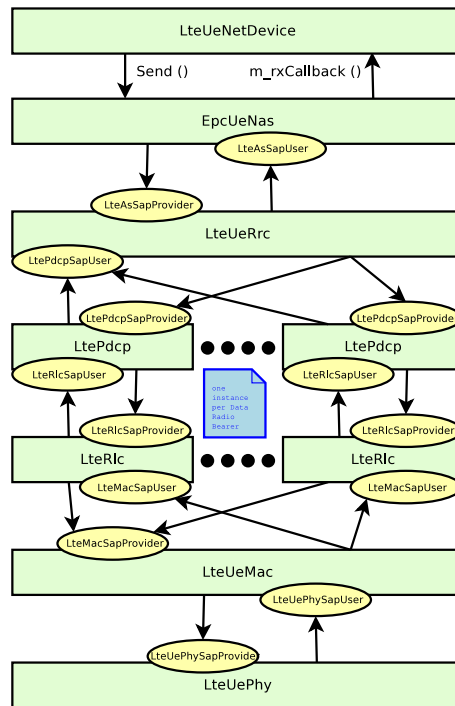
Figure 19.2: LTE radio protocol stack architecture for the UE on the data plane
