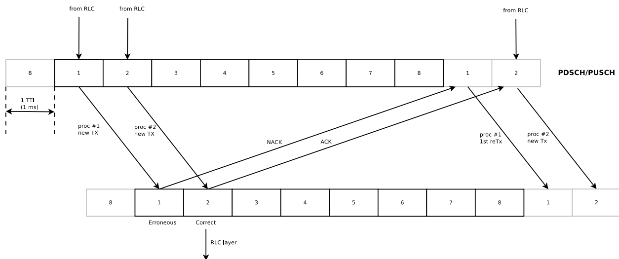
Figure 19.21: HARQ processes behavior in LTE
