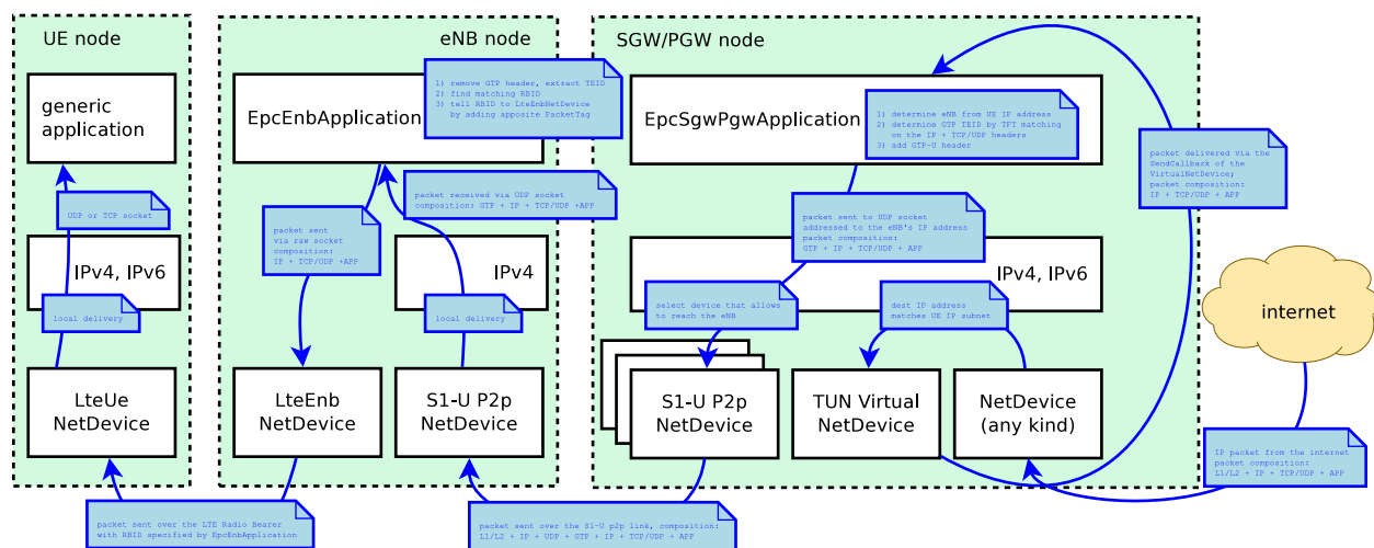
Figure 19.40: Data flow in the downlink between the internet and the UE
