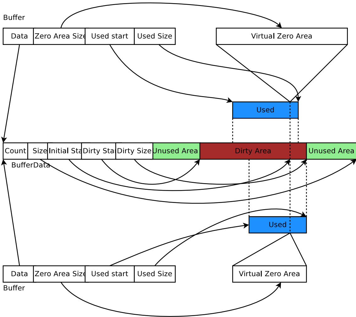
Figure 23.2: Implementation overview of a packet's byte Buffer.
