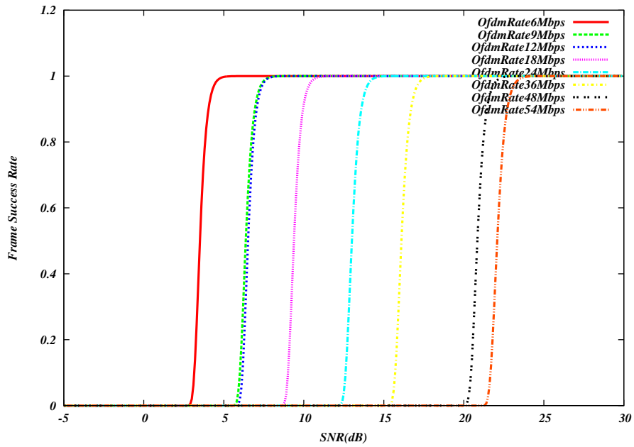
Figure 36.4: Frame error rate (NIST model) for 802.11a/g (OFDM) Wi-Fi
