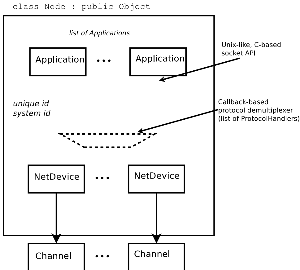
Figure 23.3: High-level node architecture
