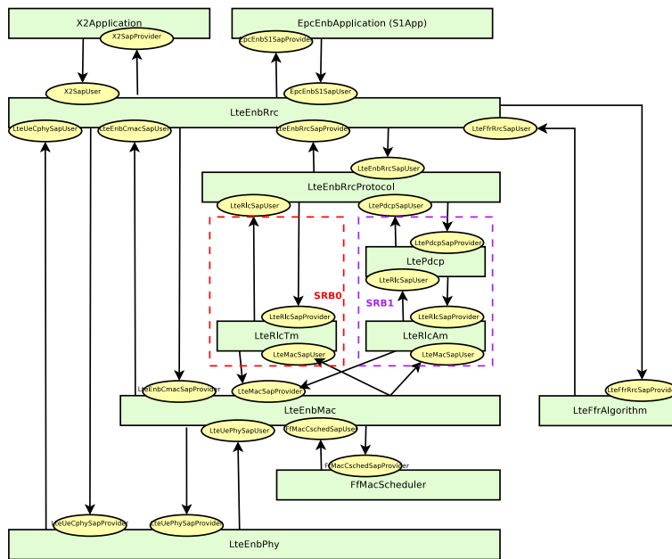
Figure 19.6: LTE radio protocol stack architecture for the eNB on the control plane
