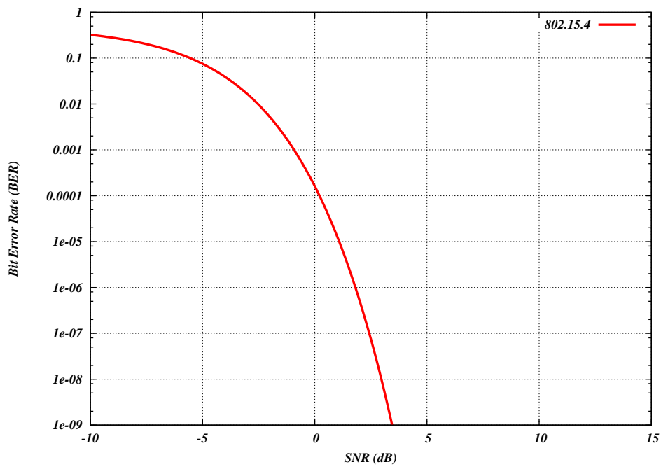
Figure 18.6: Default output of the program lr-wpan-error-model-plot.cc
