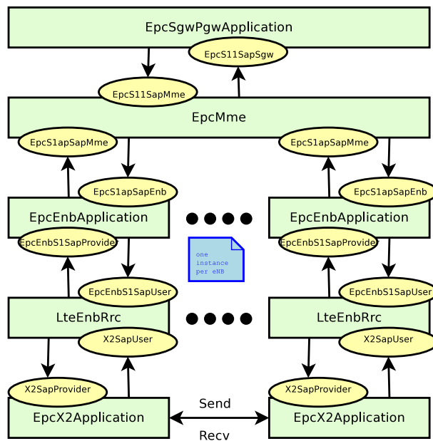
Figure 19.9: EPC control model
