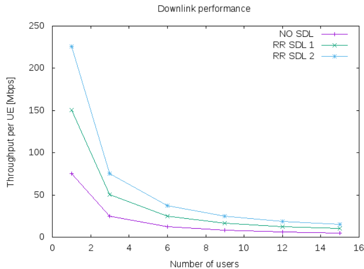
Figure 19.79: Example of CA test performance in the downlink
