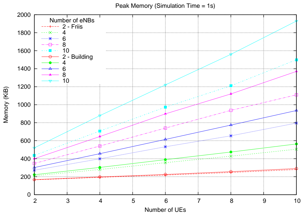
Figure 19.97: Memory profile
