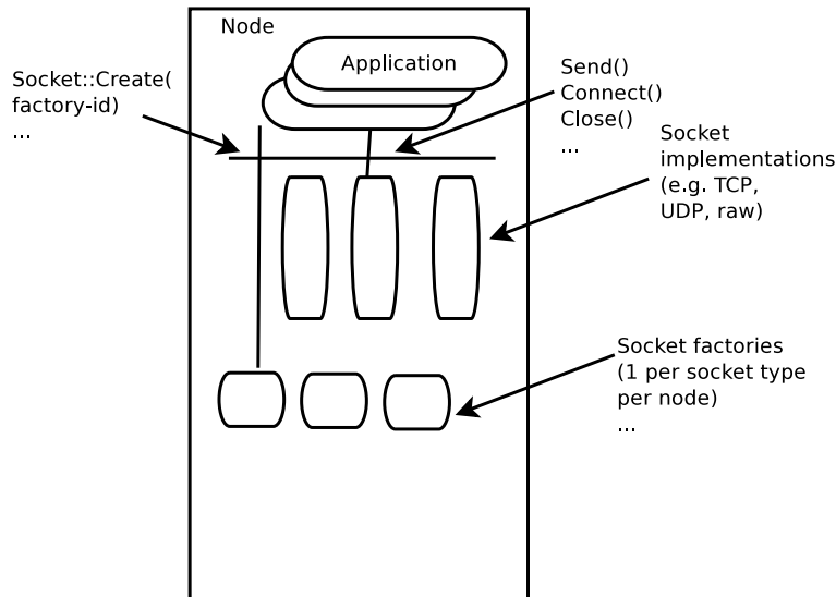
Figure 23.4: Implementation overview of native sockets API
