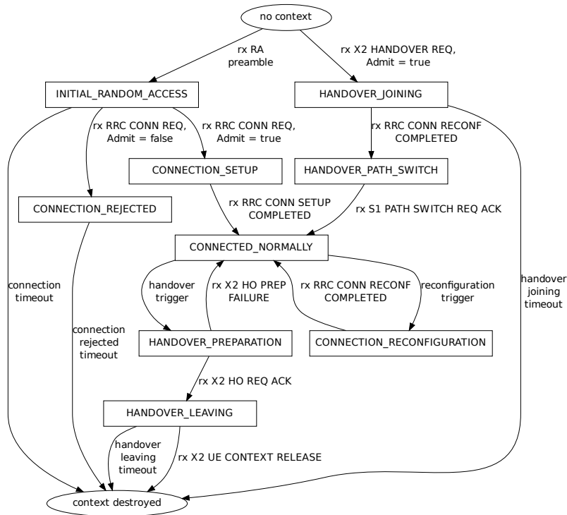
Figure 19.31: ENB RRC State Machine for each UE
