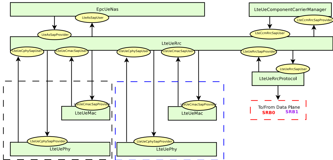
Figure 19.66: UE Control Plane Architecture
