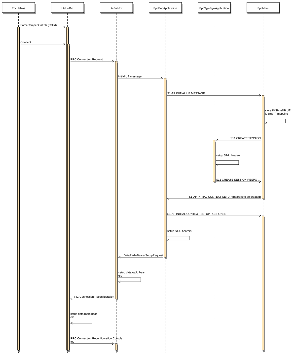
Figure 19.39: Sequence diagram of the attach procedure
