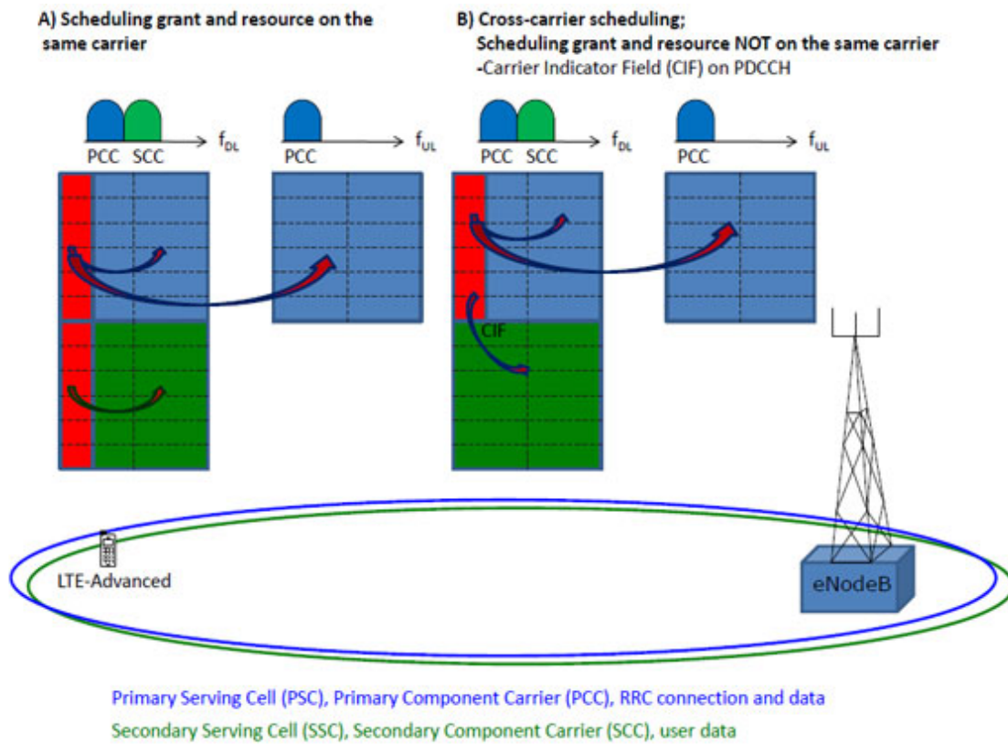
Figure 19.57: CA scheduling schemes (from 3gpp.org)
