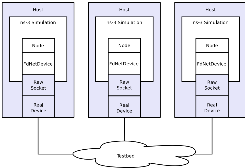
Figure 13.1: Example Implementation of Testbed Emulation.
