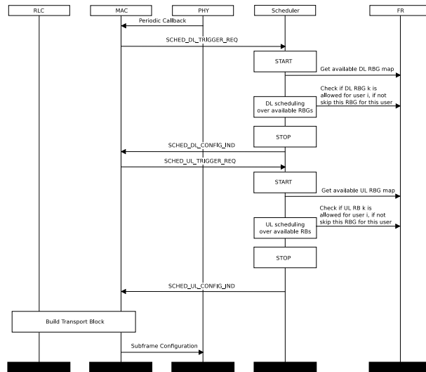
Figure 19.46: Sequence diagram of Scheduling with FR algorithm
