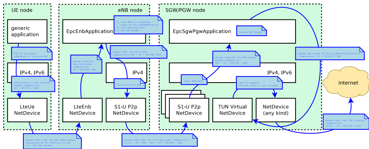
Figure 19.41: Data flow in the uplink between the UE and the internet
