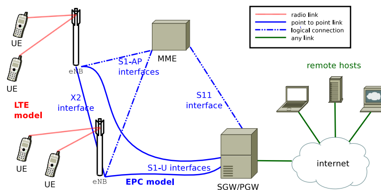
Figure 19.1: Overview of the LTE-EPC simulation model
