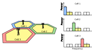
Figure 19.53: Enhanced Fractional Fractional Frequency Reuse scheme
