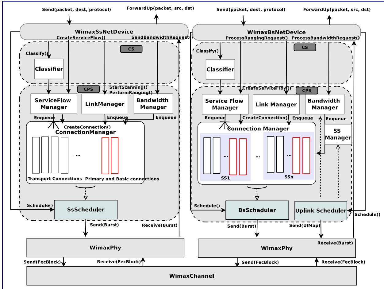
Figure 37.1: WiMAX architecture
