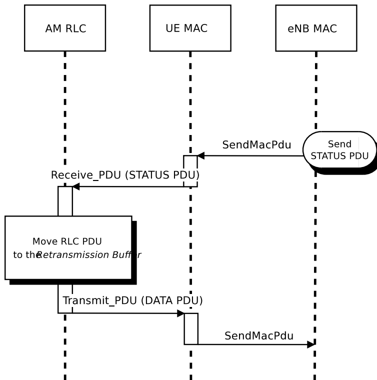
Figure 19.29: Sequence diagram of data PDU retransmission in uplink
