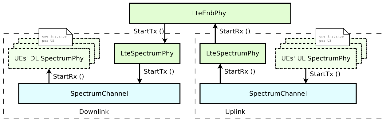
Figure 19.7: PHY and channel model architecture for the eNB
