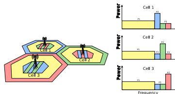
Figure 19.52: Soft Fractional Fractional Frequency Reuse scheme
