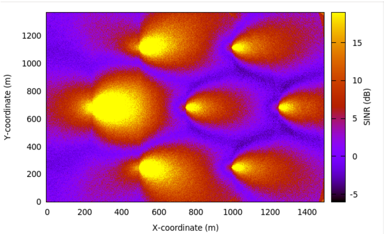
Figure 19.75: REM for RB 1 obtained from lena-dual-stripe simulation with Hard FR algorithm enabled
