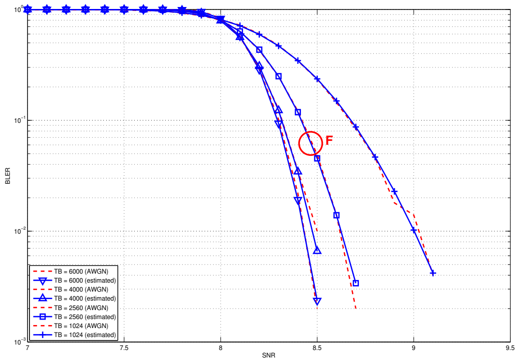
Figure 19.89: BLER for test 6.
