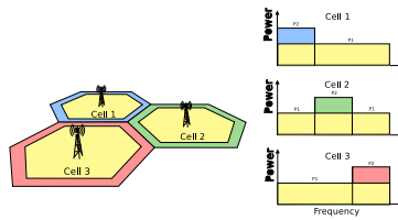
Figure 19.50: Soft Frequency Reuse scheme version 1
