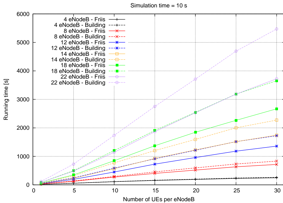
Figure 19.95: Propagation Model
