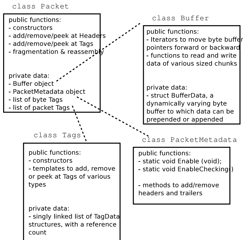
Figure 23.1: Implementation overview of Packet class.
