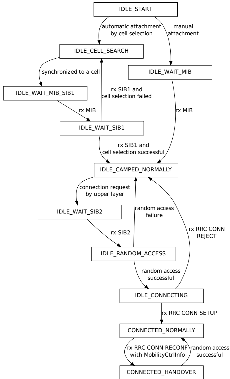
Figure 19.30: UE RRC State Machine
