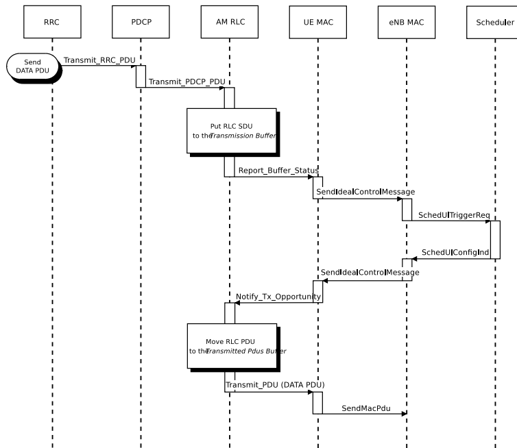
Figure 19.28: Sequence diagram of data PDU transmission in uplink
