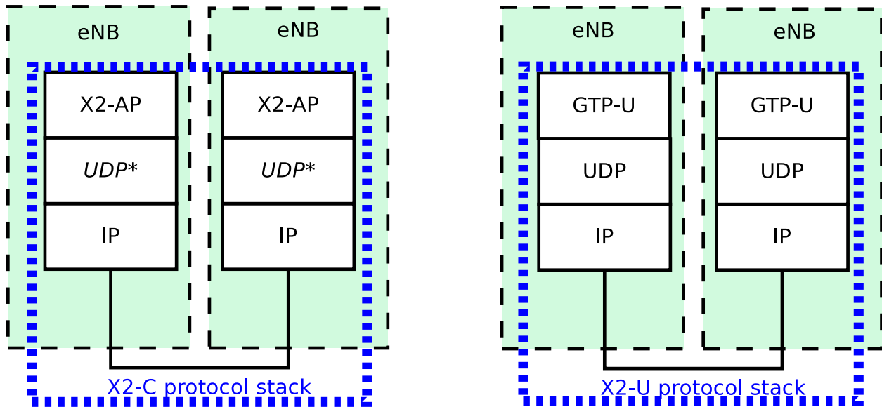
Figure 19.44: X2 interface protocol stacks
