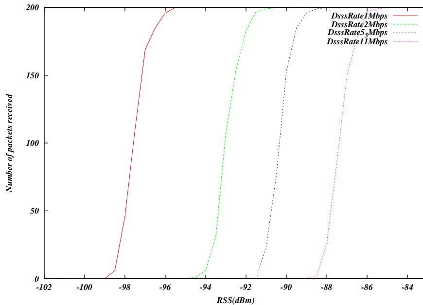
Figure 36.3: Clear channel (AWGN) error model for 802.11b
