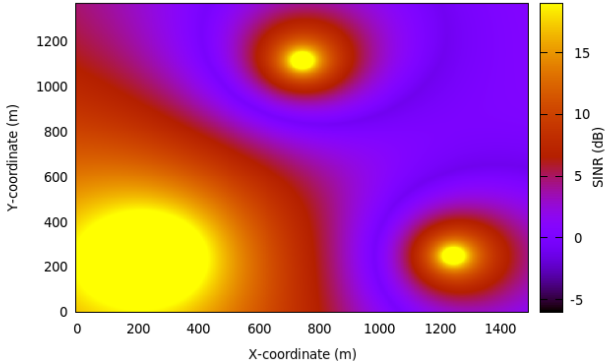
Figure 19.73: REM for RB 1 obtained from lena-frequency-reuse example with Soft FR algorithm enabled
