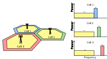
Figure 19.49: Strict Frequency Reuse scheme
