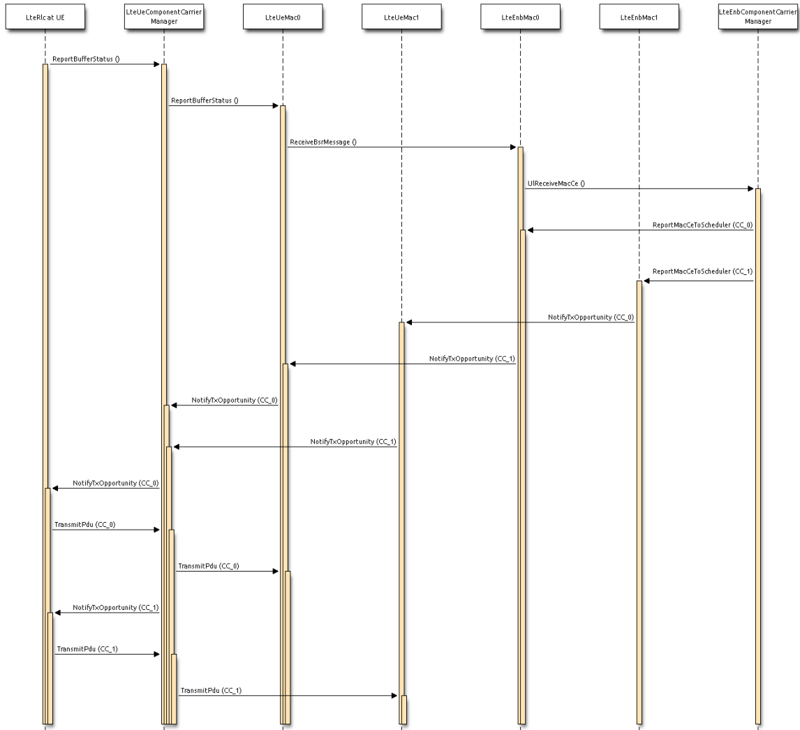
Figure 19.65: Uplink buffer status reporting with CA
