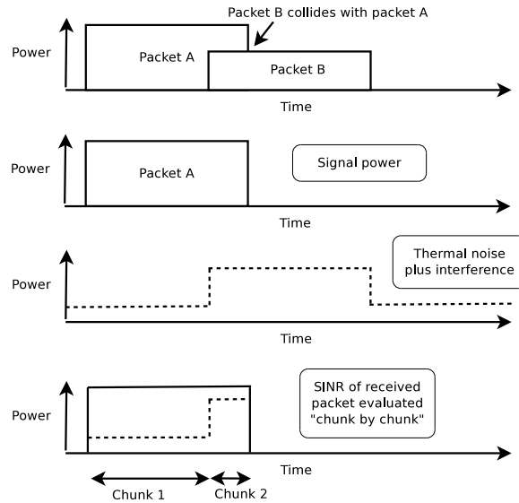
Figure 36.2: SNIR function over time.
