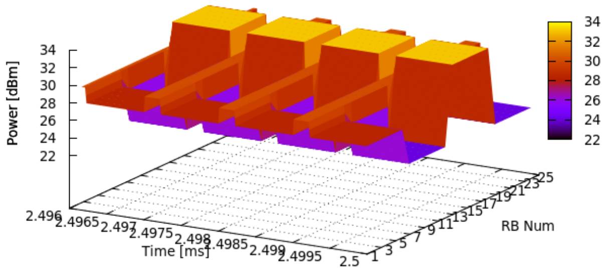
Figure 19.74: Spectrum Analyzer trace obtained from lena-frequency-reuse example with Soft FFR algorithm enabled. Spectrum Analyzer was located near eNB with FrCellTypeId 2 .
