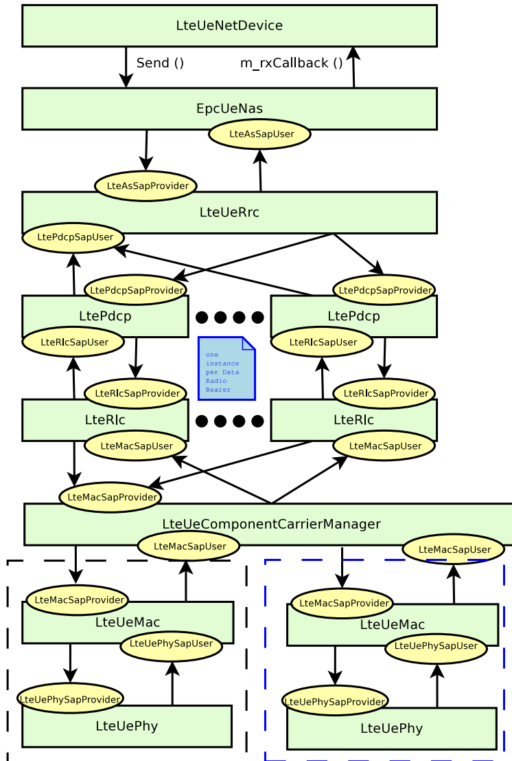
Figure 19.64: UE Data Plane Architecture
