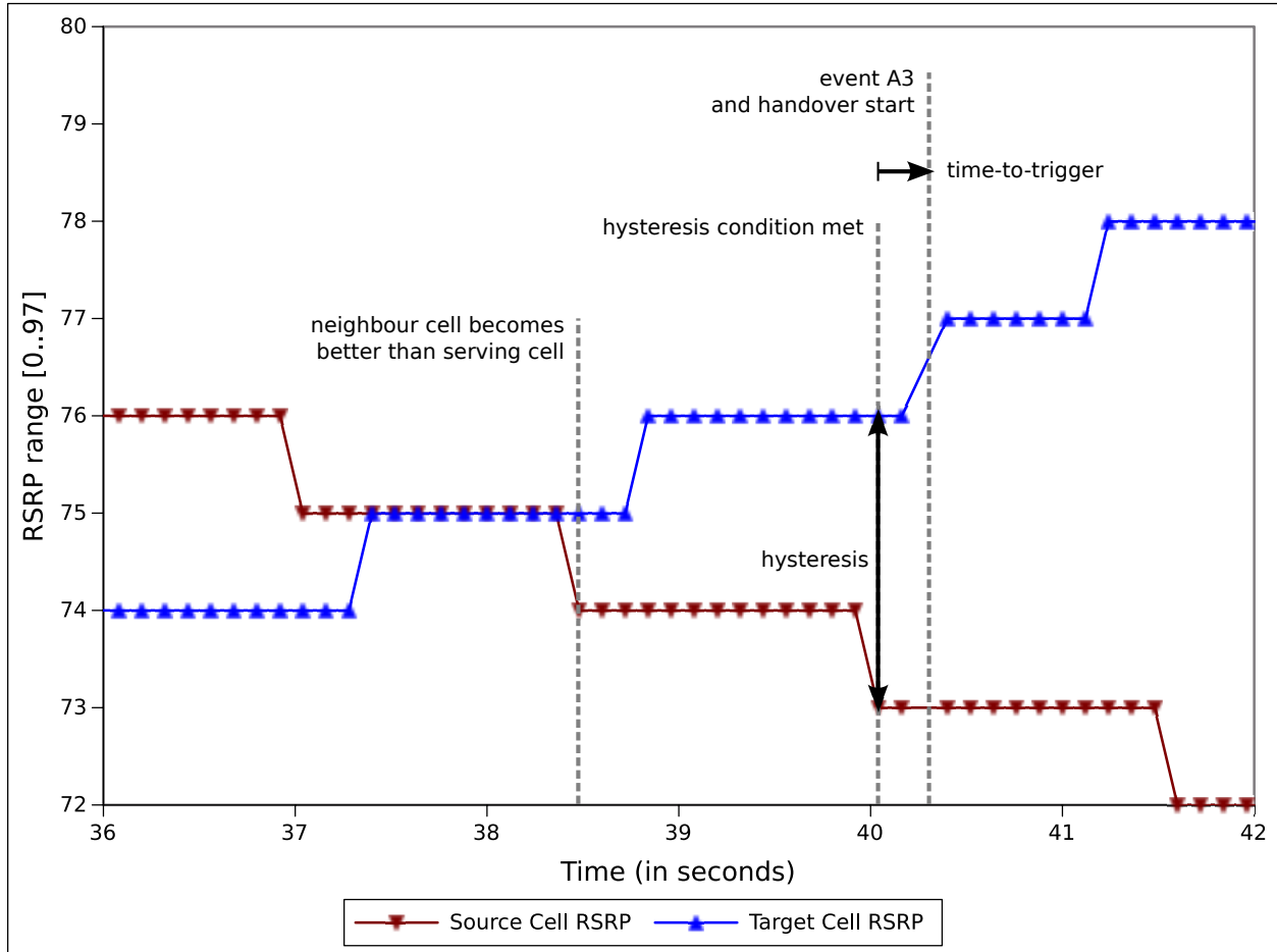
Figure 19.35: Effect of hysteresis and time-to-trigger in strongest cell handover algorithm
