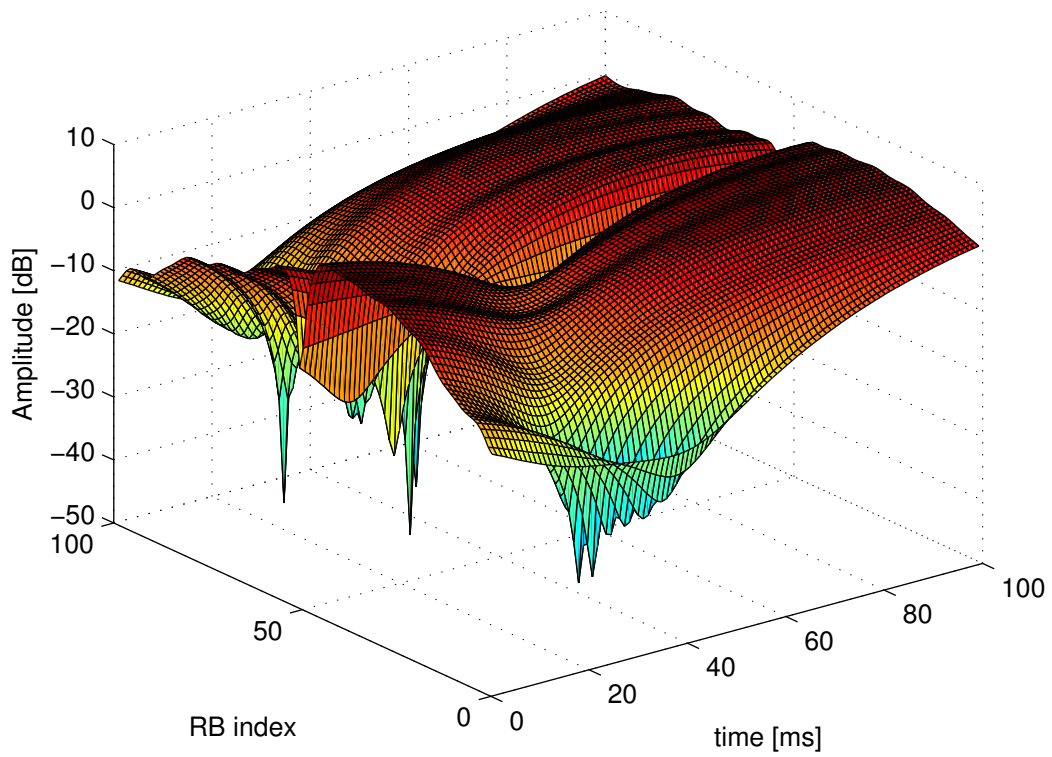
Figure 19.68: Excerpt of the fading trace included in the simulator for a pedestrian scenario (speed of 3 kmph).
