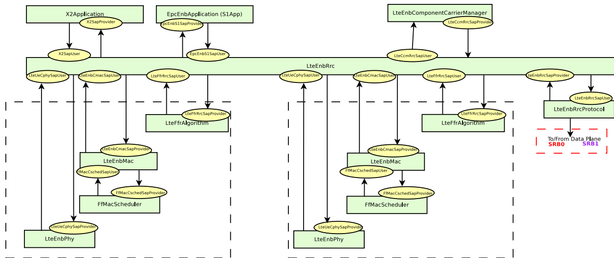
Figure 19.62: eNB Control Plane Architecture
