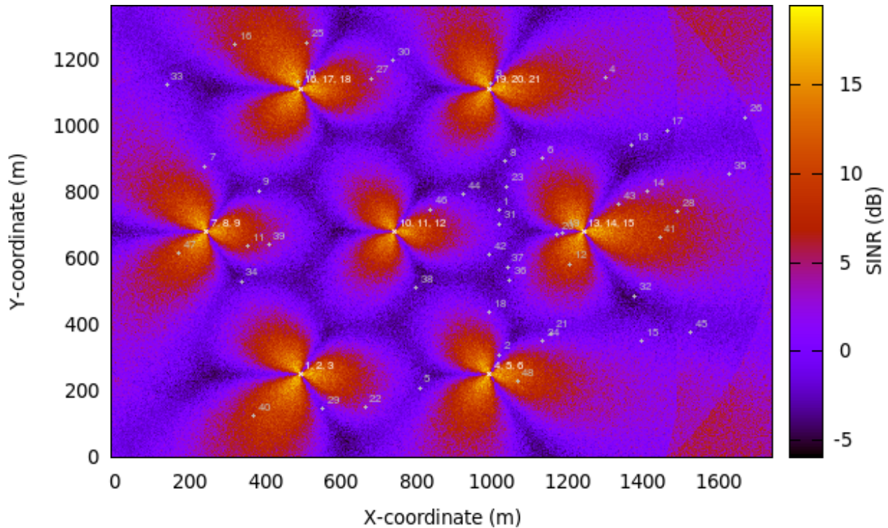
Figure 19.72: REM obtained from a simulation in handover campaign
