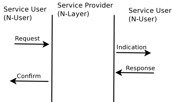
Figure 18.2: Service primitives
