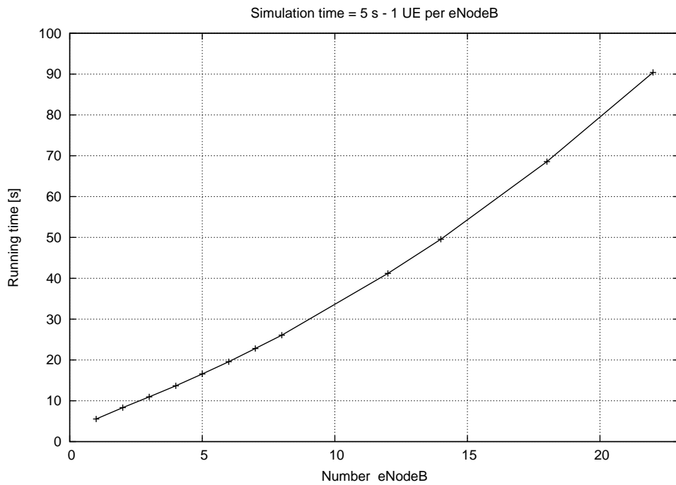
Figure 19.98: Running time
