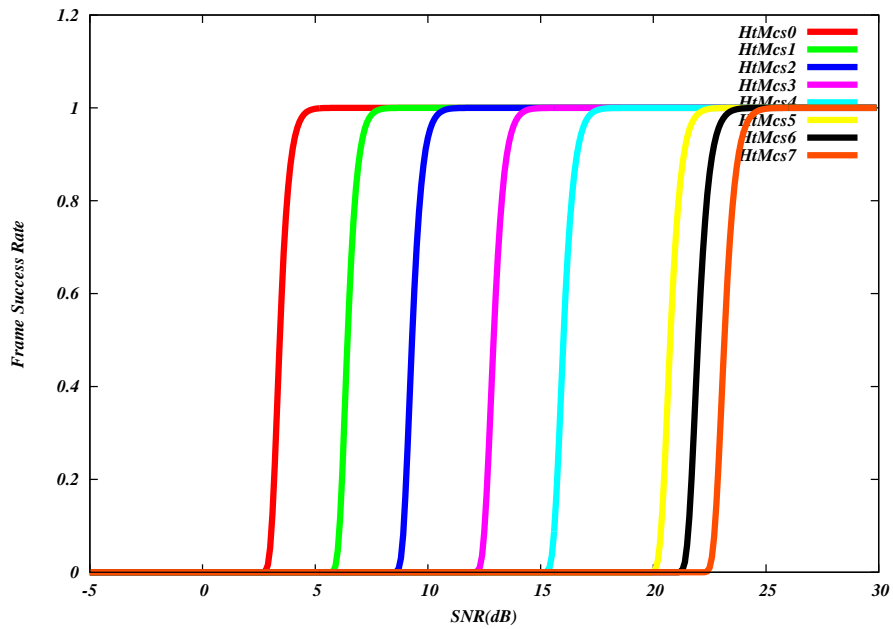
Figure 36.5: Frame error rate (NIST model) for 802.11n (HT OFDM) Wi-Fi
