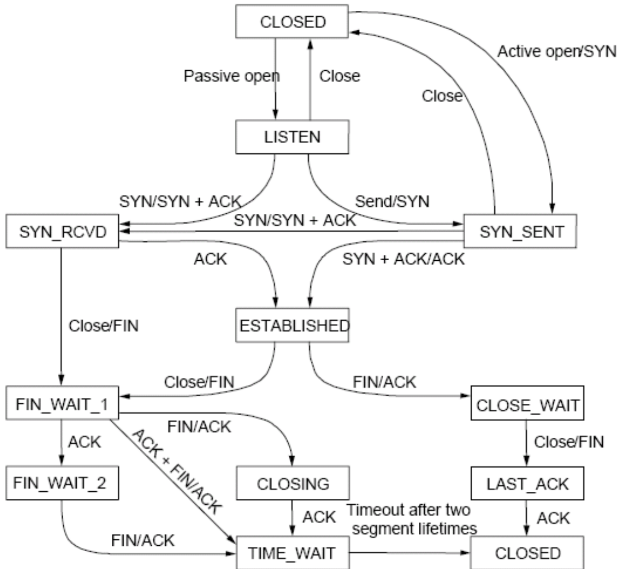
Figure 17.5: TCP State machine
