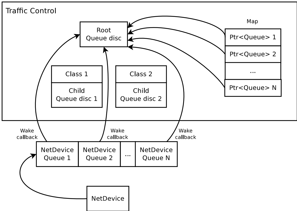
Figure 33.1: Setup of a queue disc (wake mode: WAKE_ROOT)
