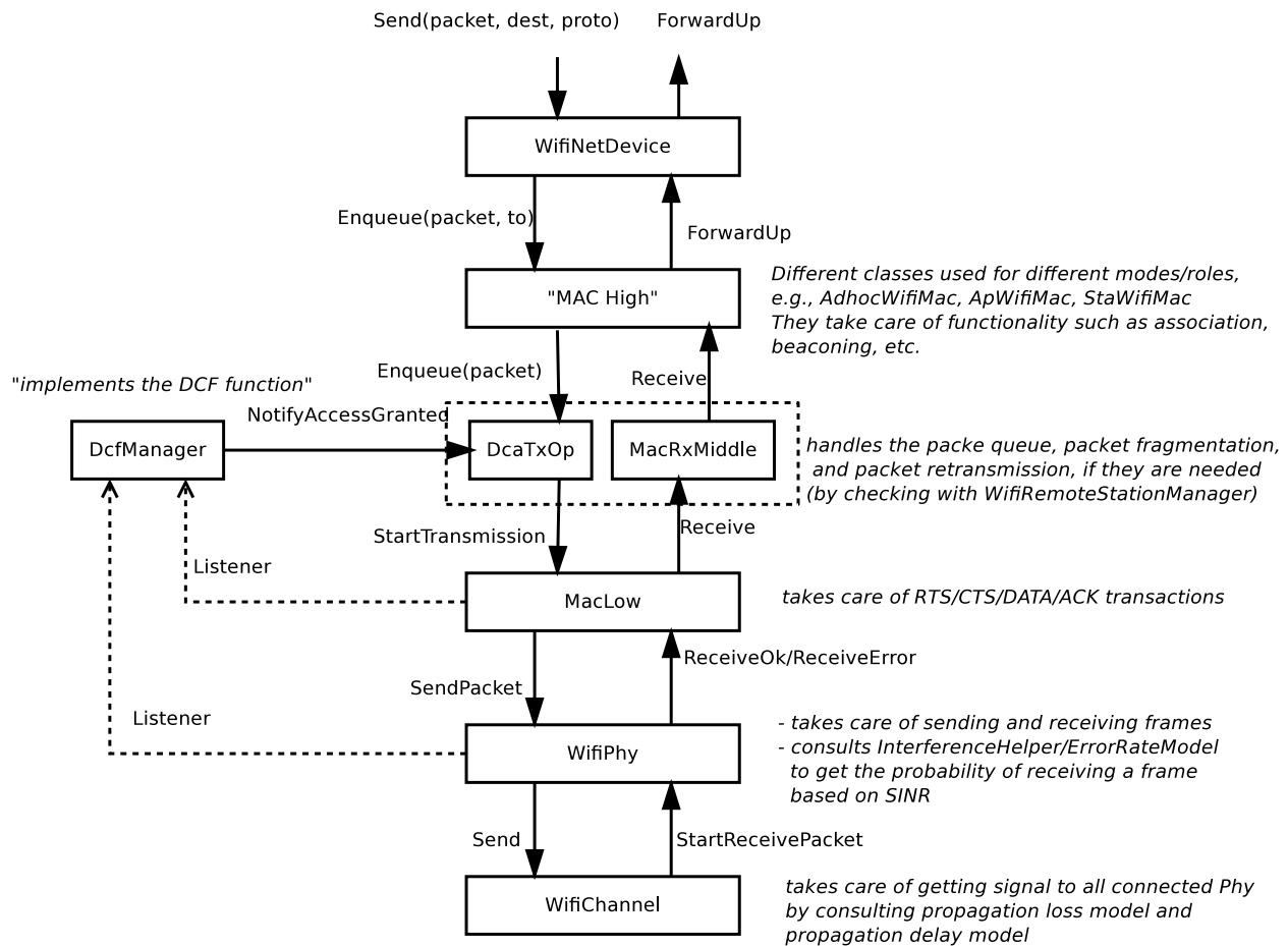
Figure 36.1: WifiNetDevice architecture.
