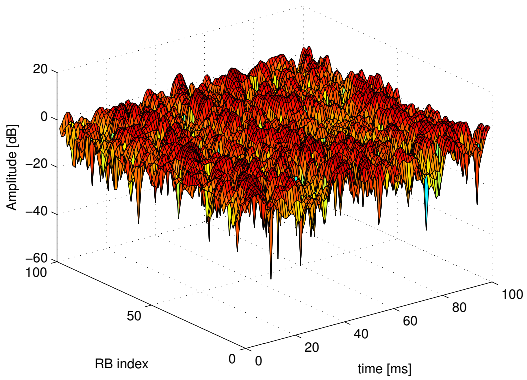
Figure 19.69: Excerpt of the fading trace included in the simulator for a vehicular scenario (speed of 60 kmph).
