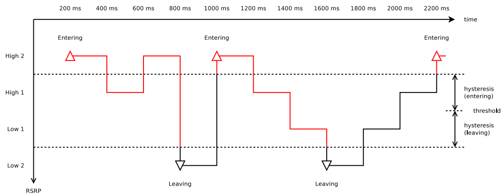
Figure 19.84: Measured RSRP trace of an example Event A1 with hysteresis test case in piecewise configuration
