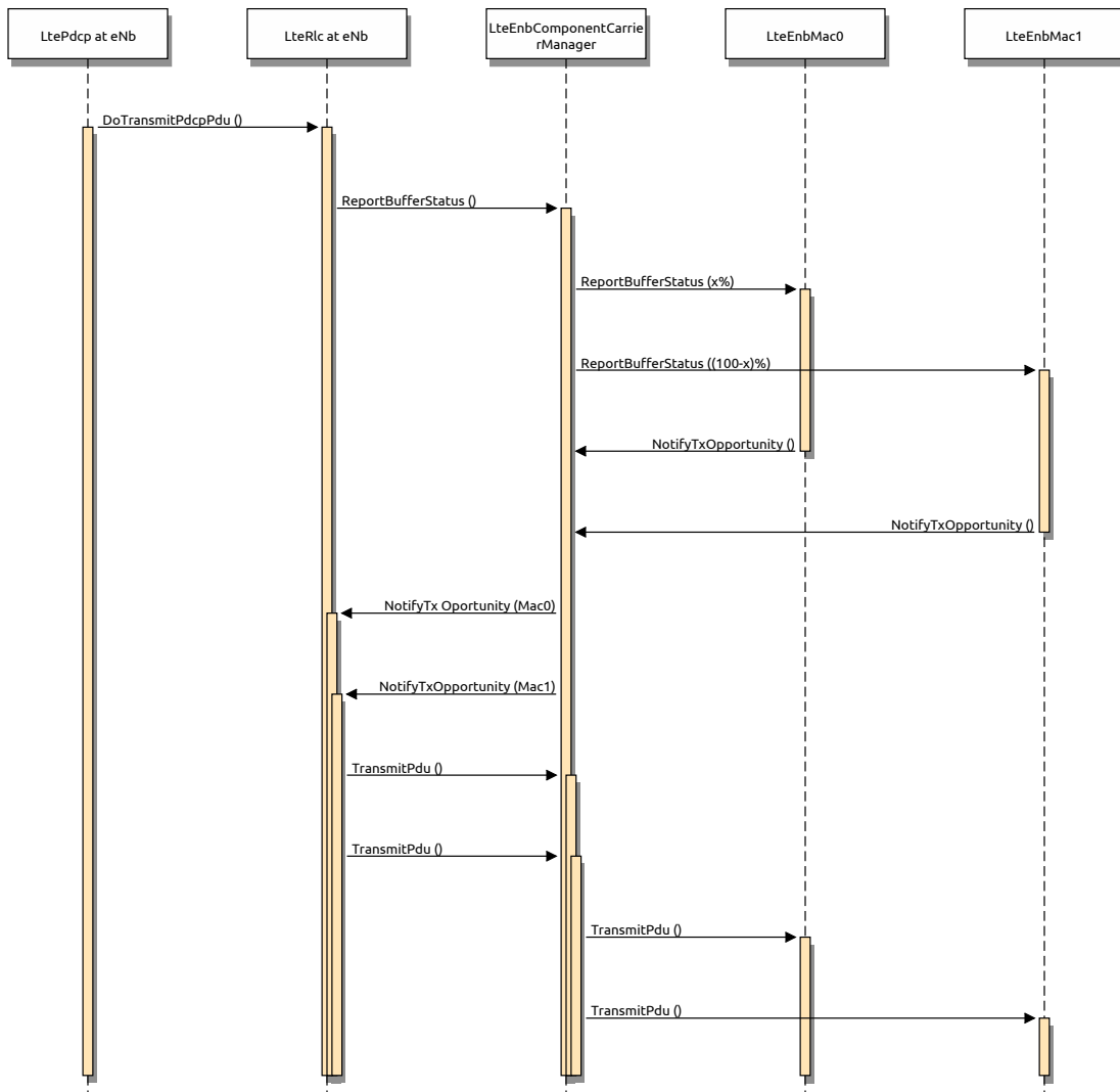
Figure 19.61: Sequence Diagram of downlink buffer status reporting (BSR) with CA
