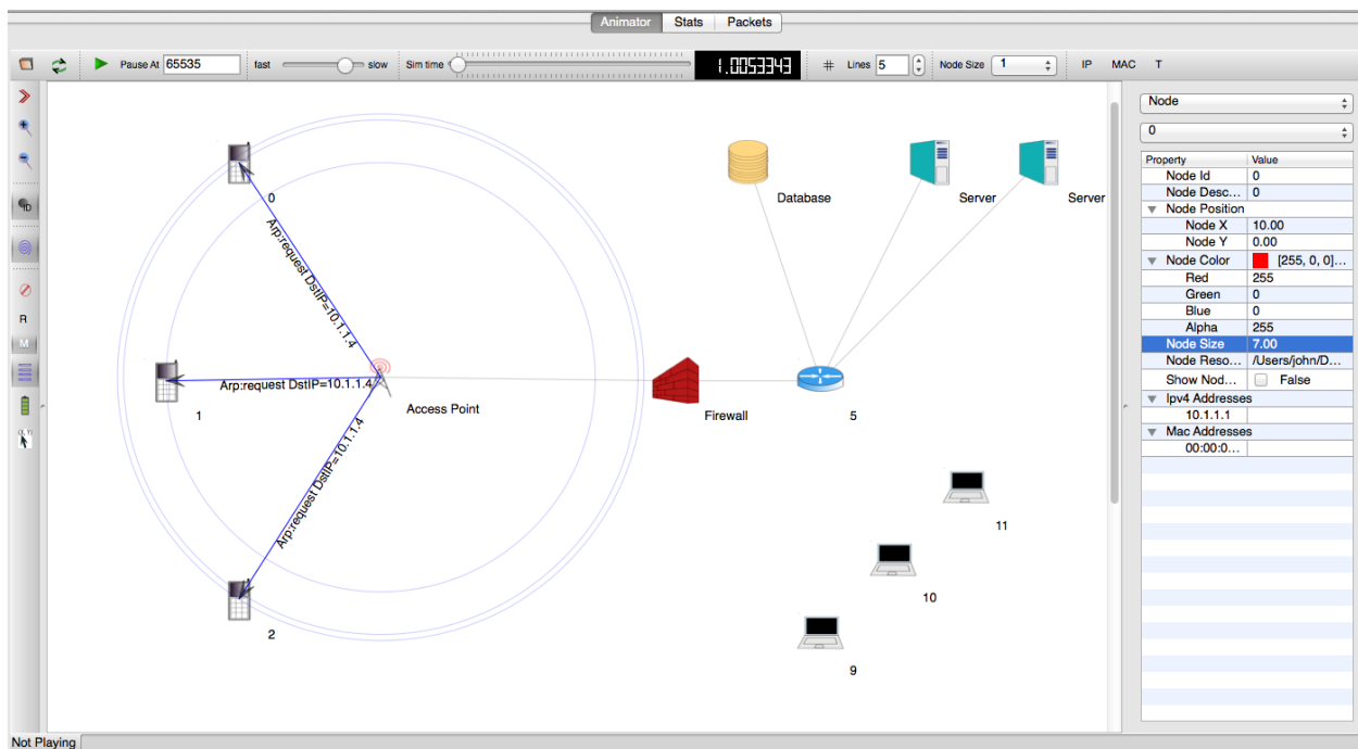
Figure 2.1: An example of packet animation on wired-links
