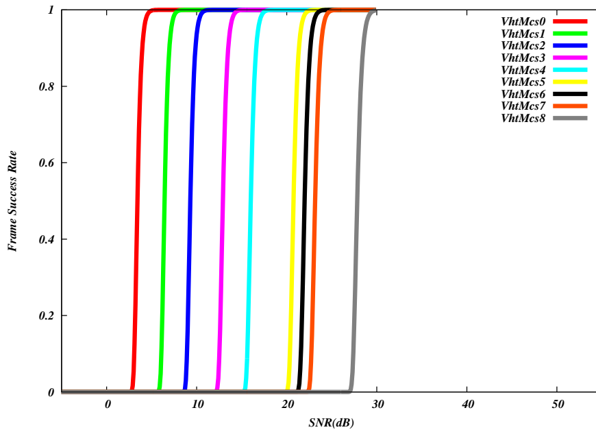
Figure 36.6: Frame error rate (NIST model) for 802.11ac (VHT OFDM) Wi-Fi
