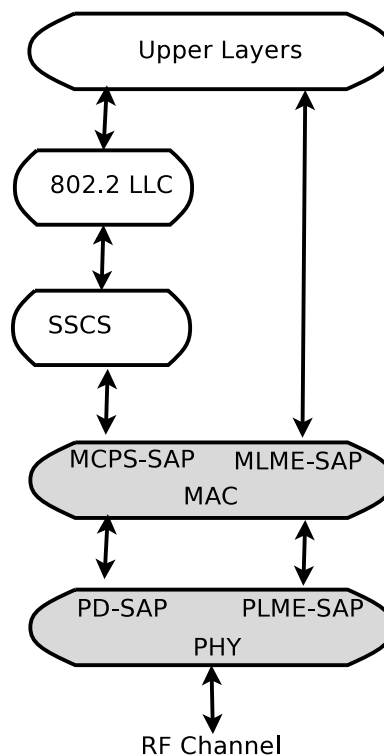
Figure 18.1: Architecture and scope of lr-wpan models
