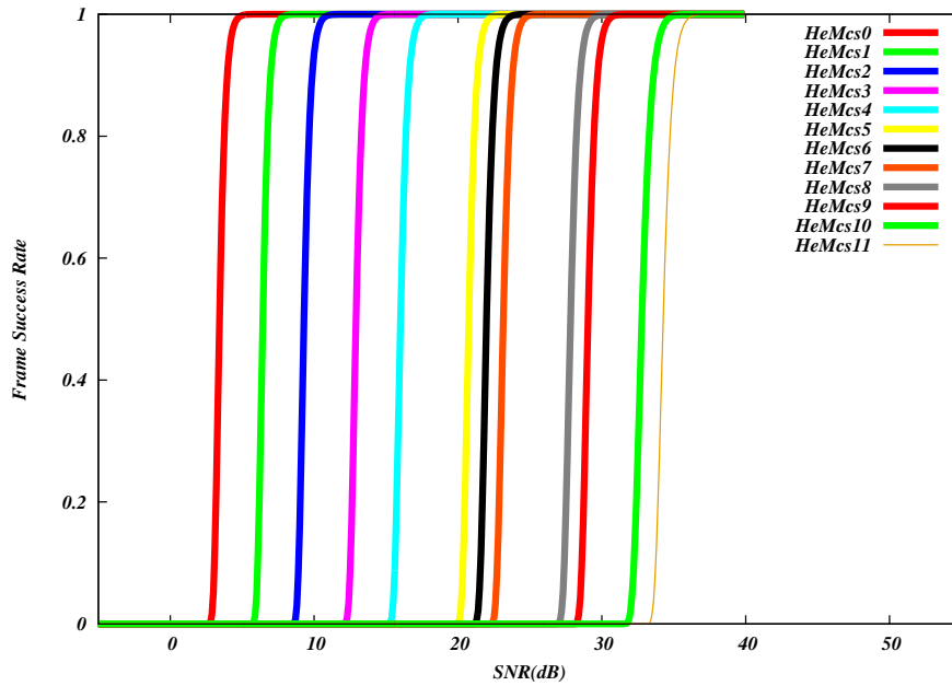
Figure 36.7: Frame error rate (NIST model) for 802.11ax (HE OFDM) Wi-Fi
