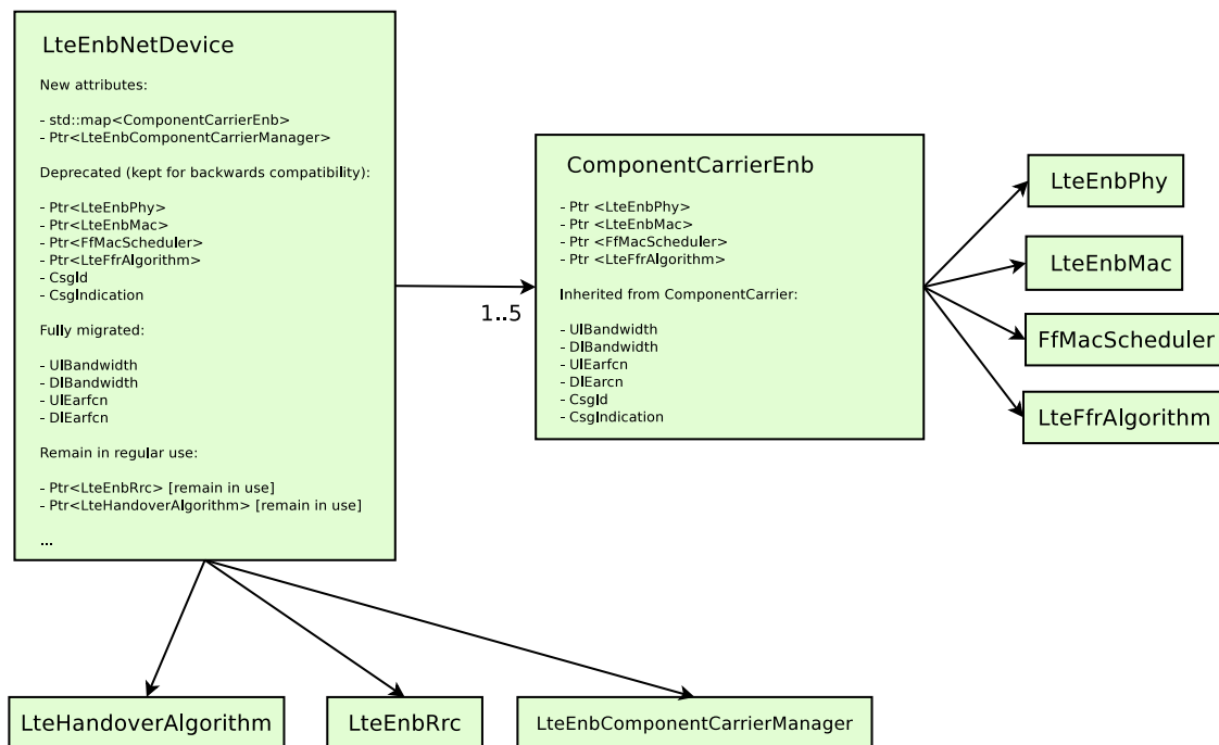
Figure 19.58: Changes in LteEnbNetDevice to support CA
