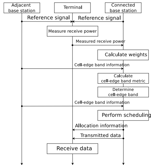
Figure 19.54: Sequence diagram of Distributed Frequency Reuse Scheme
