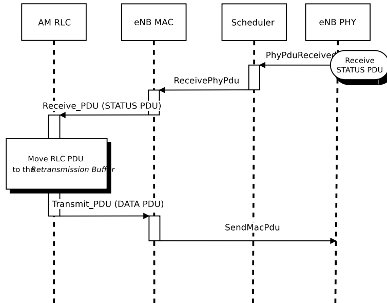
Figure 19.27: Sequence diagram of data PDU retransmission in downlink
