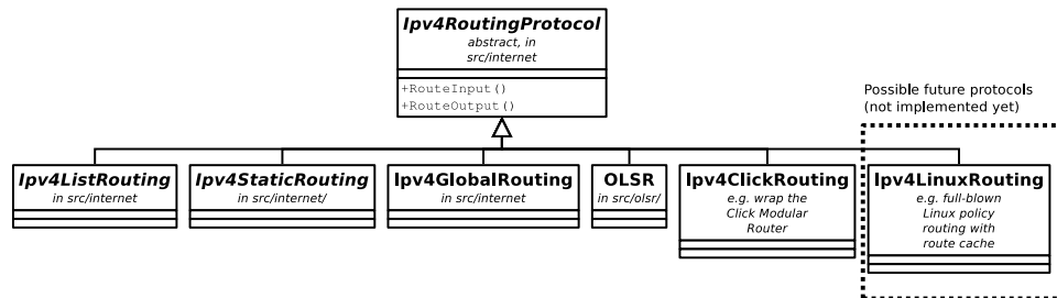
Figure 17.4: Ipv4Routing specialization.
