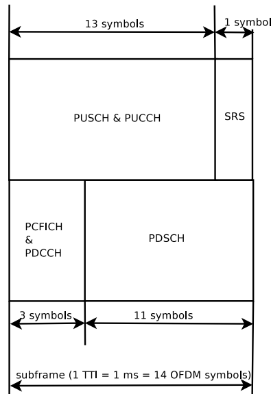
Figure 19.10: LTE subframe division.
