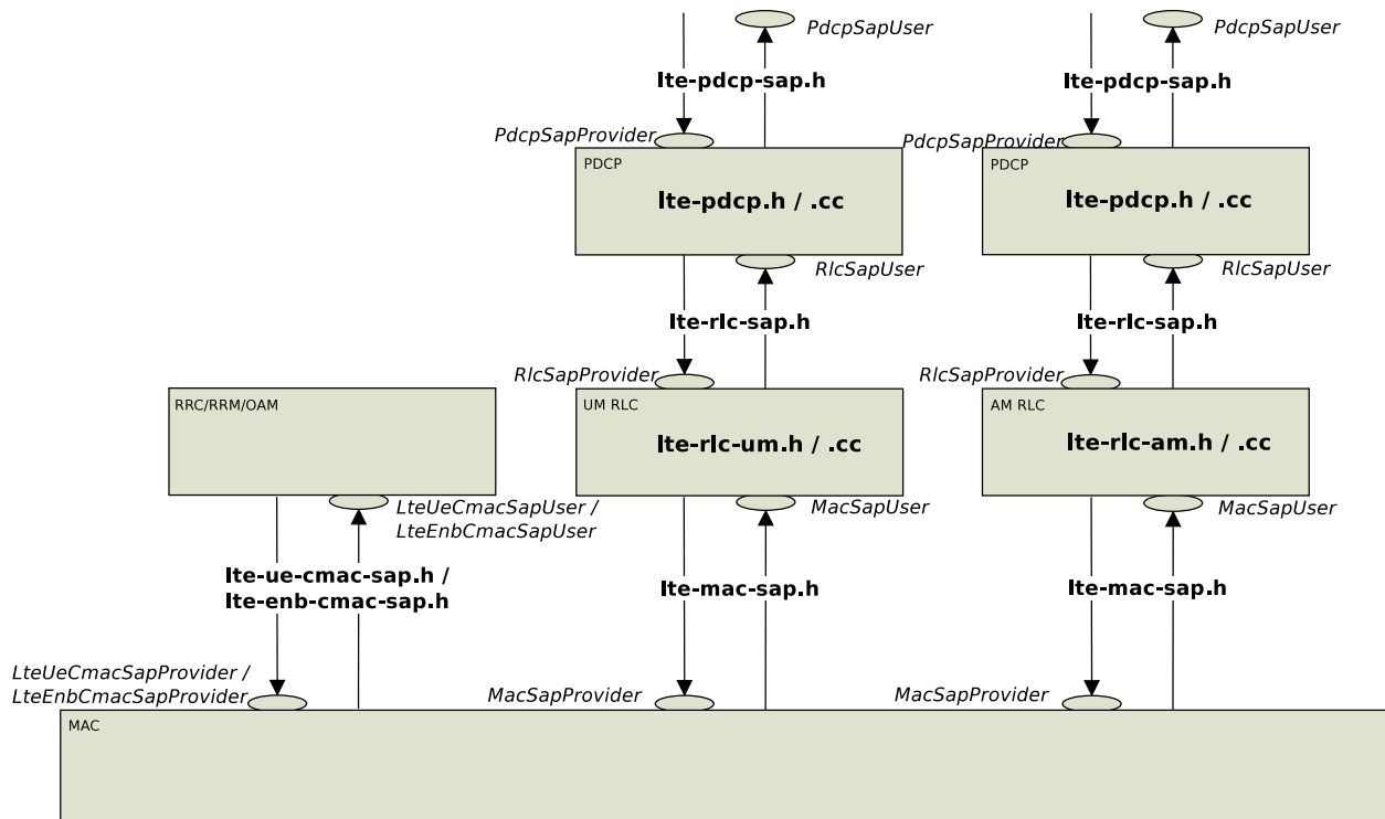
Figure 19.25: Implementation Model of PDCP, RLC and MAC entities and SAPs
