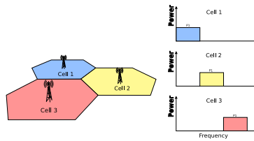
Figure 19.48: Hard Frequency Reuse scheme
