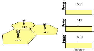
Figure 19.47: Full Frequency Reuse scheme
