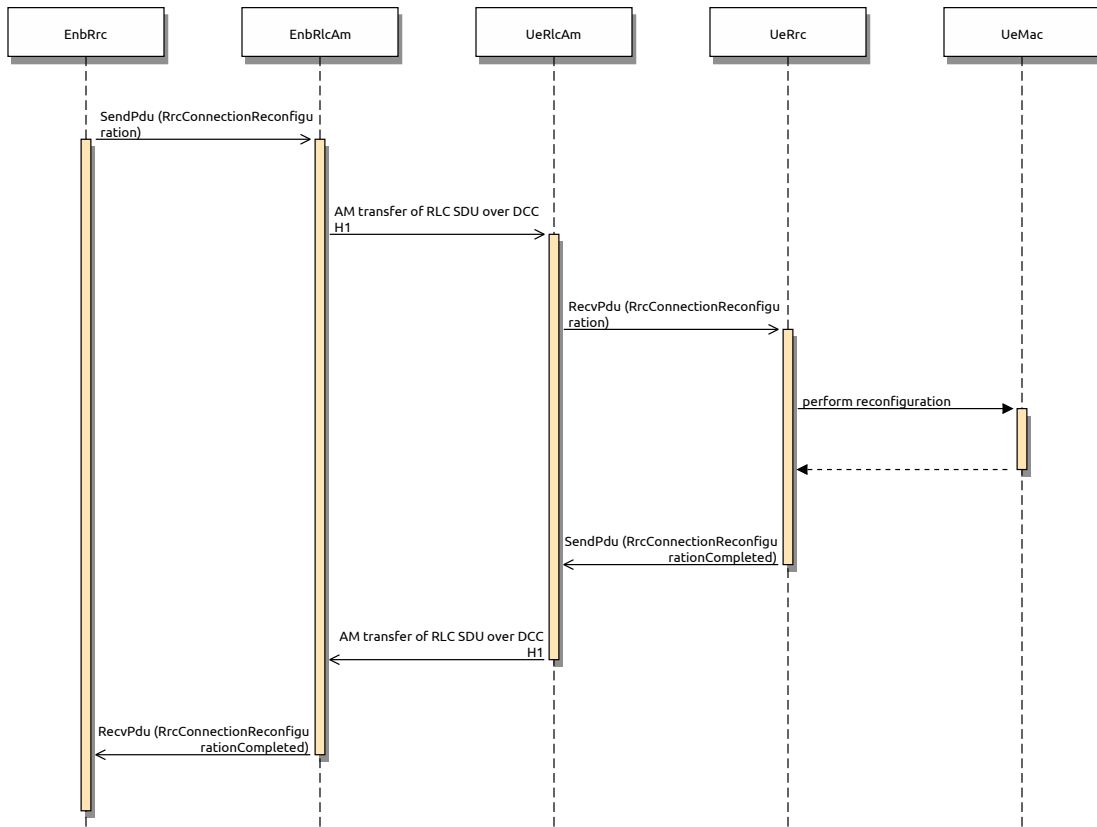
Figure 19.37: Sequence diagram of the RRC Connection Reconfiguration procedure
