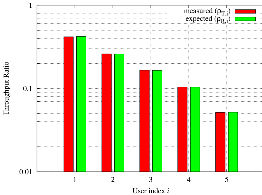
Figure 19.86: Throughput ratio evaluation for the PF scheduler in a scenario where the UEs have MCS index 28, 24, 16, 12, 6
