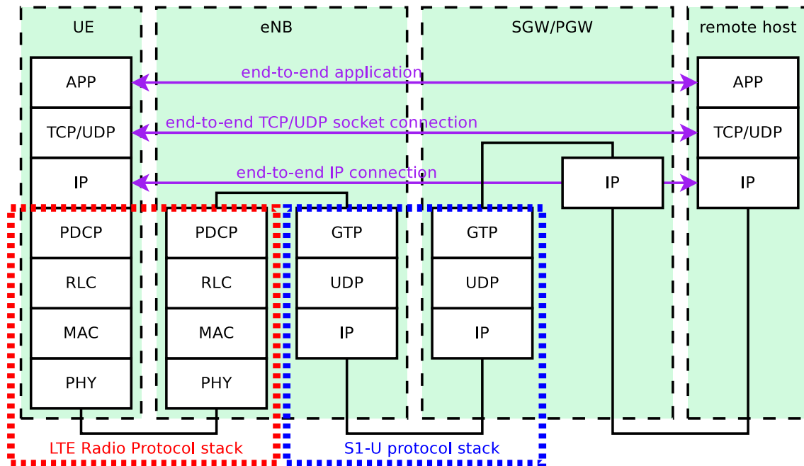
Figure 19.8: LTE-EPC data plane protocol stack
