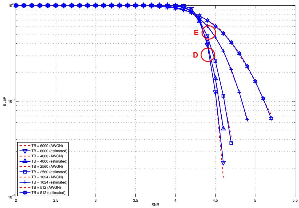
Figure 19.88: BLER for tests 4, 5.
