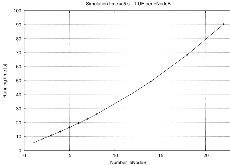
Figure 20.98: Running time
