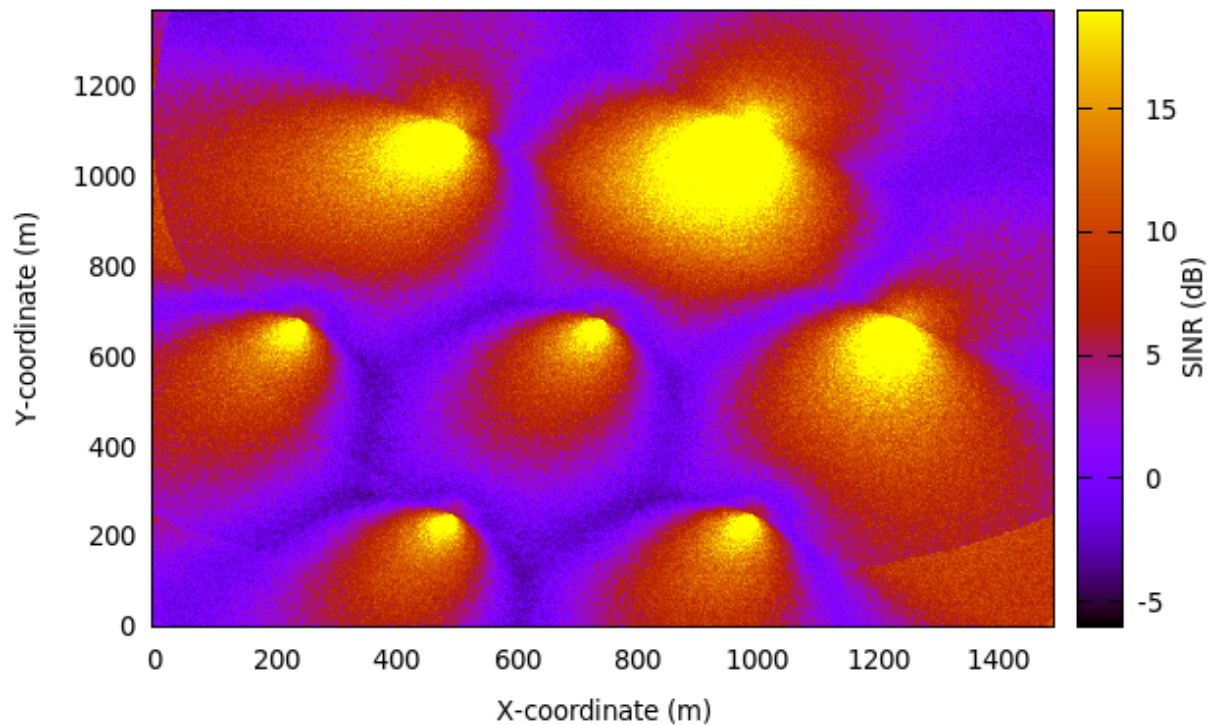
Figure 20.77: REM for RB 20 obtained from lena-dual-stripe simulation with Hard FR algorithm enabled
