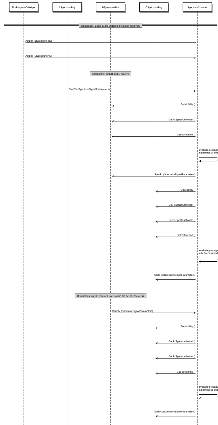
Figure 30.2: Sequence diagram showing the interaction between SpectrumPhy and SpectrumChannel
