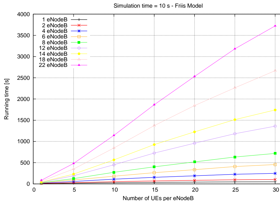
Figure 20.94: Running time
