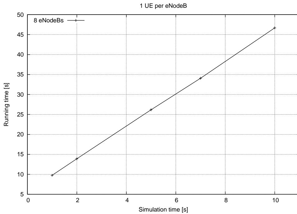
Figure 20.100: Simulation time
