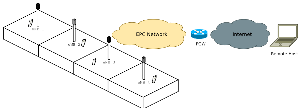
Figure 20.93: Propagation Model
