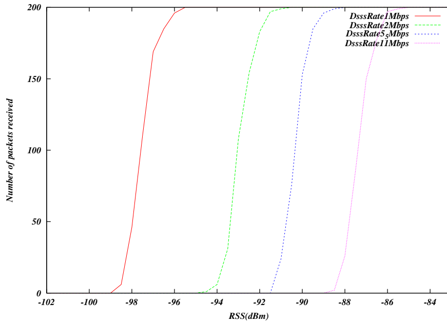
Figure 37.3: Clear channel (AWGN) error model for 802.11b
