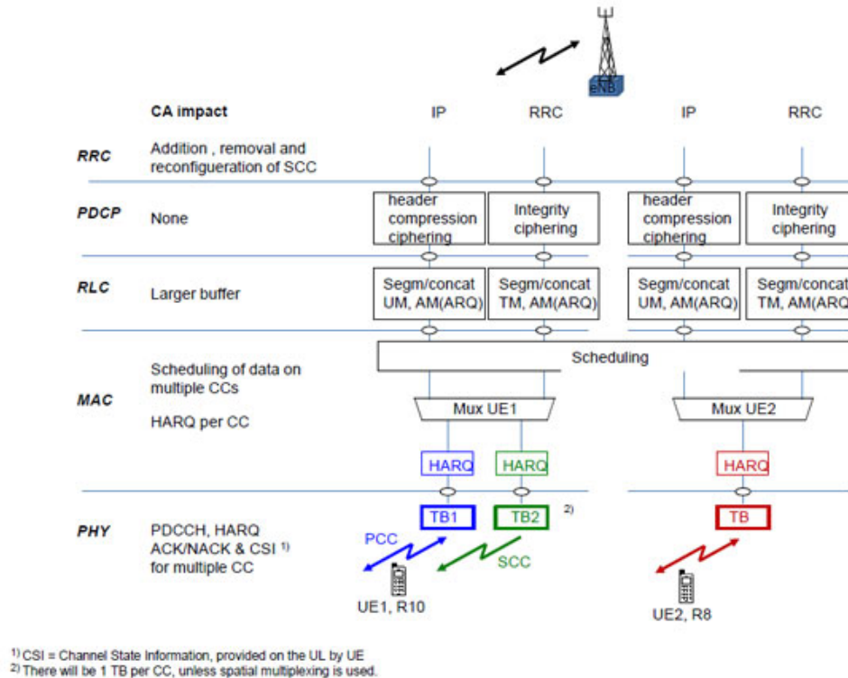
Figure 20.55: CA impact on different layers of LTE protocol stack (from 3gpp.org)
