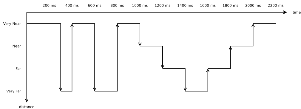
Figure 20.82: UE movement trace throughout the simulation in piecewise configuration
