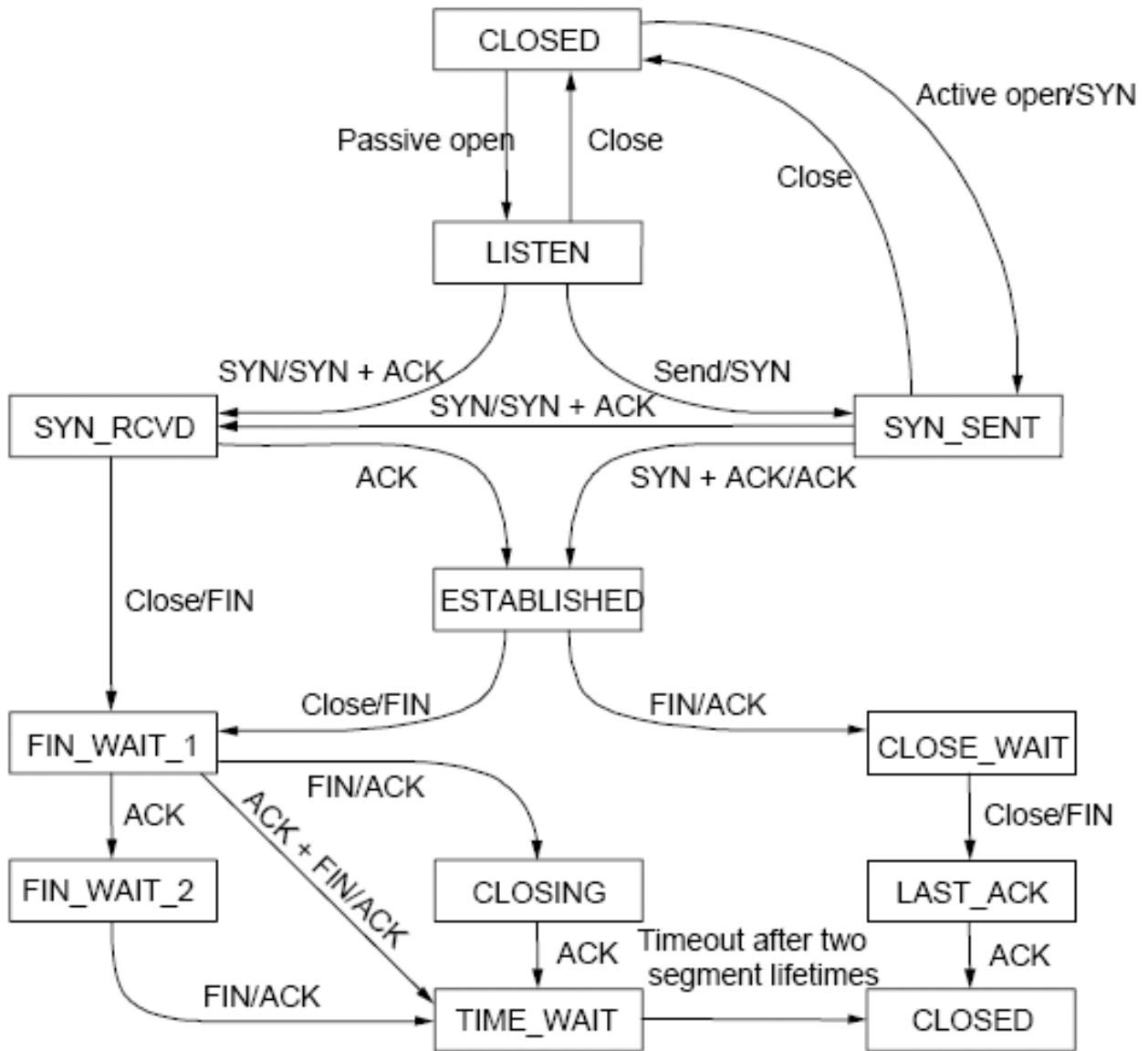
Figure 18.5: TCP State machine
