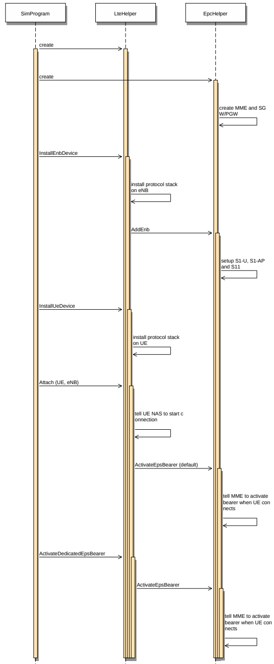
Figure 20.67: Sequence diagram of the interaction between LteHelper and EpcHelper.
