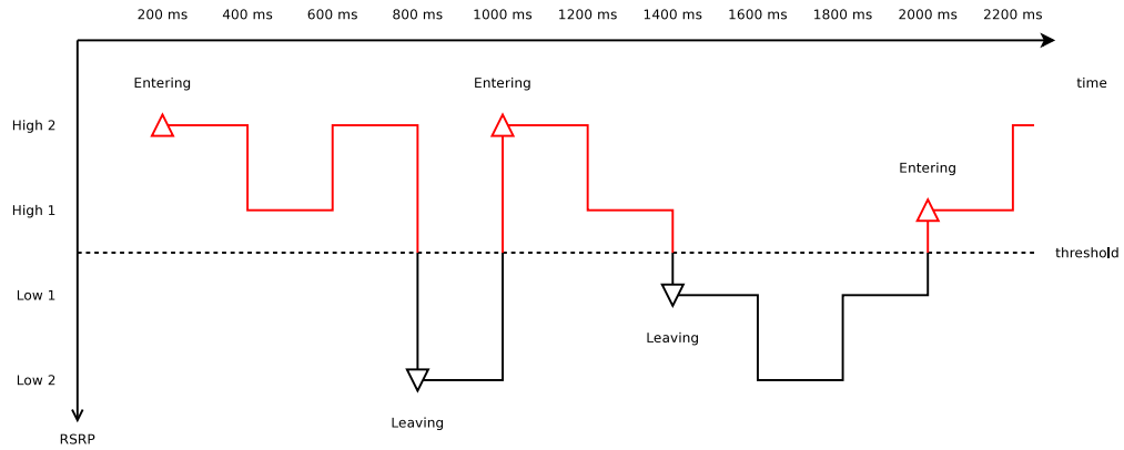
Figure 20.83: Measured RSRP trace of an example Event A1 test case in piecewise configuration
