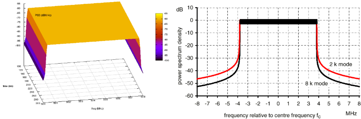
Figure 30.3: 8K COFDM signal spectrum generated from TvSpectrumTransmitter (Left) and theoretical COFDM signal spectrum [KoppCOFDM] (Right)
