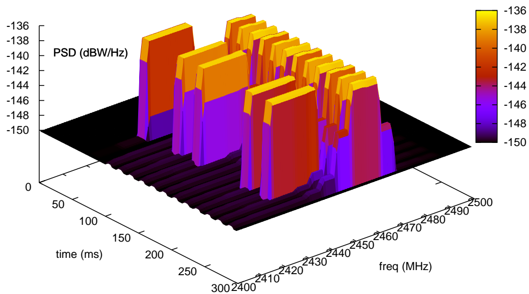
Figure 30.1: Spectrogram produced by a spectrum analyzer in a scenario involving wifi signals interfered by a microwave oven, as simulated by the example adhoc-aloah-ideal-phy-with-microwave-oven .
