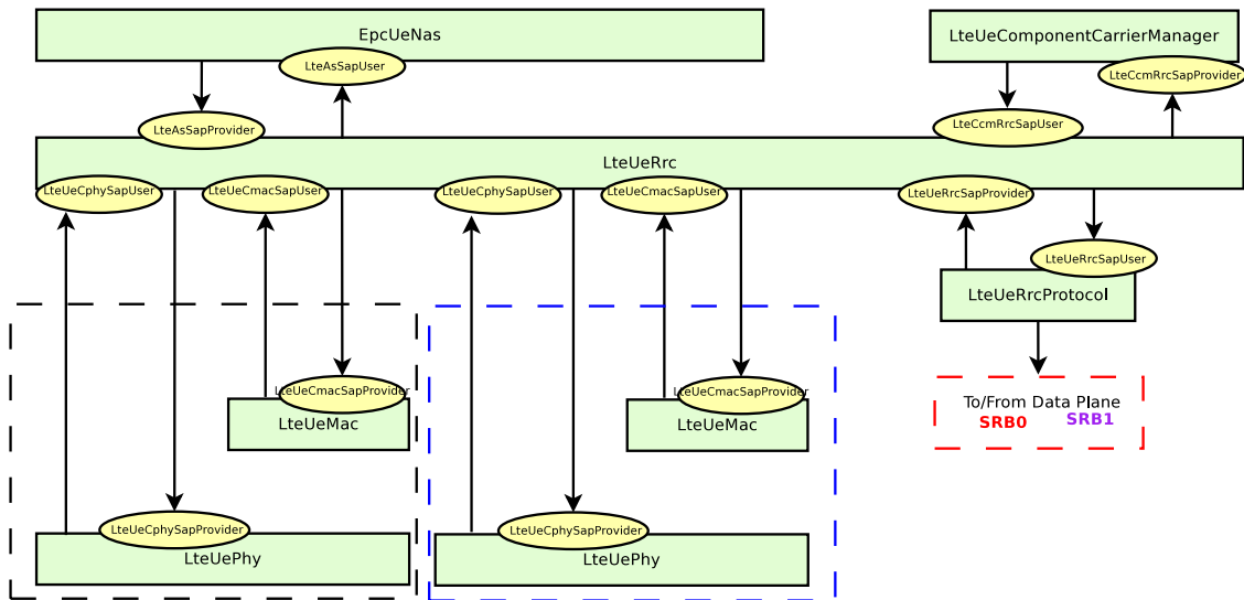
Figure 20.66: UE Control Plane Architecture
