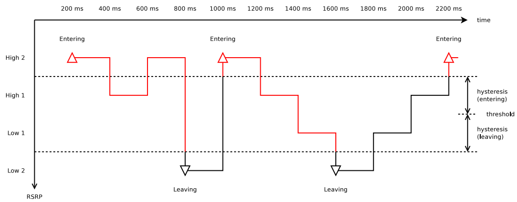
Figure 20.84: Measured RSRP trace of an example Event A1 with hysteresis test case in piecewise configuration
