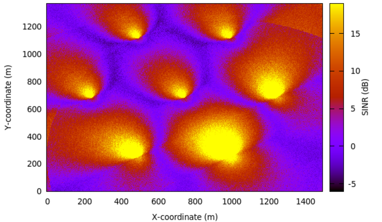
Figure 20.76: REM for RB 10 obtained from lena-dual-stripe simulation with Hard FR algorithm enabled
