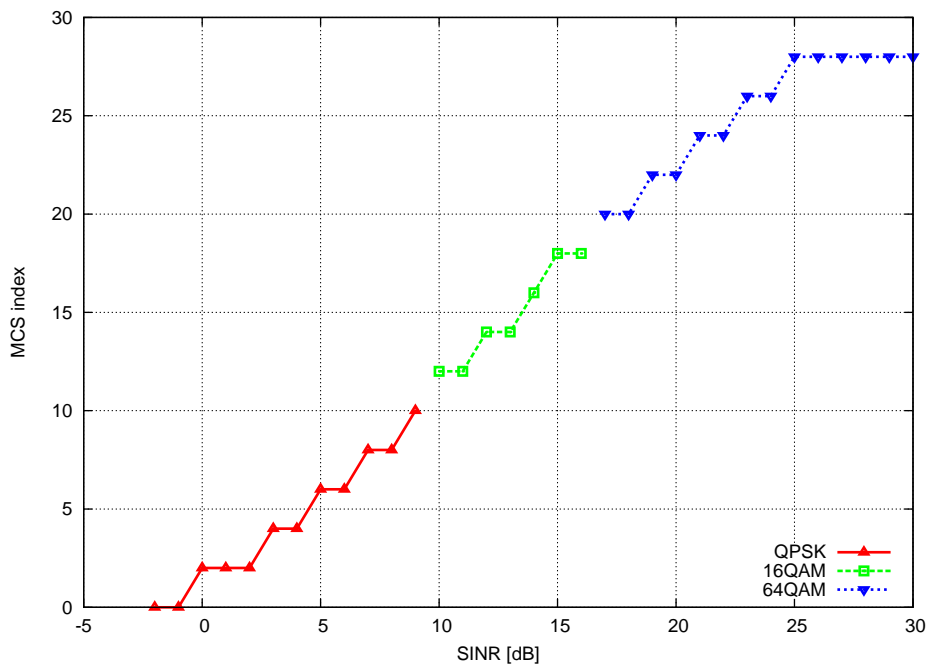
Figure 20.80: Test vector for Adaptive Modulation and Coding
