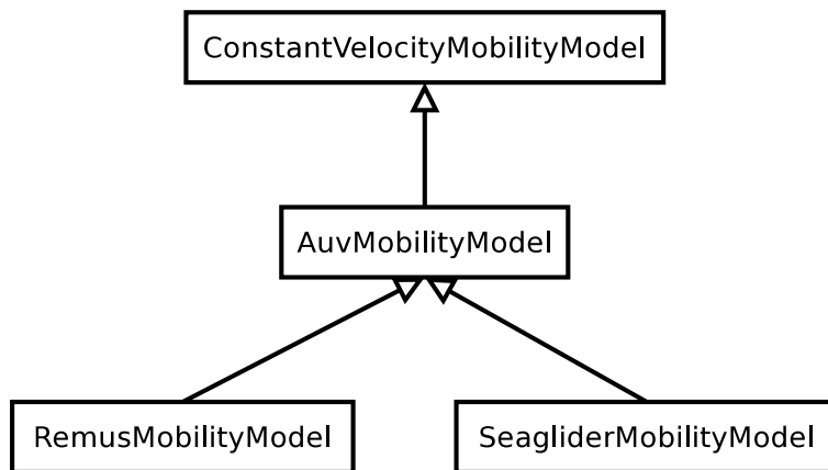
Figure 35.1: AUV’s mobility model classes overview
