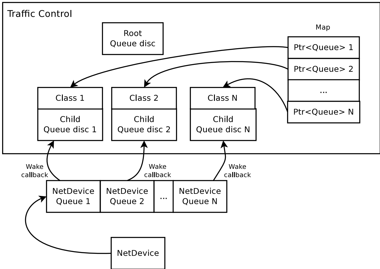
Figure 34.2: Setup of a multi-queue aware queue disc
