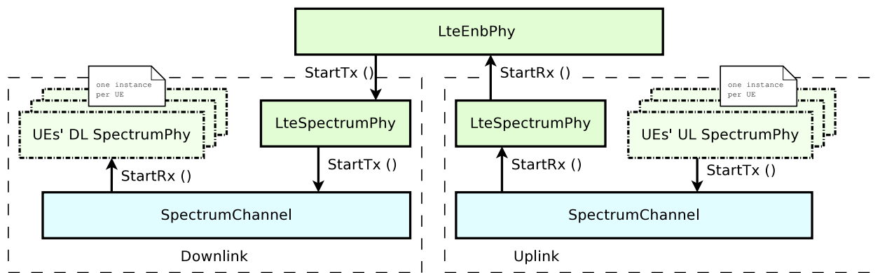
Figure 20.7: PHY and channel model architecture for the eNB
