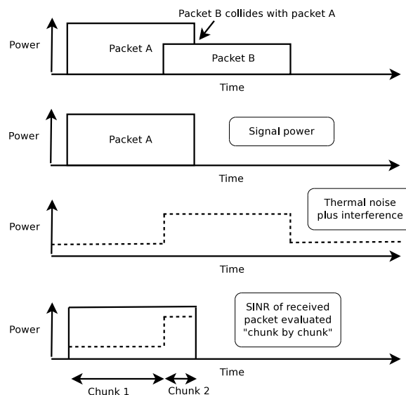
Figure 37.2: SNIR function over time .
