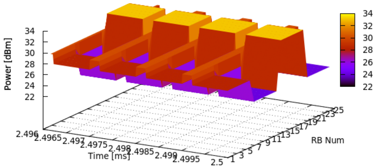
Figure 20.74: Spectrum Analyzer trace obtained from lena-frequency-reuse example with Soft FFR algorithm enabled. Spectrum Analyzer was located near eNB with FrCellTypeId 2 .
