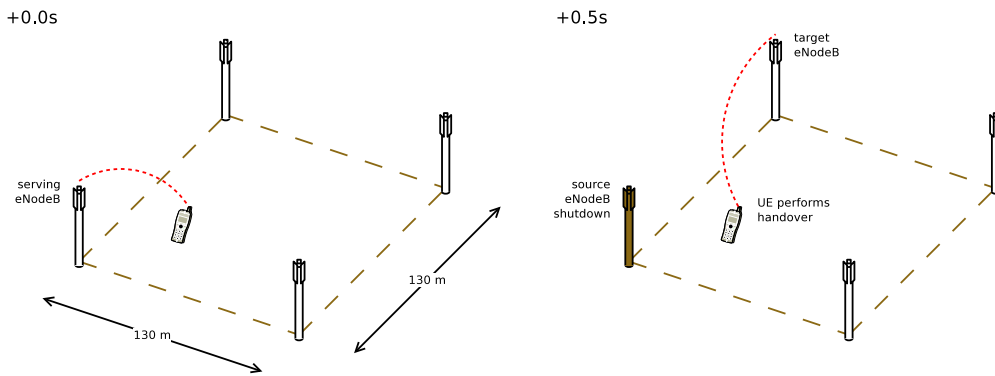
Figure 20.91: lte-handover-target test scenario in a 2x2 grid
