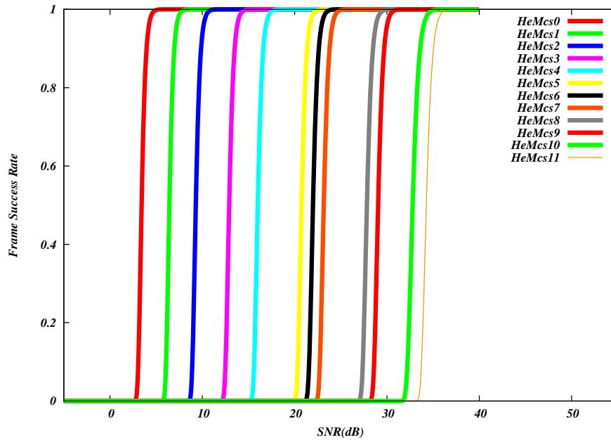
Figure 37.7: Frame error rate (NIST model) for 802.11ax (HE OFDM) Wi-Fi
