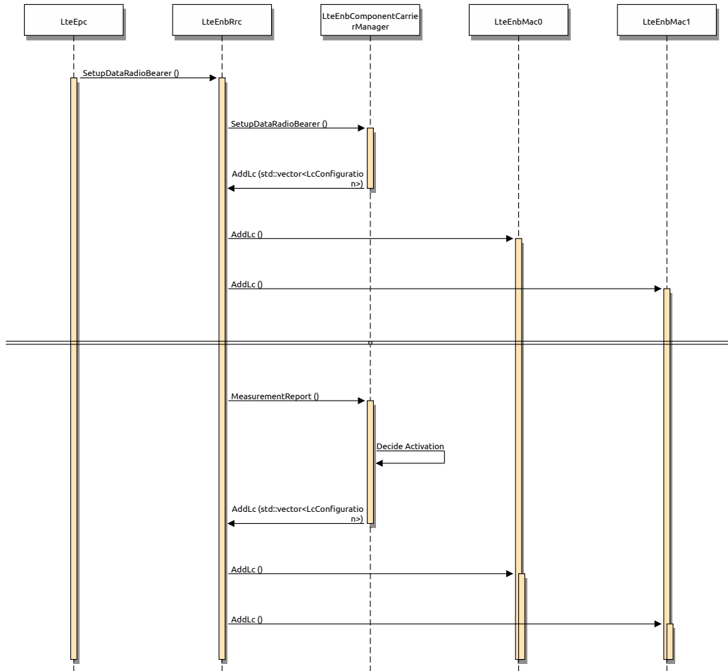
Figure 20.63: Sequence Diagram of Data Radio Bearer Setup
