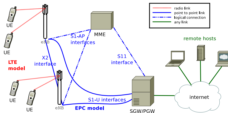
Figure 20.1: Overview of the LTE-EPC simulation model
