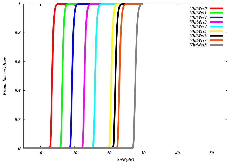
Figure 37.6: Frame error rate (NIST model) for 802.11ac (VHT OFDM) Wi-Fi
