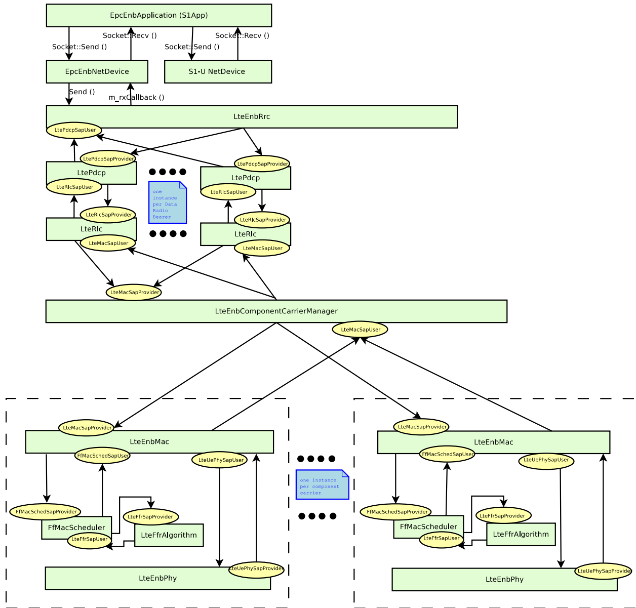
Figure 20.60: eNB Data Plane Architecture
