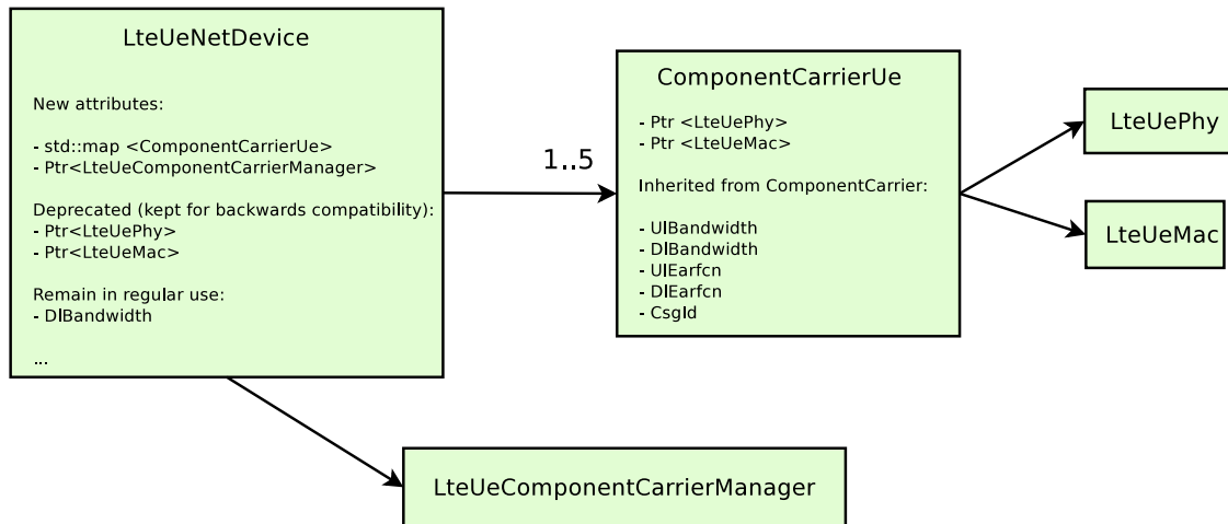
Figure 20.59: Changes in LteUeNetDevice to support CA
