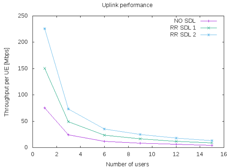
Figure 20.78: Example of CA test performance in the uplink
