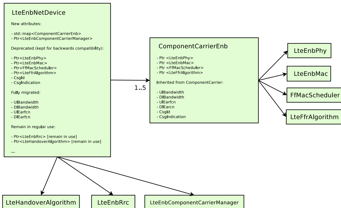
Figure 20.58: Changes in LteEnbNetDevice to support CA
