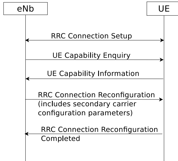
Figure 20.56: A schematic overview of the secondary carrier enabling procedure
