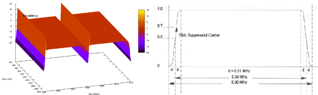
Figure 30.4: North America ATSC channel 19 & 20 signals generated using TvSpectrumTransmitterHelper (Left) and theoretical 8-VSB signal [Baron8VSB] (Right). Note that the theoretical signal is not shown in dB while the ns-3 generated signals are.
