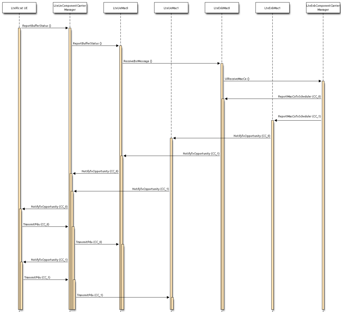
Figure 20.65: Uplink buffer status reporting with CA
