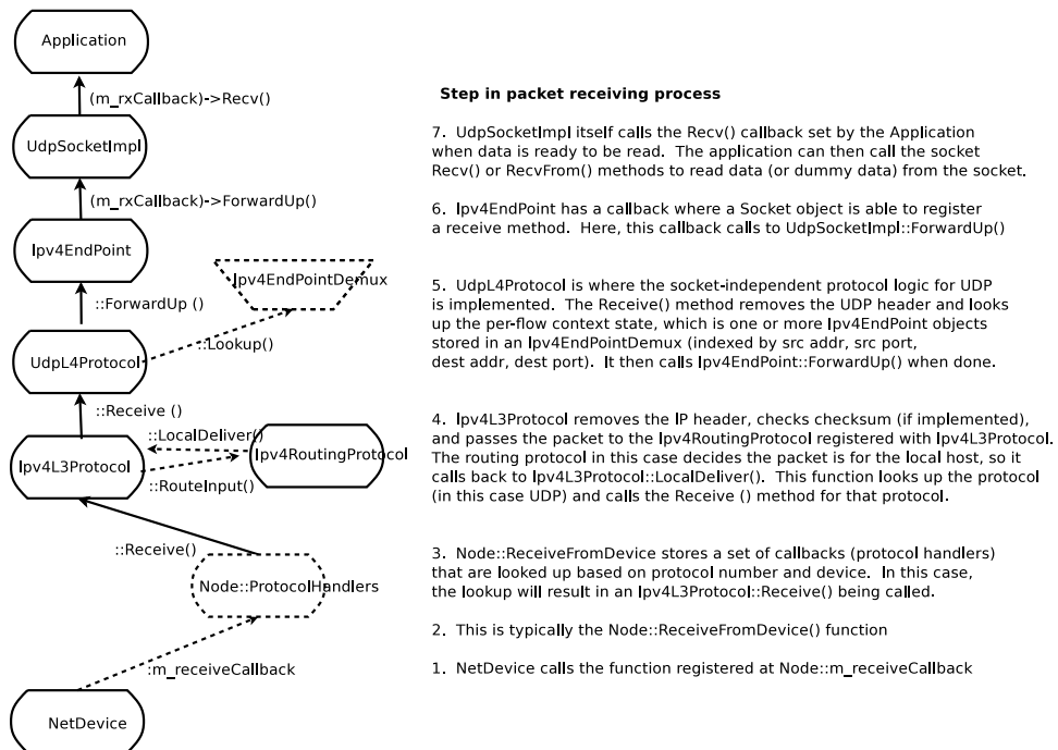
Figure 18.2: Receive path of a packet.
