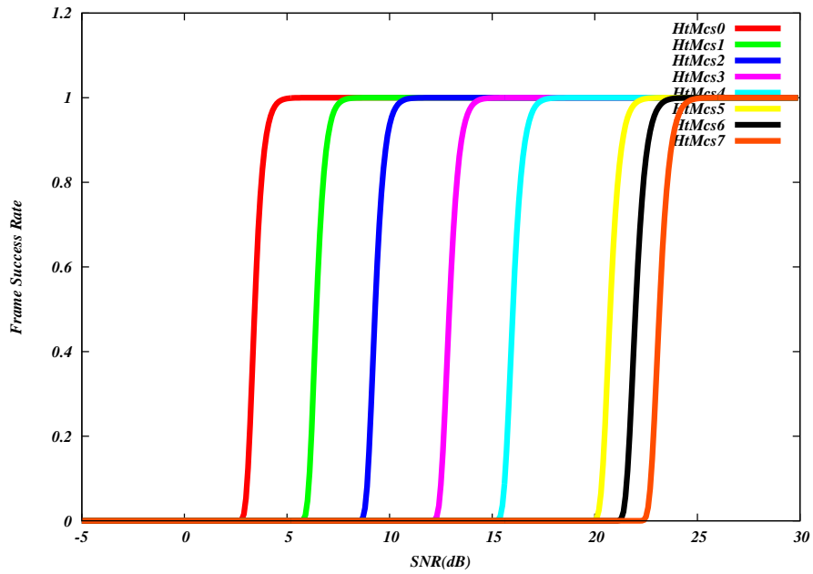
Figure 37.5: Frame error rate (NIST model) for 802.11n (HT OFDM) Wi-Fi
