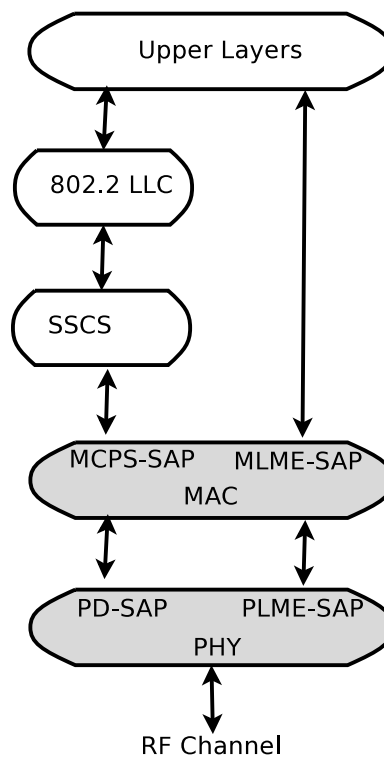
Figure 19.1: Architecture and scope of lr-wpan models
