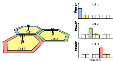
Figure 20.53: Enhanced Fractional Fractional Frequency Reuse scheme
