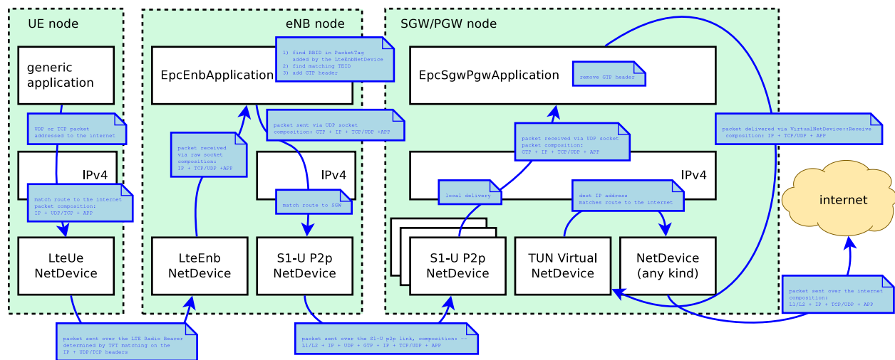
Figure 20.41: Data flow in the uplink between the UE and the internet
