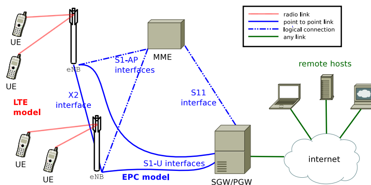
Figure 20.1: Overview of the LTE-EPC simulation model
