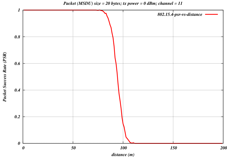
Figure 19.5: Default output of the program lr-wpan-error-distance-plot.cc
