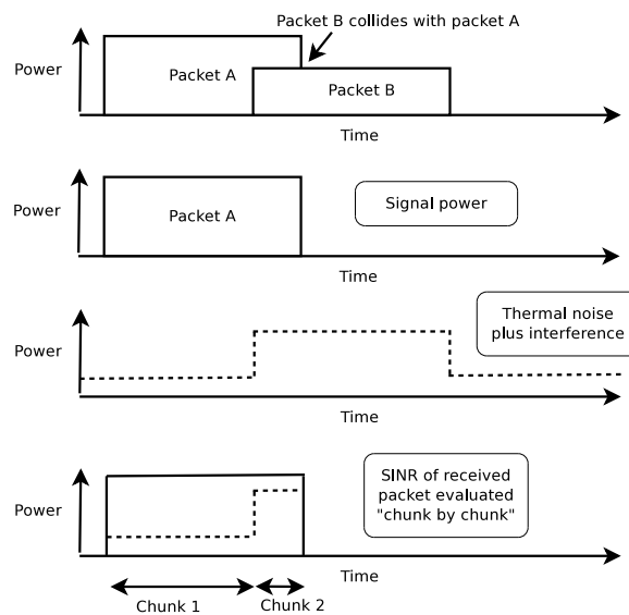
Figure 36.2: SNIR function over time .
