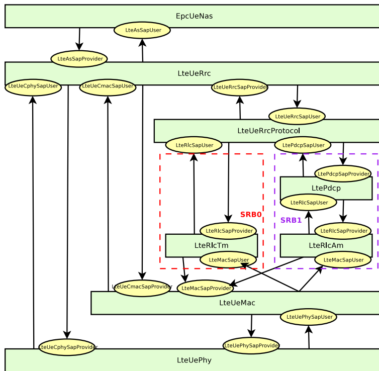
Figure 20.3: LTE radio protocol stack architecture for the UE on the control plane
