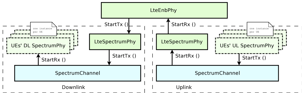
Figure 20.7: PHY and channel model architecture for the eNB
