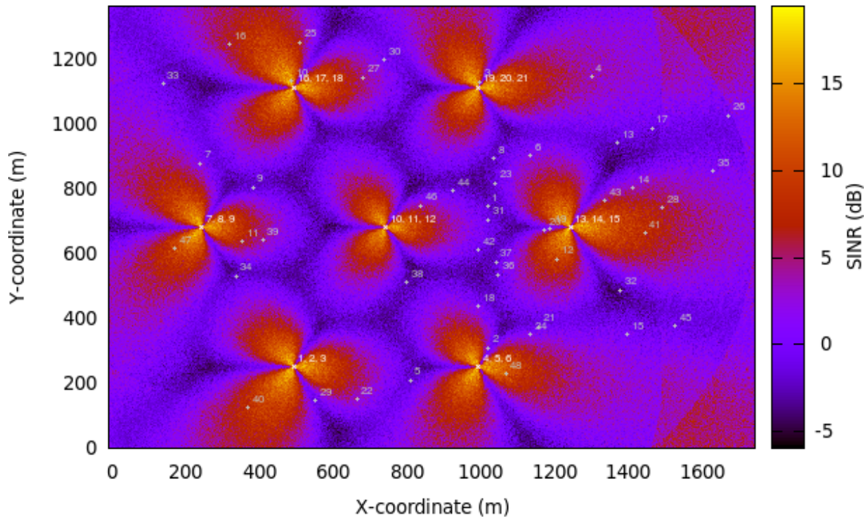
Figure 20.60: REM obtained from a simulation in handover campaign
