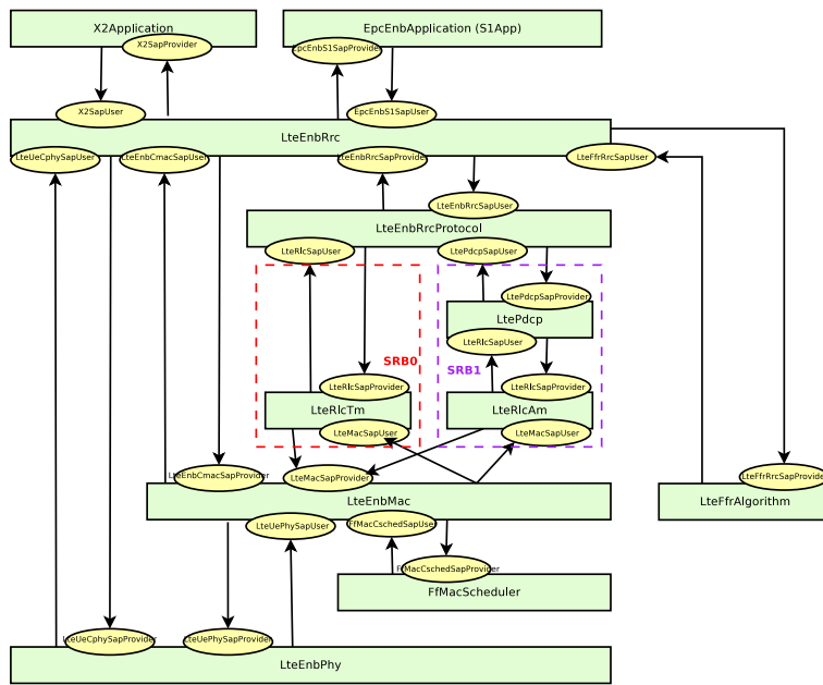
Figure 20.6: LTE radio protocol stack architecture for the eNB on the control plane
