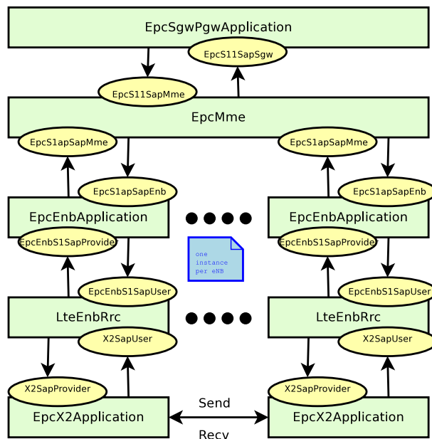
Figure 20.9: EPC control model
