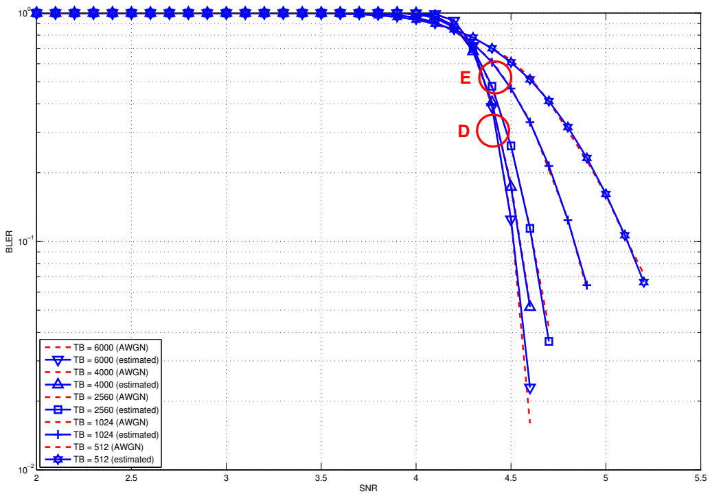
Figure 20.74: BLER for tests 4, 5.
