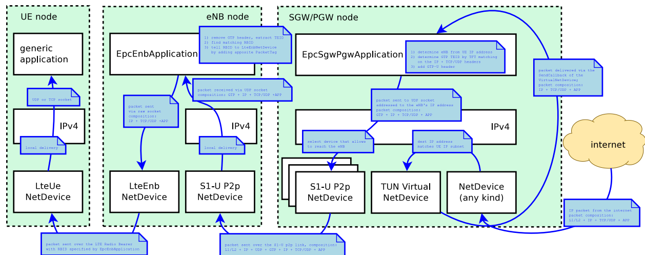
Figure 20.40: Data flow in the downlink between the internet and the UE
