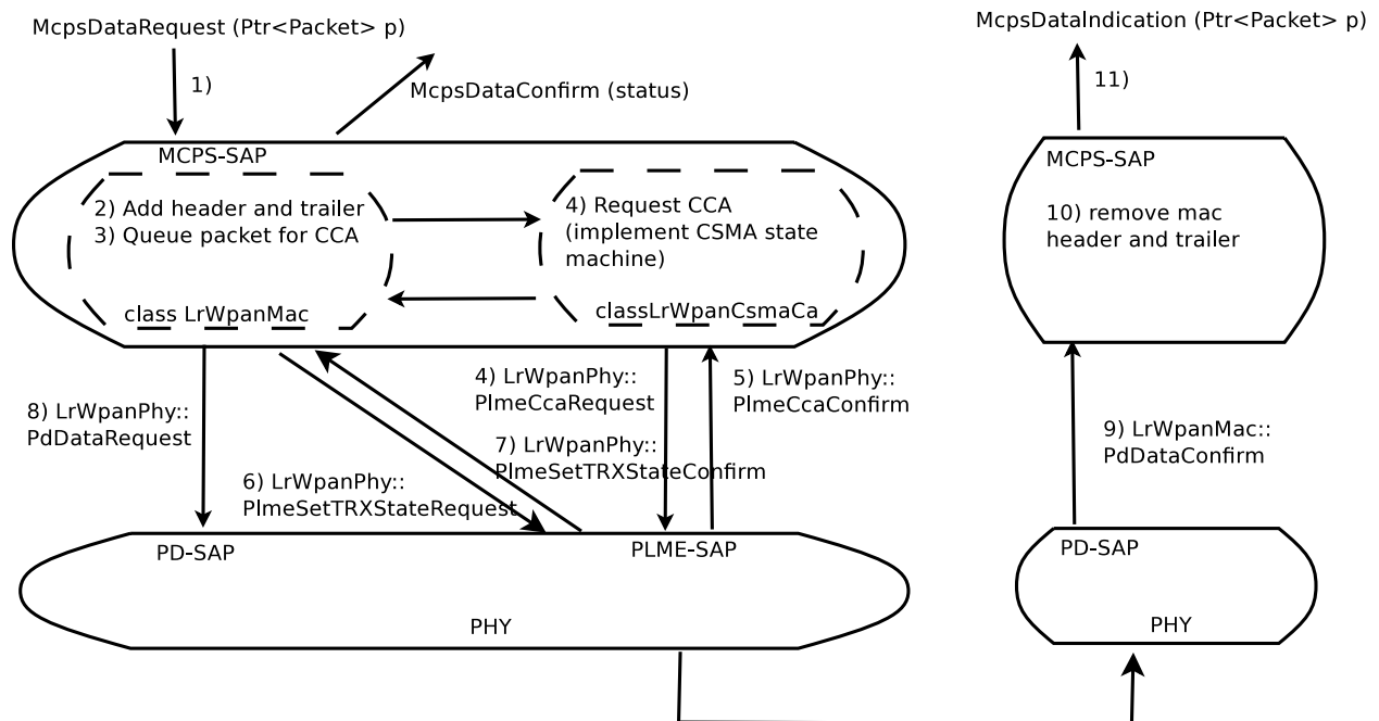
Figure 19.4: Data example for simple LR-WPAN data transfer end-to-end
