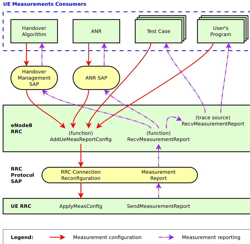
Figure 20.33: Relationship between UE measurements and its consumers
