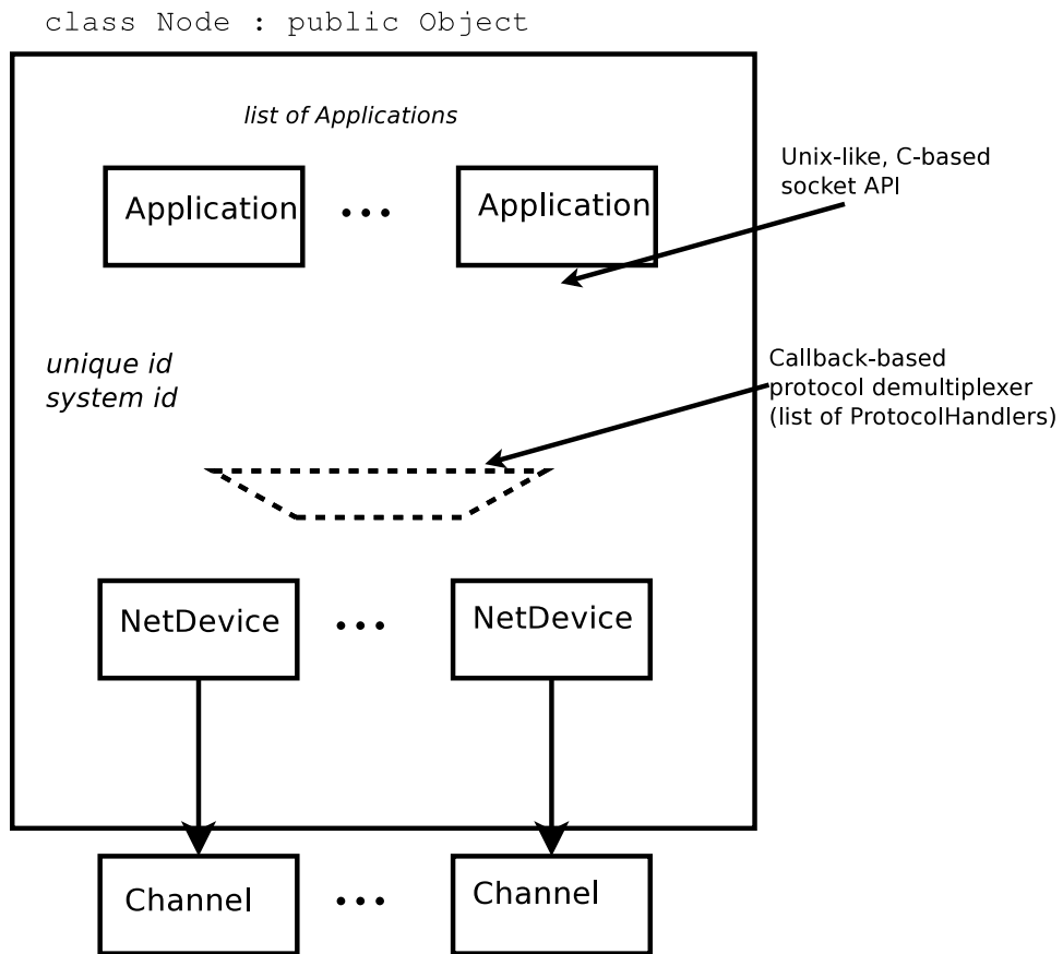
Figure 24.3: High-level node architecture
