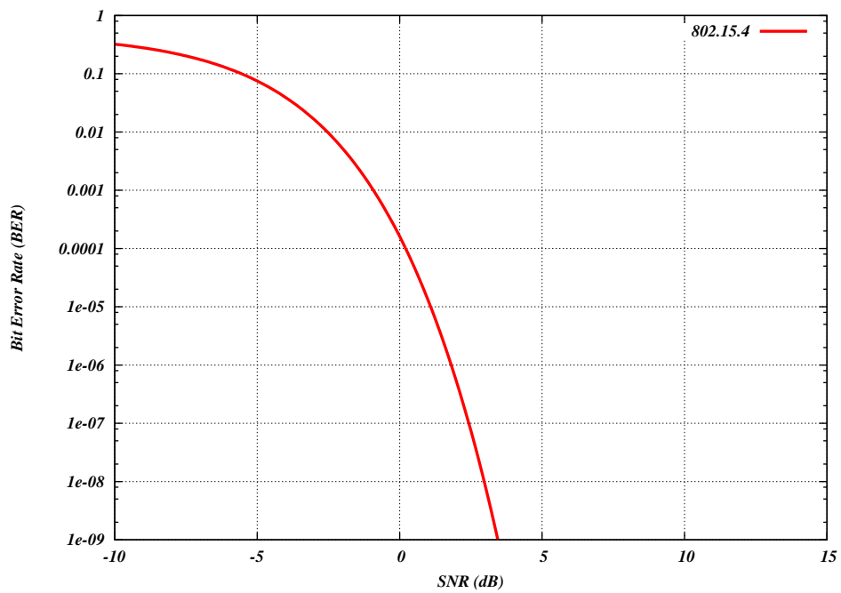
Figure 19.6: Default output of the program lr-wpan-error-model-plot.cc
