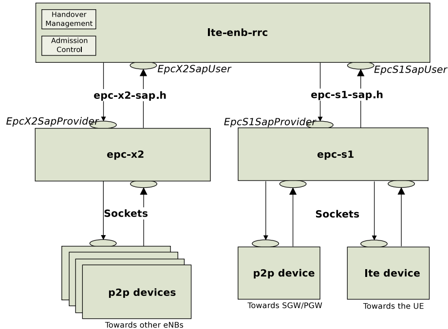
Figure 20.43: Implementation Model of X2 entity and SAPs
