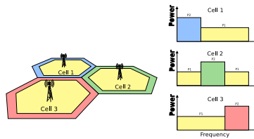
Figure 20.51: Soft Frequency Reuse scheme version 2
