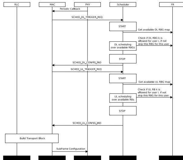
Figure 20.46: Sequence diagram of Scheduling with FR algorithm
