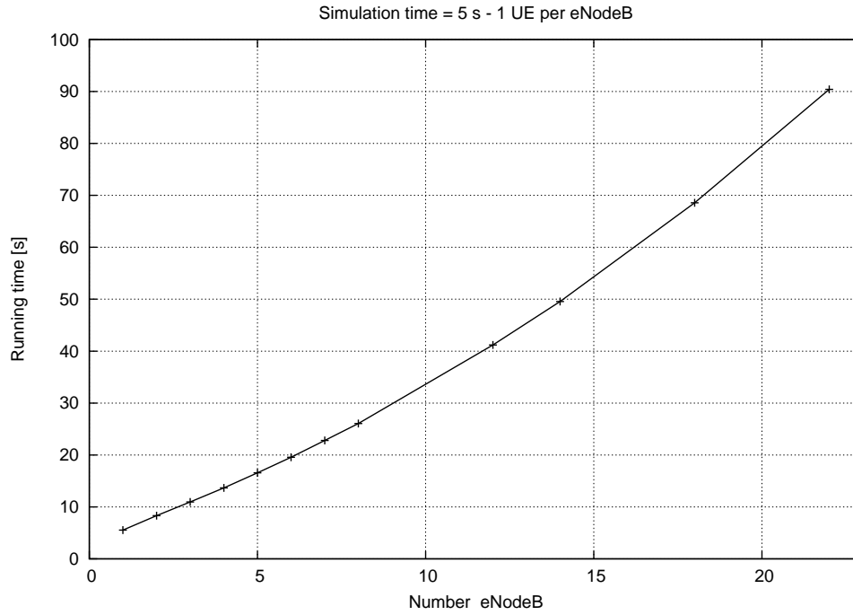
Figure 20.84: Running time
