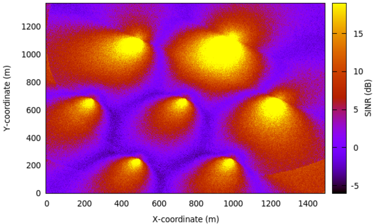
Figure 20.65: REM for RB 20 obtained from lena-dual-stripe simulation with Hard FR algorithm enabled
