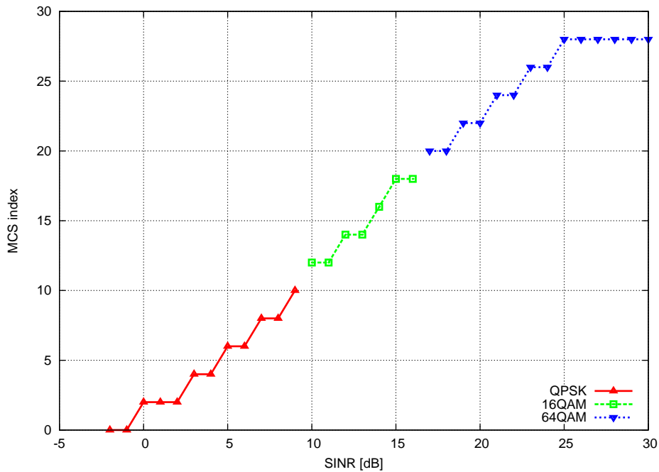
Figure 20.66: Test vector for Adaptive Modulation and Coding
