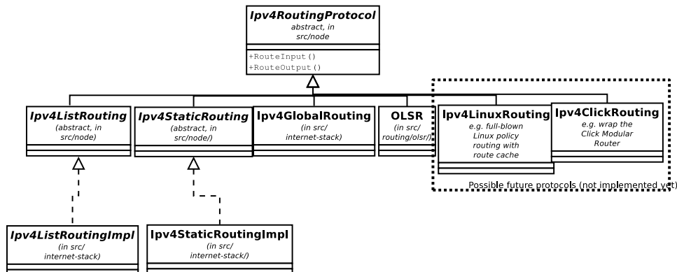
Figure 18.4: Ipv4Routing specialization.
