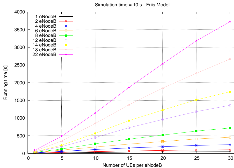
Figure 20.80: Running time
