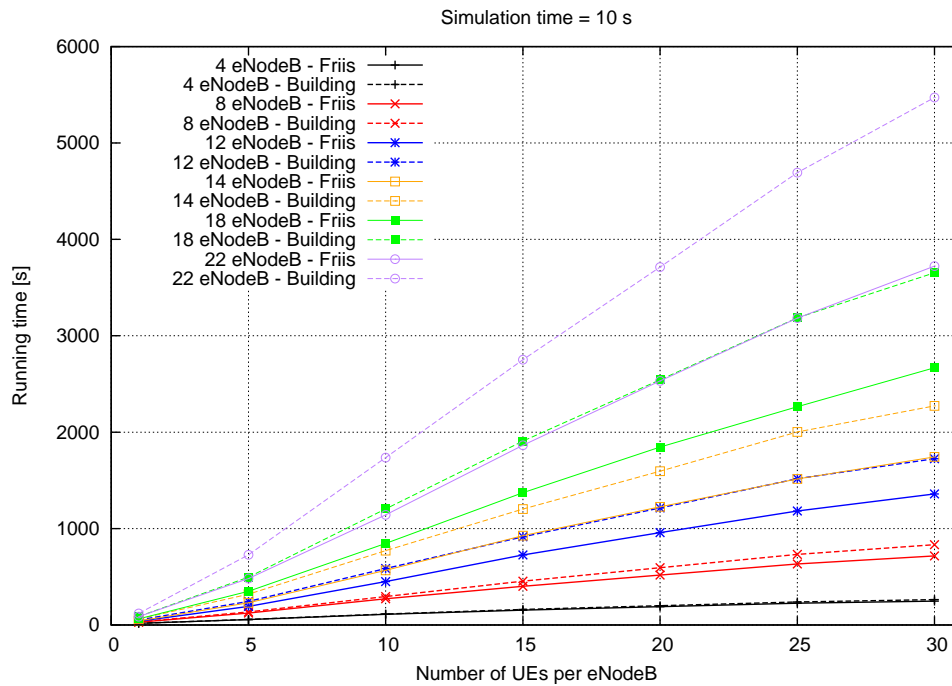
Figure 20.81: Propagation Model
