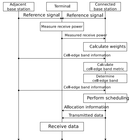
Figure 20.54: Sequence diagram of Distributed Frequency Reuse Scheme
