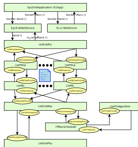
Figure 20.5: LTE radio protocol stack architecture for the eNB on the data plane
