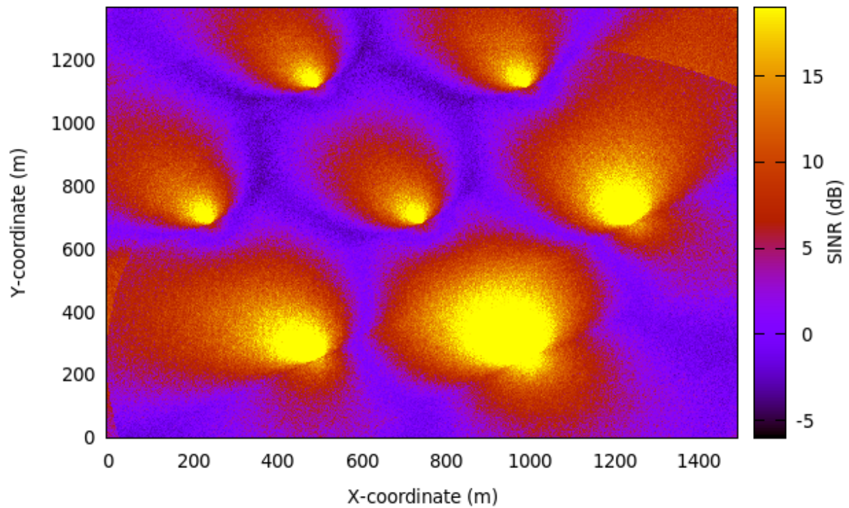
Figure 20.64: REM for RB 10 obtained from lena-dual-stripe simulation with Hard FR algorithm enabled
