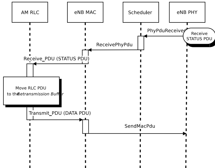
Figure 20.27: Sequence diagram of data PDU retransmission in downlink
