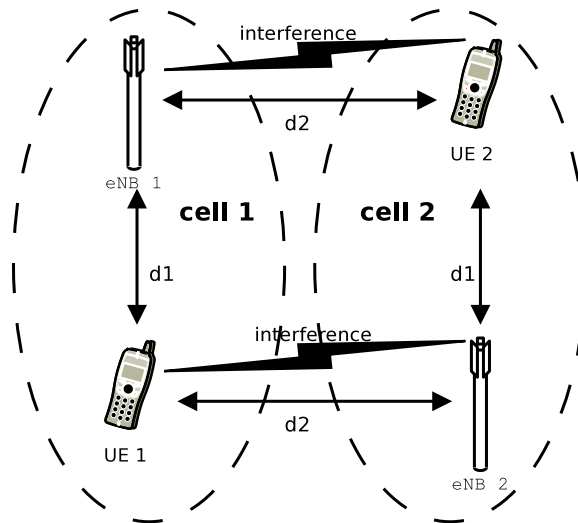
Figure 20.67: Topology for the inter-cell interference test
