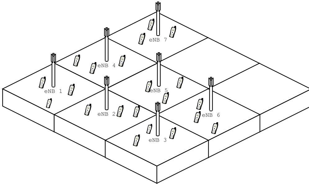
Figure 20.78: E-UTRAN
