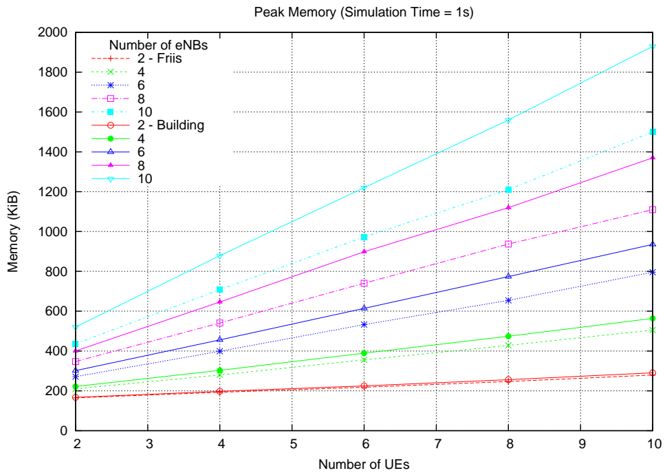
Figure 20.83: Memory profile
