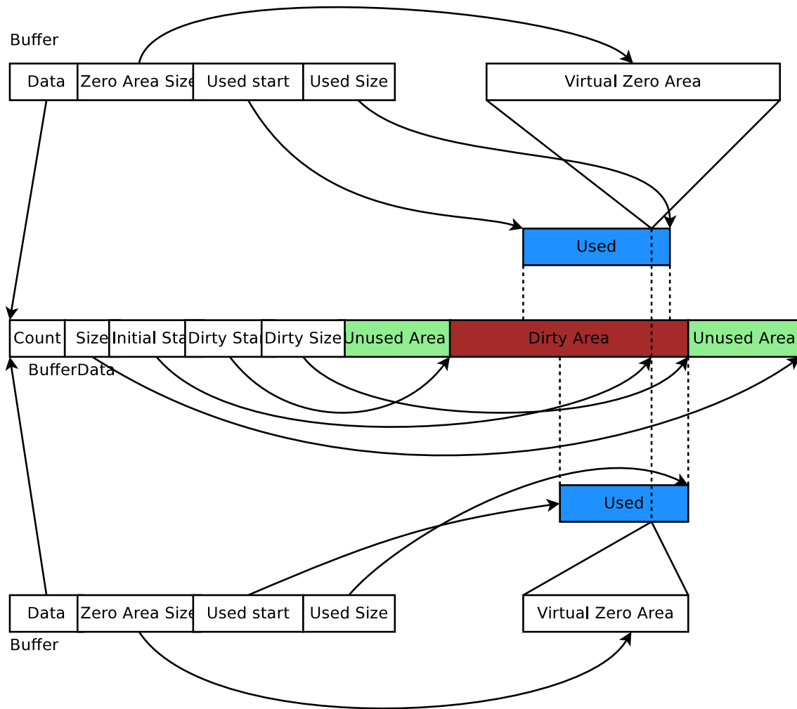
Figure 24.2: Implementation overview of a packet's byte Buffer.
