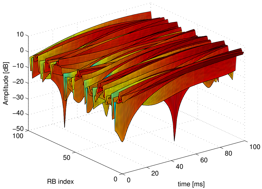
Figure 20.58: Excerpt of the fading trace included in the simulator for an urban scenario (speed of 3 kmph).
