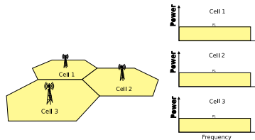
Figure 20.47: Full Frequency Reuse scheme
