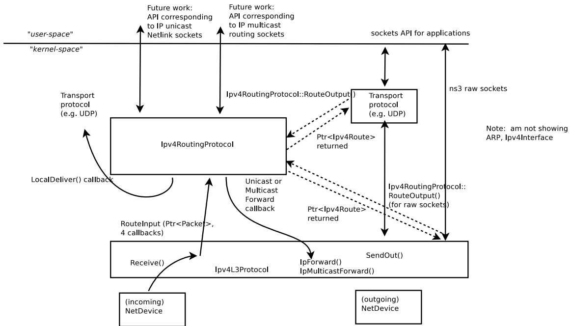
Figure 18.3: Overview of routing
