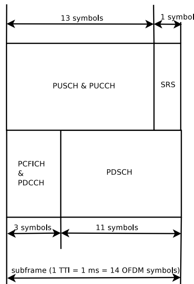
Figure 20.10: LTE subframe division.
