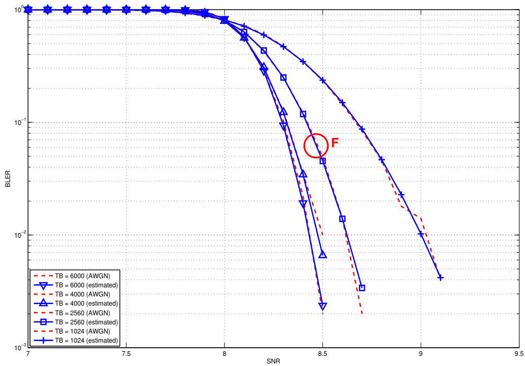
Figure 20.75: BLER for test 6.
