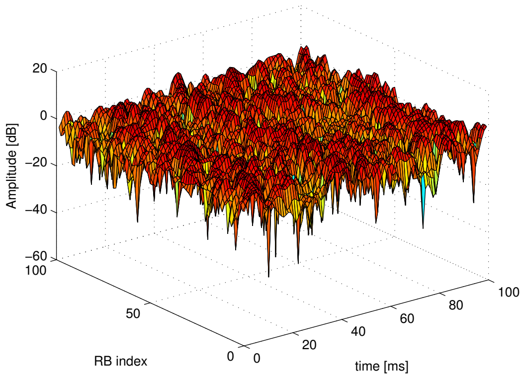
Figure 20.57: Excerpt of the fading trace included in the simulator for a vehicular scenario (speed of 60 kmph).
