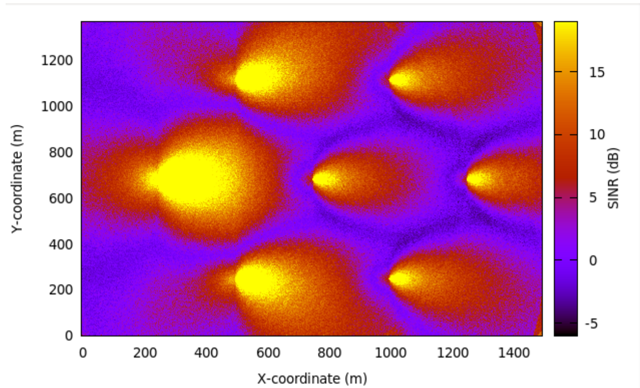
Figure 20.63: REM for RB 1 obtained from lena-dual-stripe simulation with Hard FR algorithm enabled
