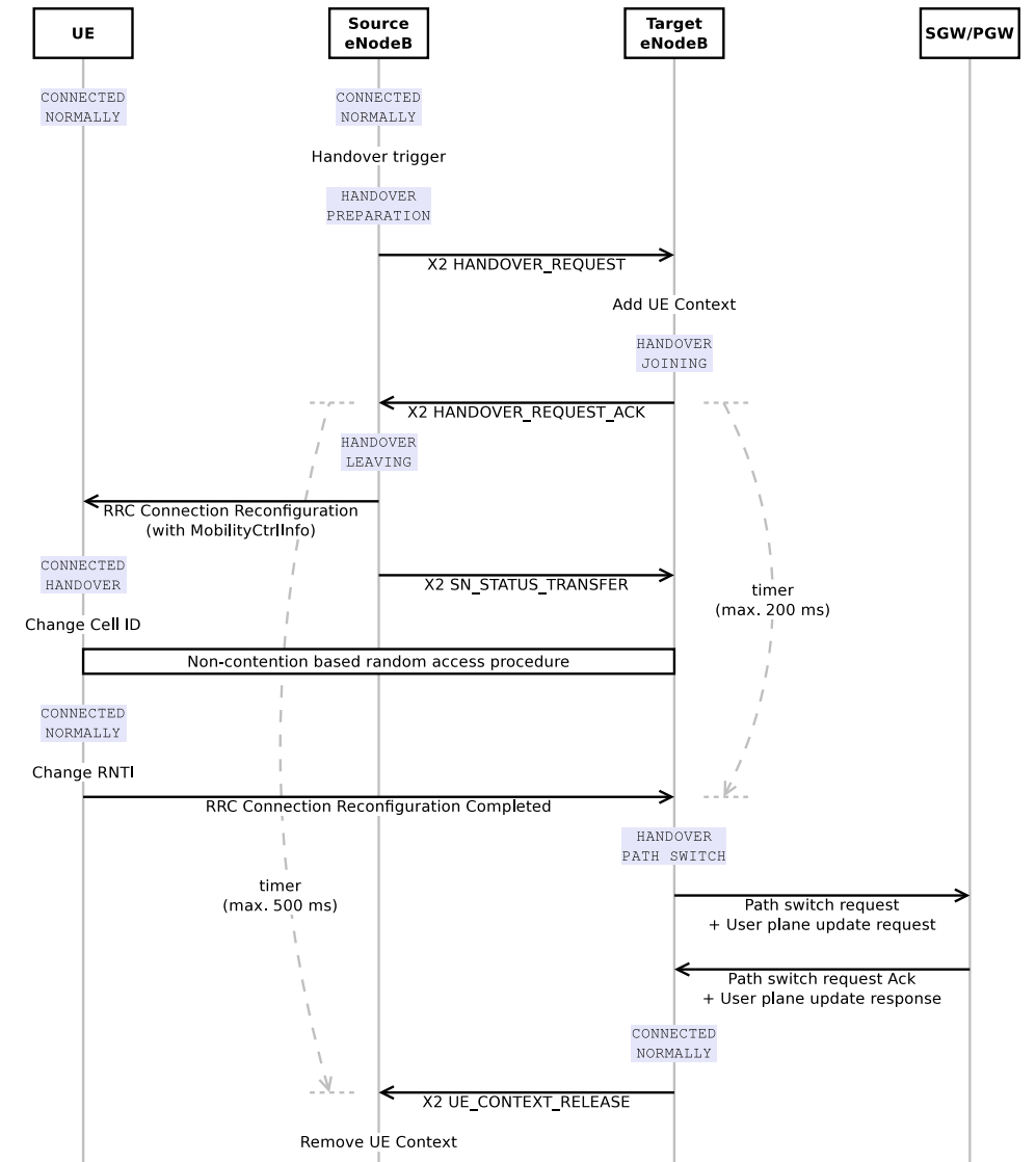
Figure 20.42: Sequence diagram of the X2-based handover
