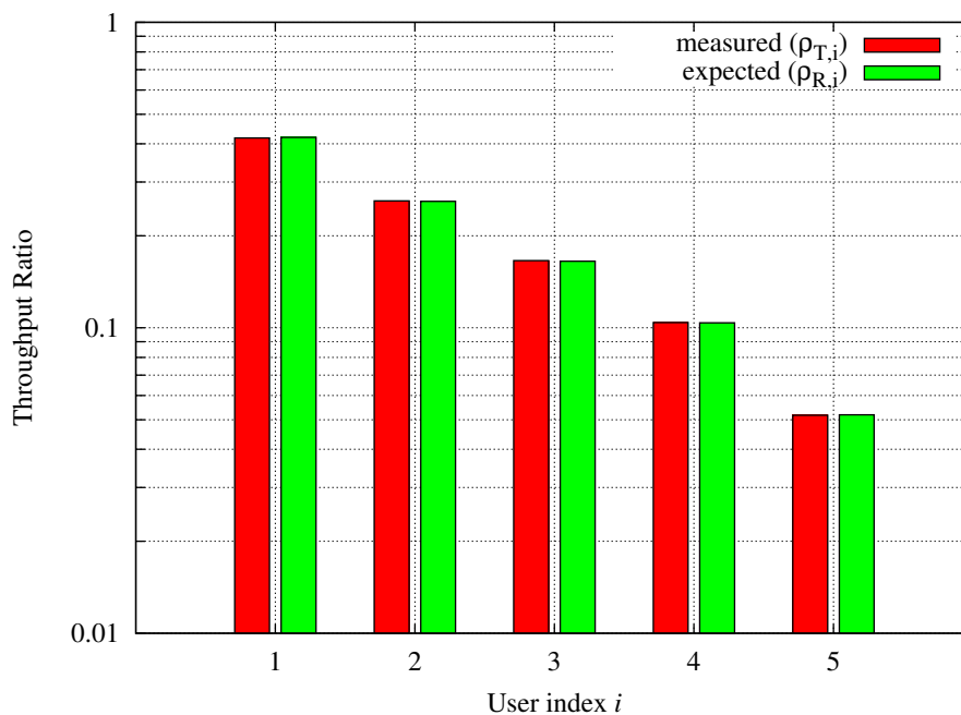
Figure 20.72: Throughput ratio evaluation for the PF scheduler in a scenario where the UEs have MCS index 28, 24, 16, 12, 6
