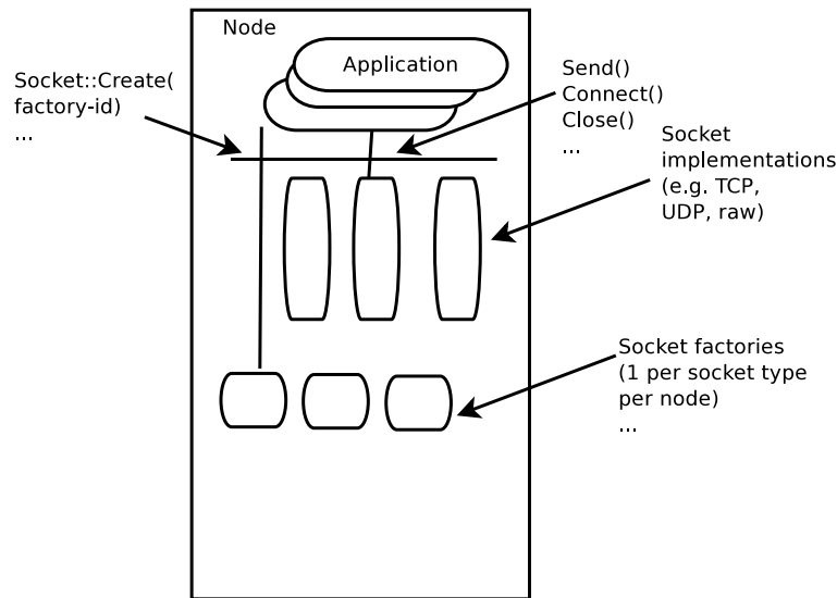
Figure 24.4: Implementation overview of native sockets API
