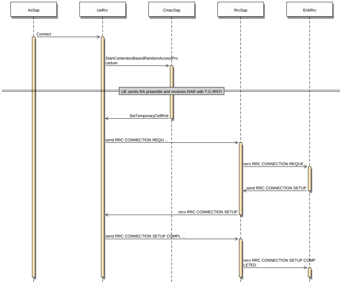
Figure 20.36: Sequence diagram of the RRC Connection Establishment procedure
