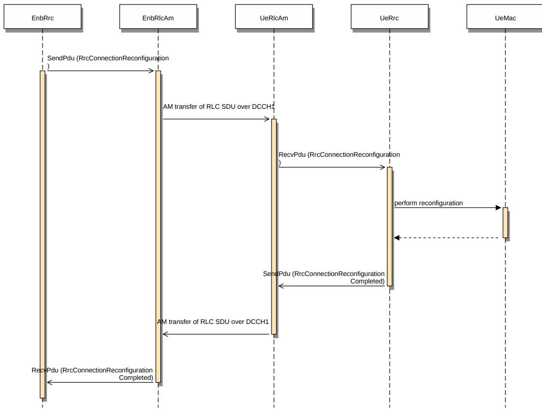
Figure 20.37: Sequence diagram of the RRC Connection Reconfiguration procedure
