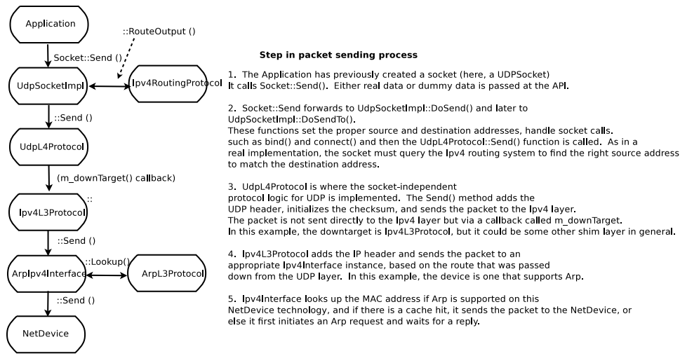
Figure 18.1: Send path of a packet.
