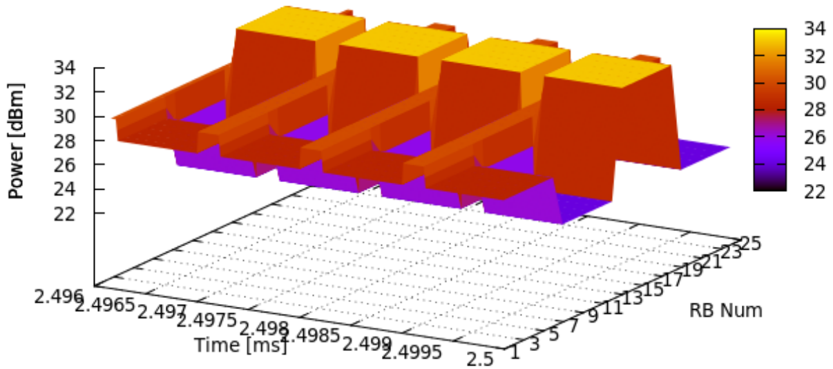
Figure 20.62: Spectrum Analyzer trace obtained from lena-frequency-reuse example with Soft FFR algorithm enabled. Spectrum Analyzer was located near eNB with FrCellTypeId 2.
