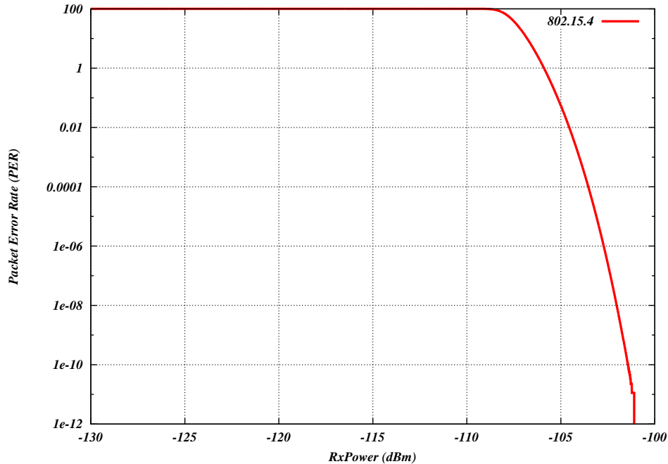
Figure 19.3: Packet error rate vs. signal power
