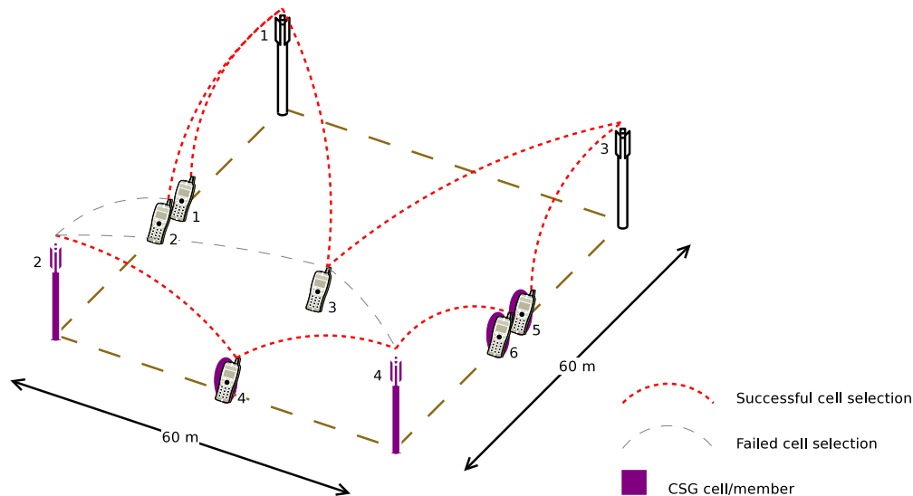
Figure 20.76: Sample result of cell selection test
