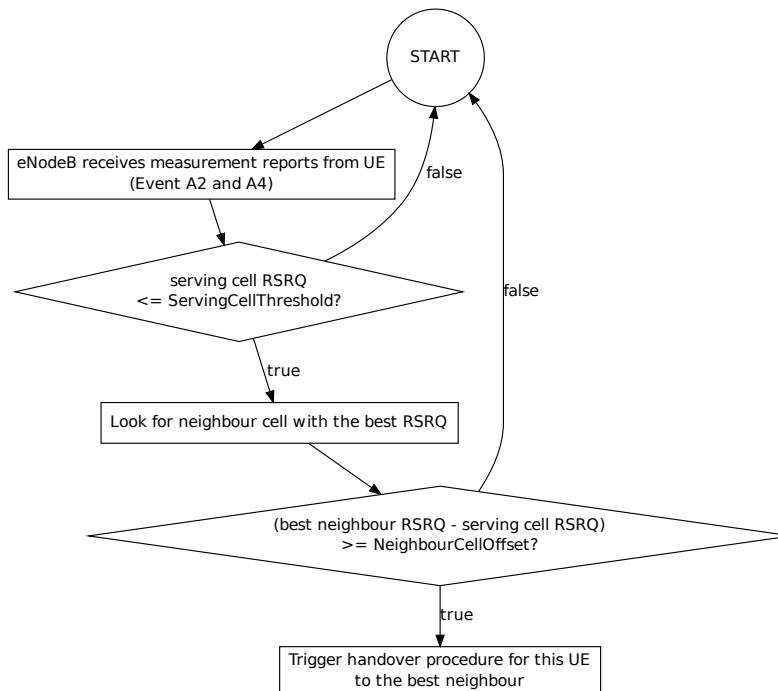
Figure 20.34: A2-A4-RSRQ handover algorithm
