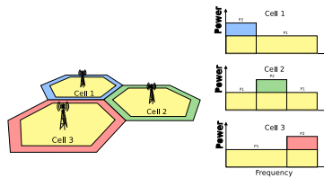
Figure 20.50: Soft Frequency Reuse scheme version 1
