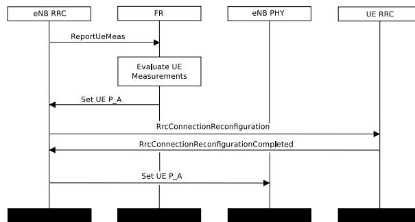
Figure 20.45: Sequence diagram of Downlink Power Control
