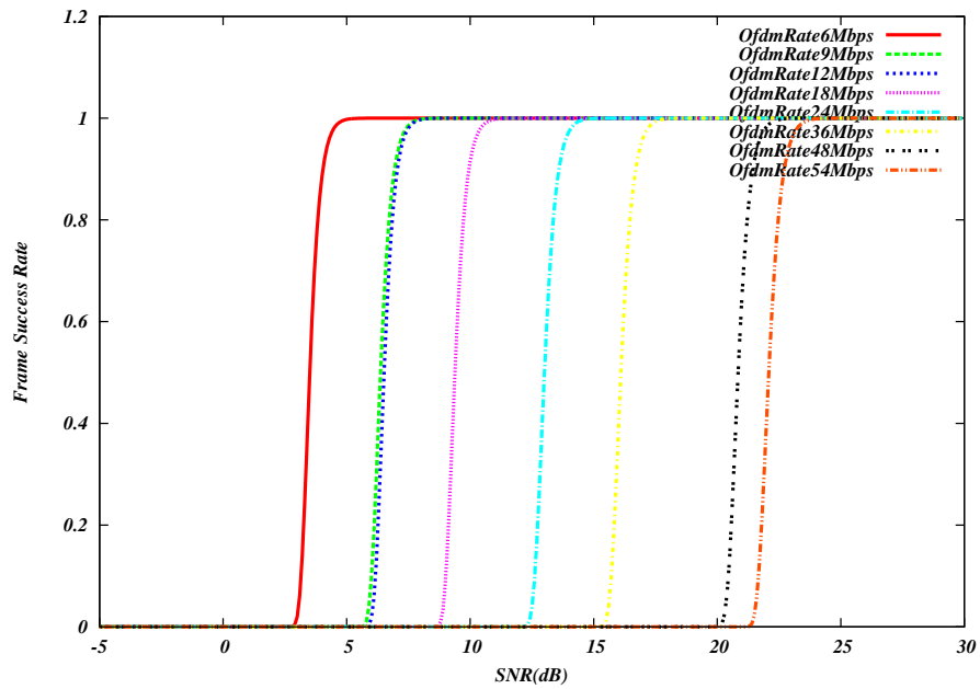
Figure 36.4: Frame error rate (NIST model) for OFDM Wi-Fi
