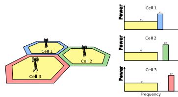
Figure 20.49: Strict Frequency Reuse scheme
