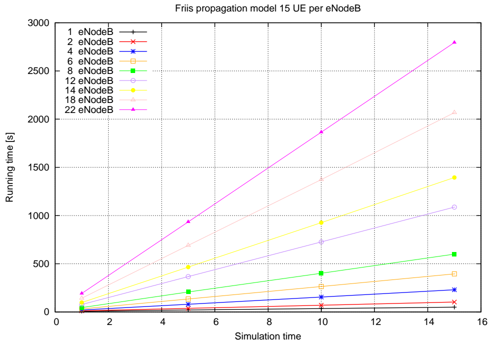
Figure 20.82: Simulation time
