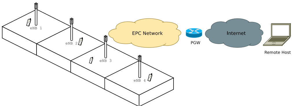
Figure 20.79: Propagation Model
