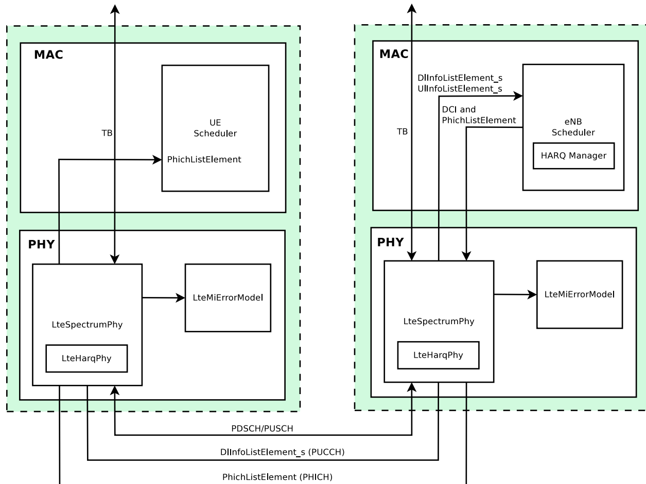
Figure 20.22: Interaction between HARQ and LTE protocol stack
