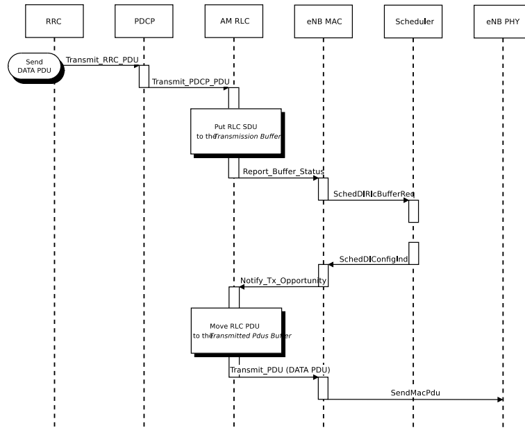
Figure 20.26: Sequence diagram of data PDU transmission in downlink
