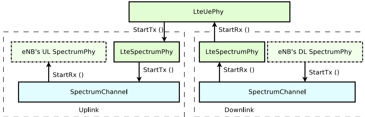
Figure 20.4: PHY and channel model architecture for the UE
