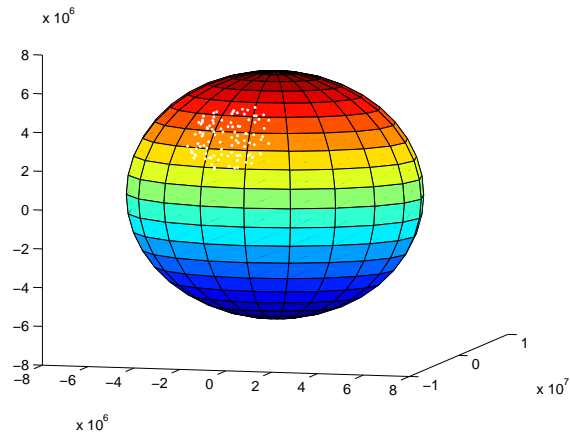
Figure 28.5: Plot from MATLAB implementation of CreateRegionalTvTransmitters method in TvSpectrumTransmitterHelper . Shows 100 random points on Earth's surface (with altitude 0) corresponding to TV transmitter locations within a 2000 km radius of 35^\circ latitude and -100^\circ longitude.
