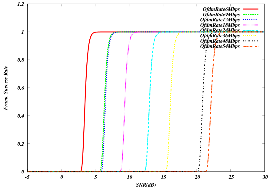
Figure 33.4: Frame error rate (NIST model) for OFDM Wi-Fi
