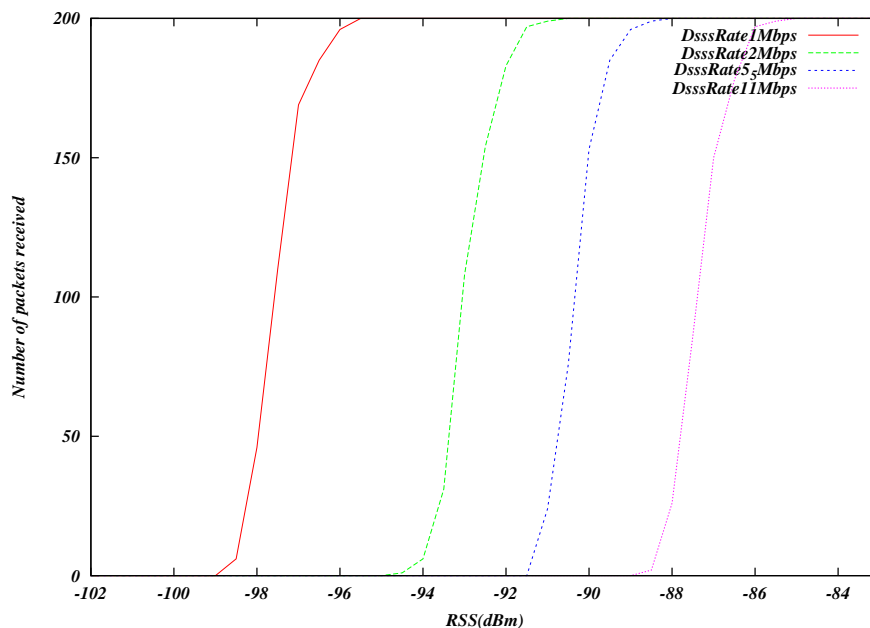
Figure 33.3: Clear channel (AWGN) error model for 802.11b
