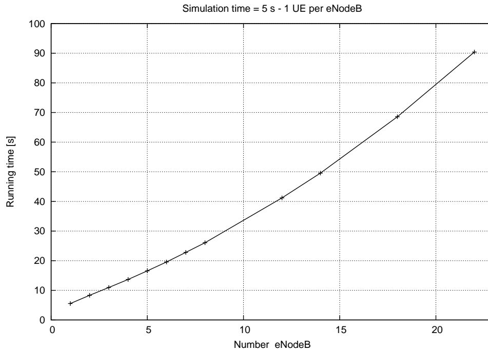
Figure 19.84: Running time
