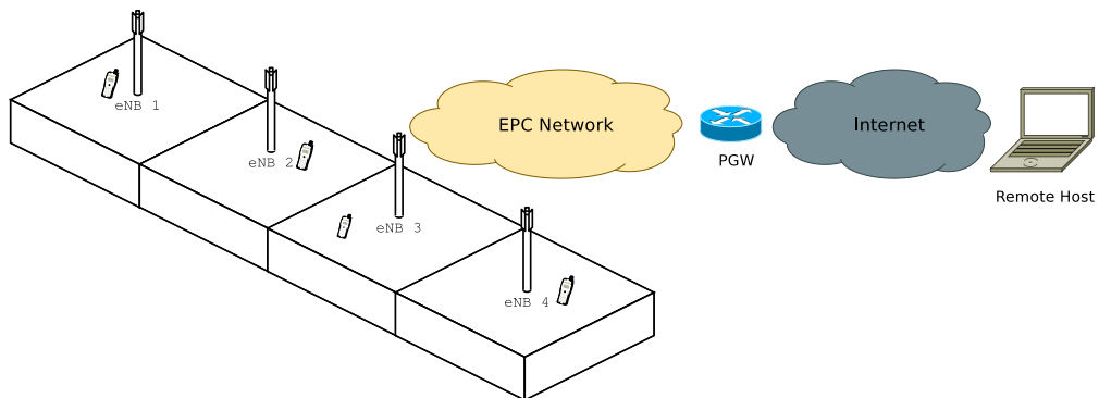
Figure 19.79: Propagation Model
