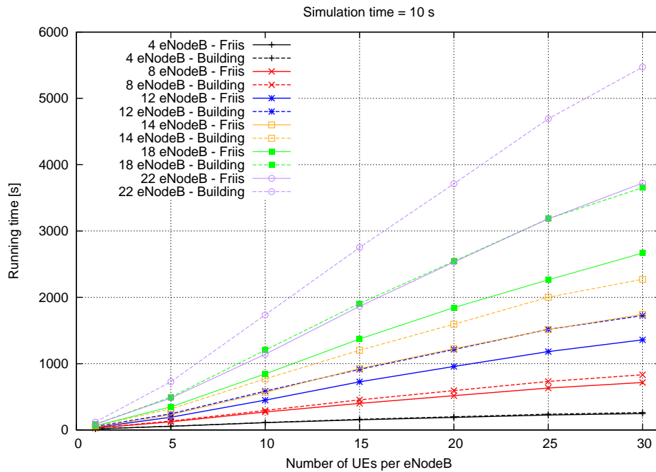
Figure 19.81: Propagation Model
