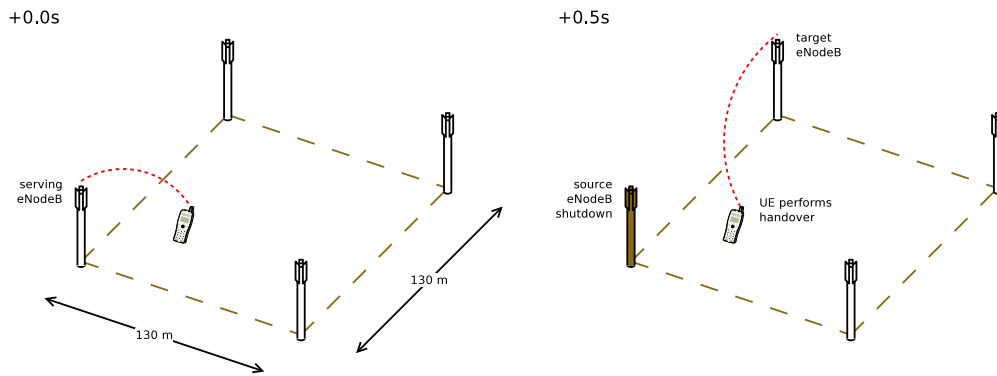
Figure 19.77: lte-handover-target test scenario in a 2x2 grid
