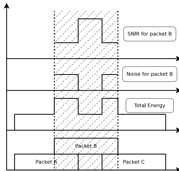
Figure 33.2: SNIR function over time .
