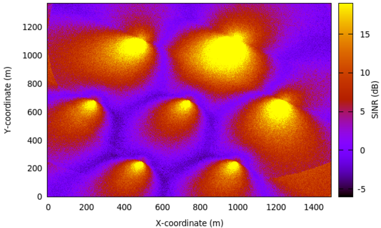
Figure 19.65: REM for RB 20 obtained from lena-dual-stripe simulation with Hard FR algorithm enabled
