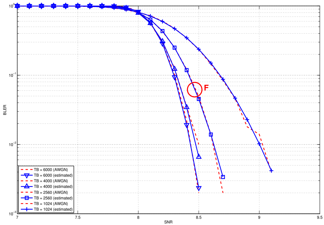
Figure 19.75: BLER for test 6.
