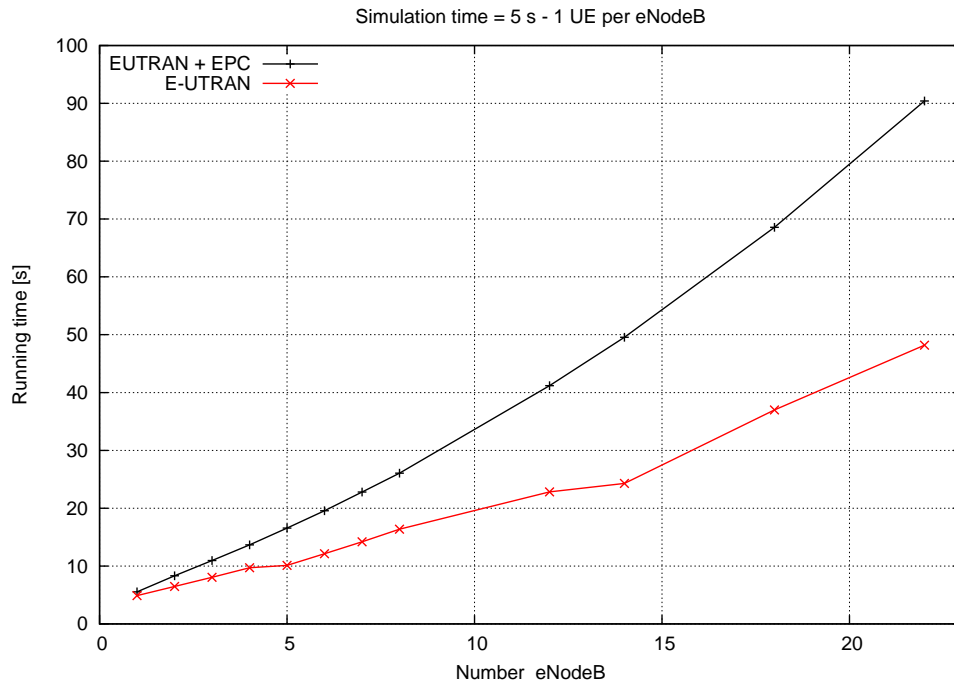
Figure 19.85: EPC E-UTRAN running time
