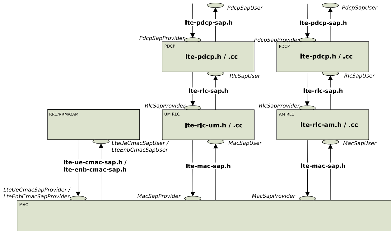
Figure 19.25: Implementation Model of PDCP, RLC and MAC entities and SAPs
