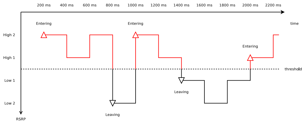
Figure 19.69: Measured RSRP trace of an example Event A1 test case in piecewise configuration
