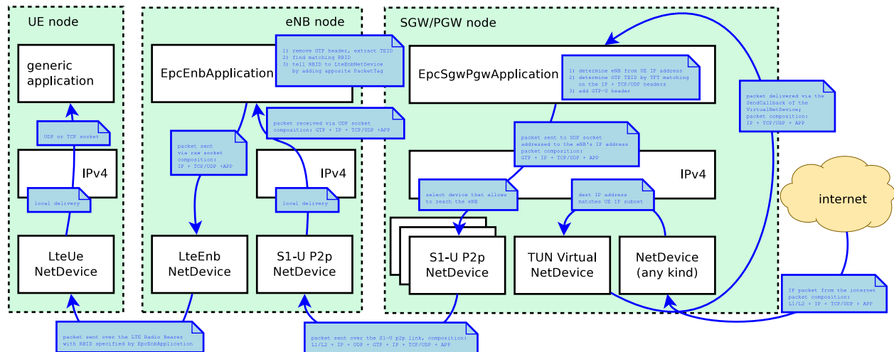
Figure 19.40: Data flow in the downlink between the internet and the UE
