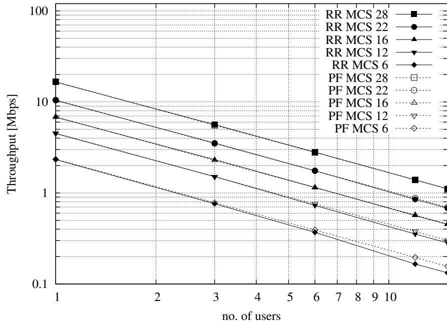
Figure 19.71: Test vectors for the RR and PF Scheduler in the downlink in a scenario where all UEs use the same MCS.
