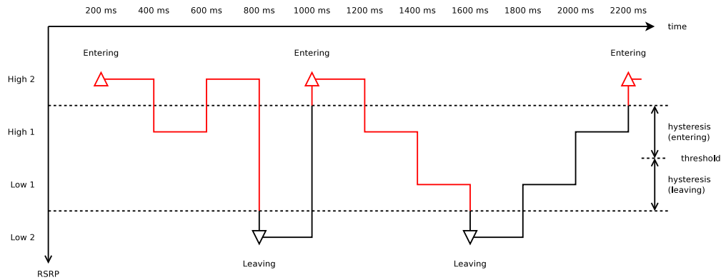
Figure 19.70: Measured RSRP trace of an example Event A1 with hysteresis test case in piecewise configuration
