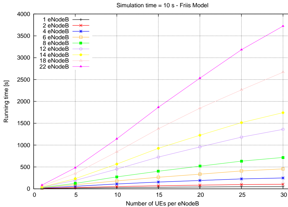
Figure 19.80: Running time
