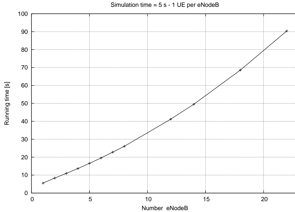
Figure 19.84: Running time
