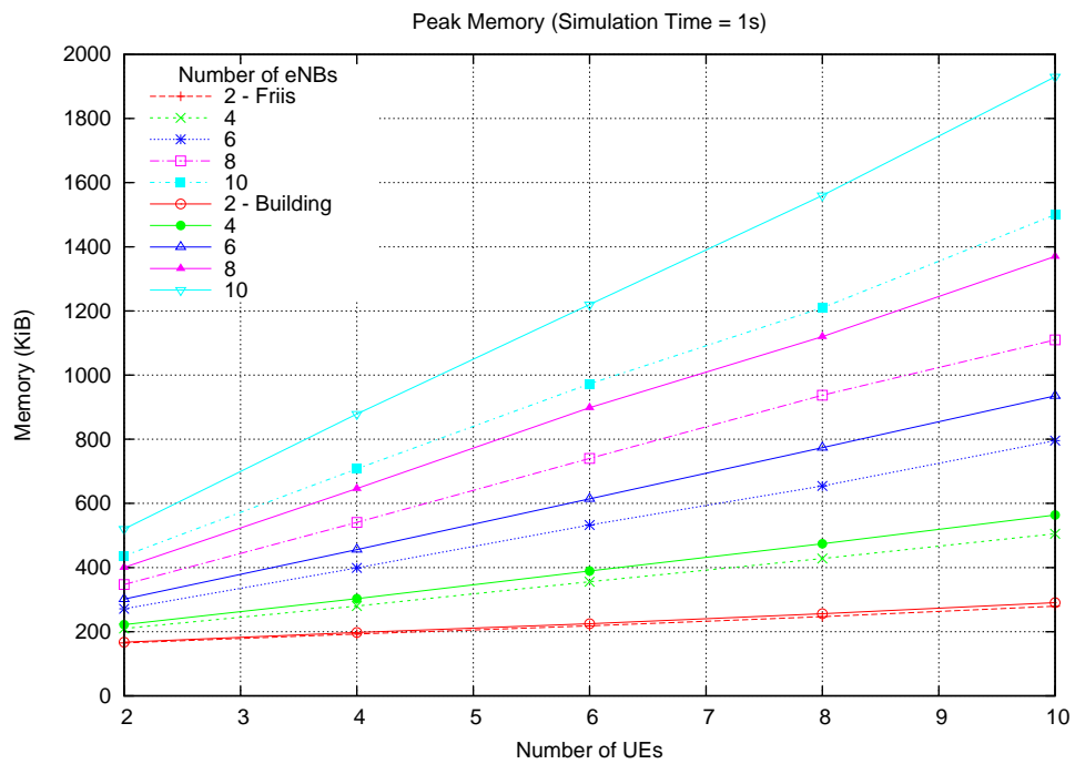
Figure 19.83: Memory profile
