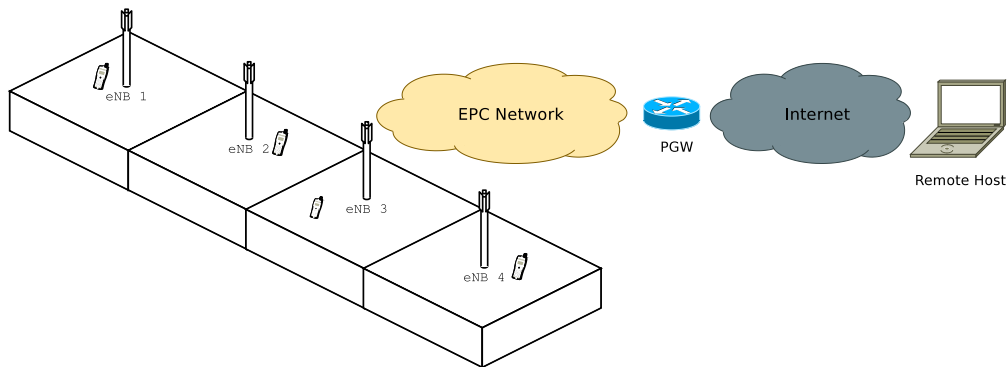
Figure 19.79: Propagation Model
