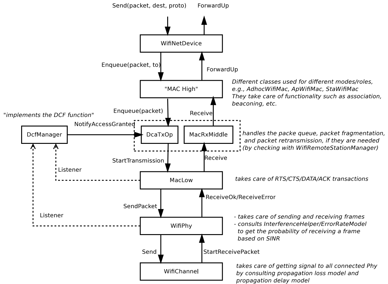
Figure 33.1: WifiNetDevice architecture.
