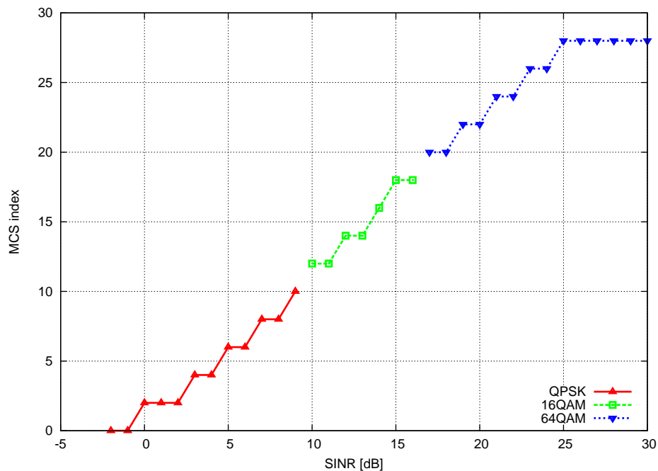
Figure 19.66: Test vector for Adaptive Modulation and Coding
