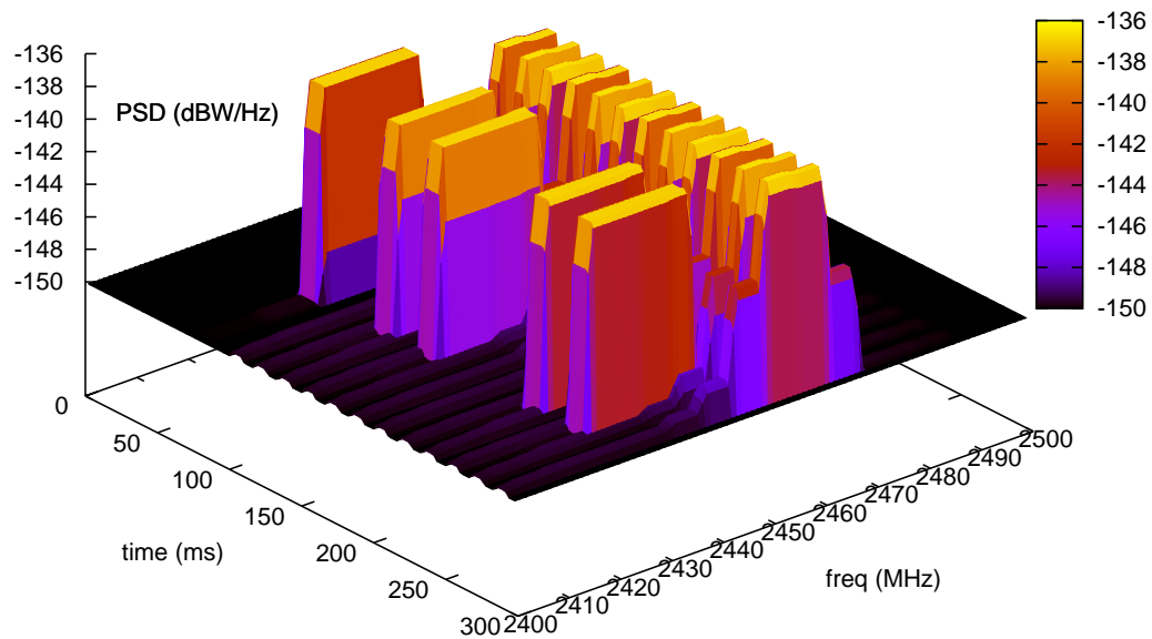
Figure 28.1: Spectrogram produced by a spectrum analyzer in a scenario involving wifi signals interfered by a microwave oven, as simulated by the example adhoc-aloah-ideal-phy-with-microwave-oven .
