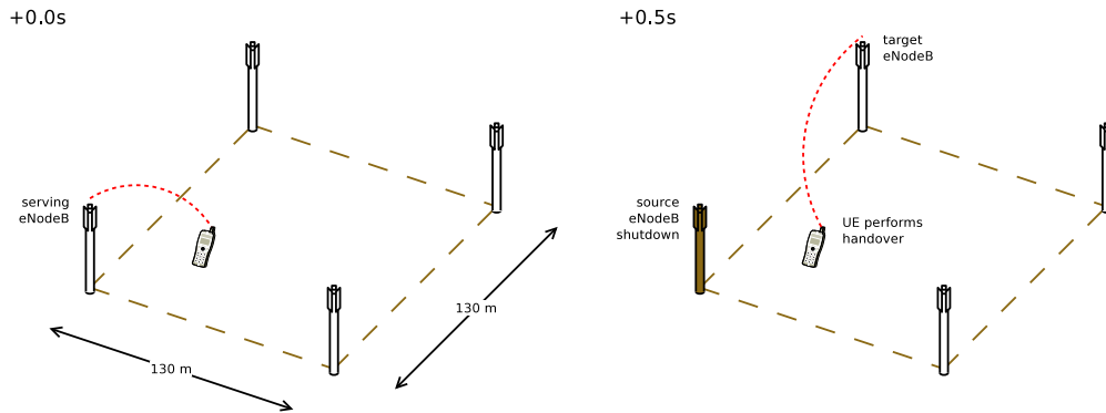
Figure 19.77: lte-handover-target test scenario in a 2x2 grid
