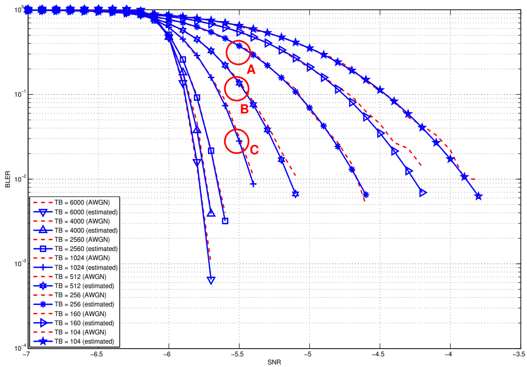
Figure 19.73: BLER for tests 1, 2, 3.
