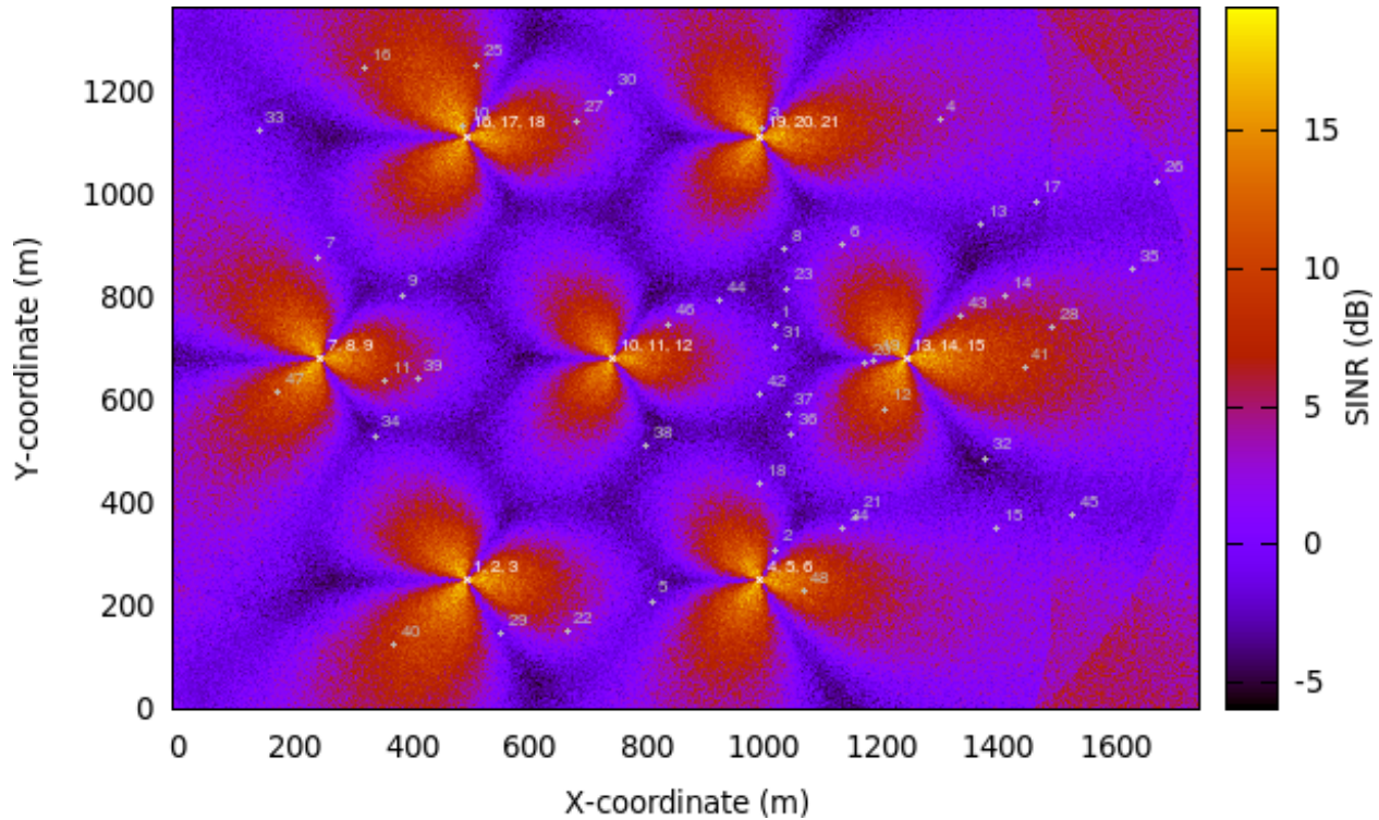
Figure 19.60: REM obtained from a simulation in handover campaign
