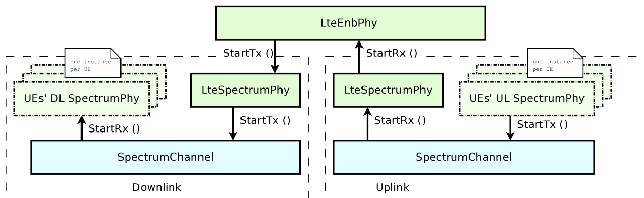
Figure 19.7: PHY and channel model architecture for the eNB
