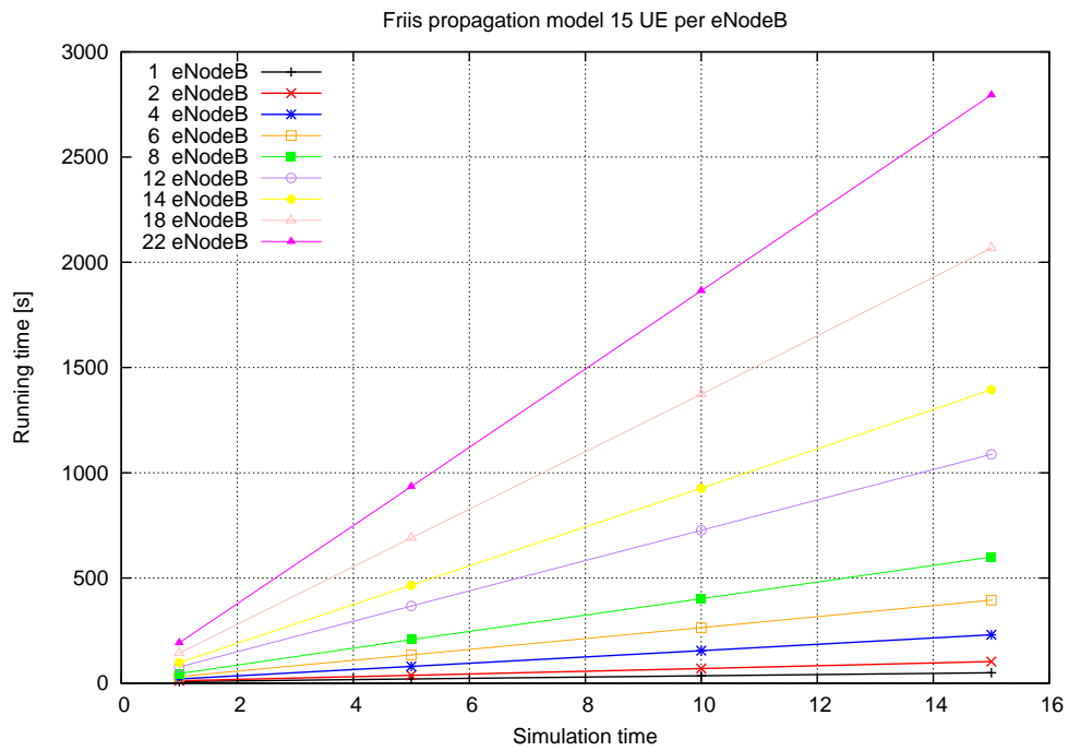
Figure 19.82: Simulation time
