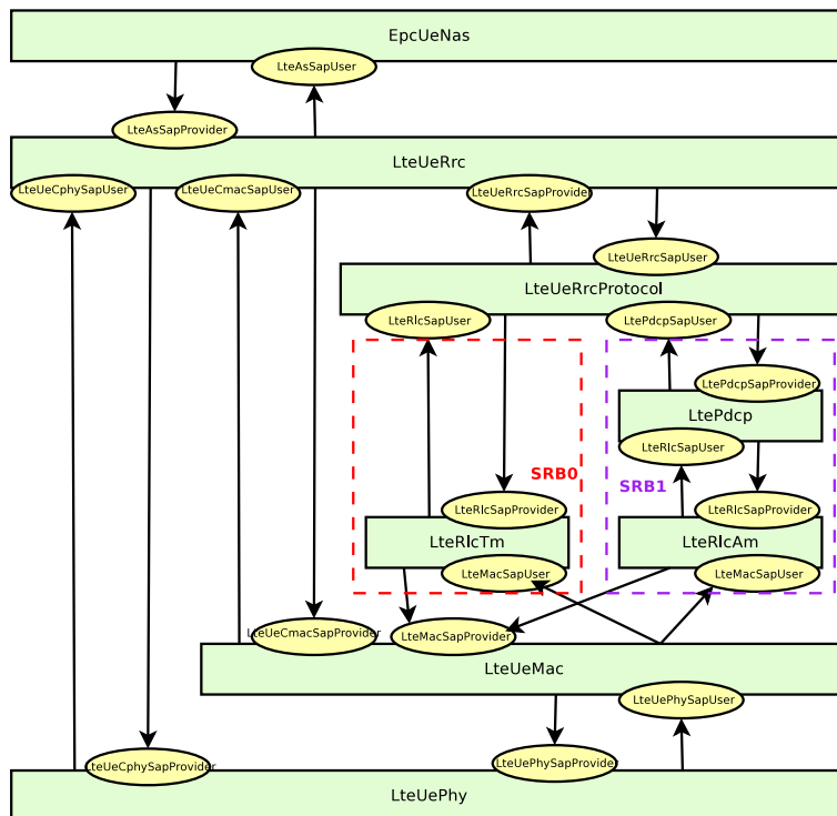
Figure 19.3: LTE radio protocol stack architecture for the UE on the control plane
