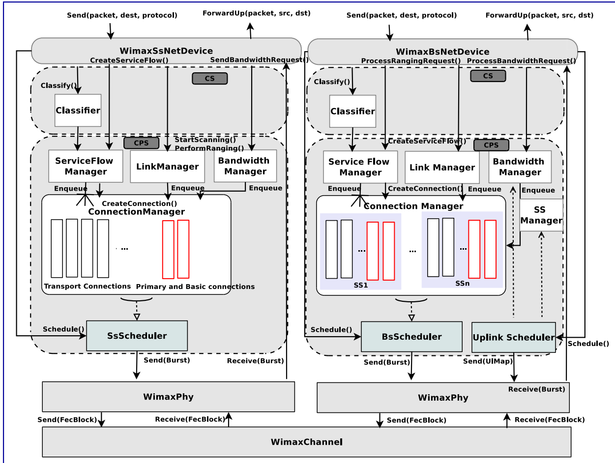
Figure 34.1: WiMAX architecture
