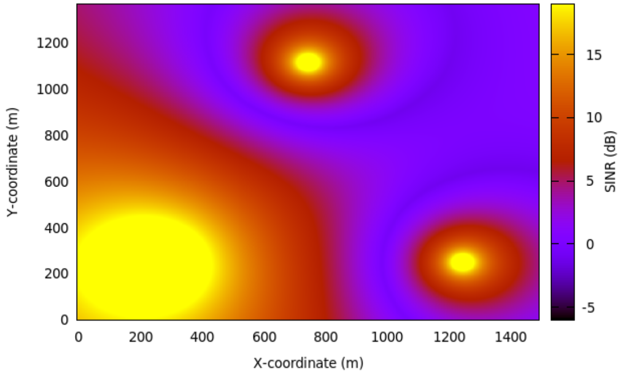
Figure 19.61: REM for RB 1 obtained from lena-frequency-reuse example with Soft FR algorithm enabled
