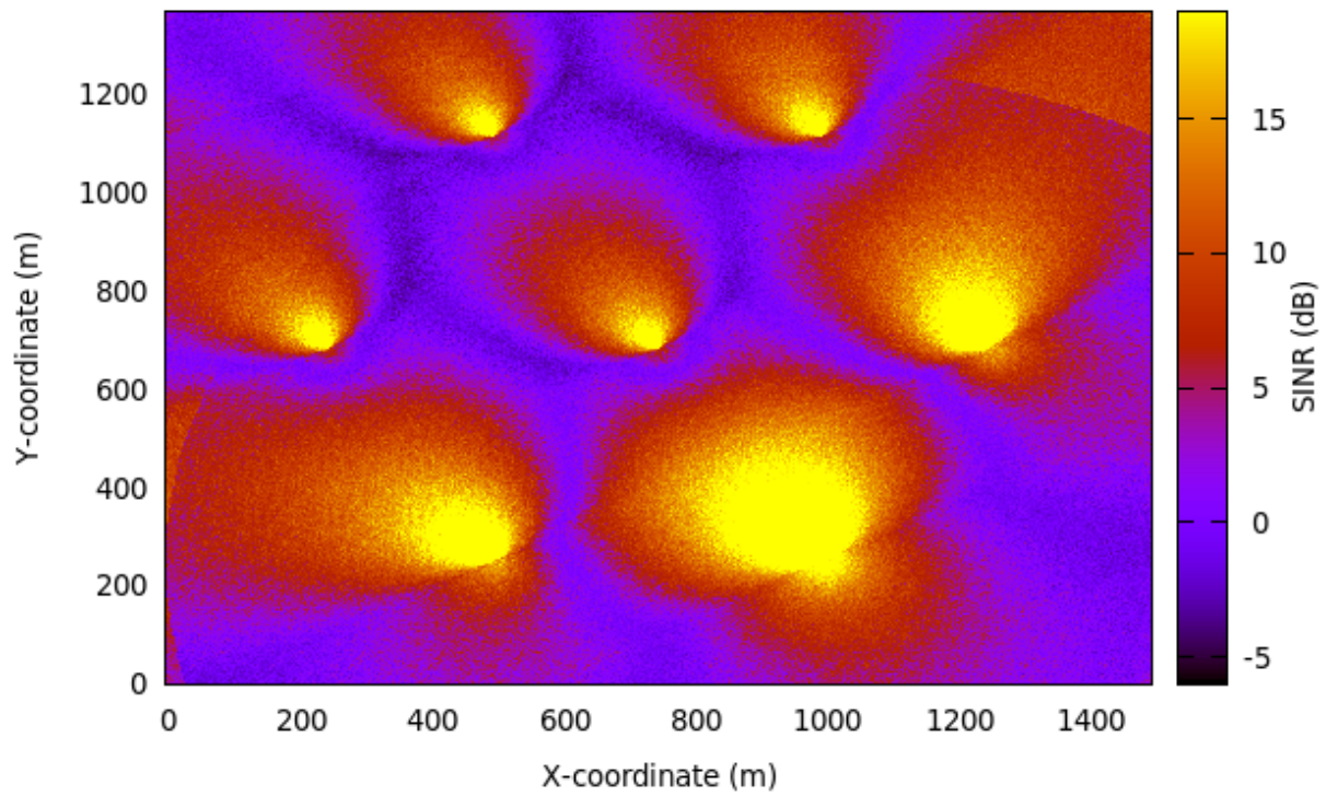
Figure 19.64: REM for RB 10 obtained from lena-dual-stripe simulation with Hard FR algorithm enabled
