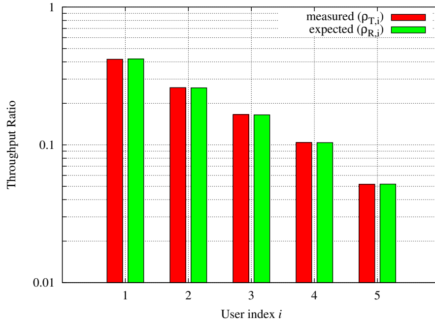
Figure 19.72: Throughput ratio evaluation for the PF scheduler in a scenario where the UEs have MCS index 28, 24, 16, 12, 6
