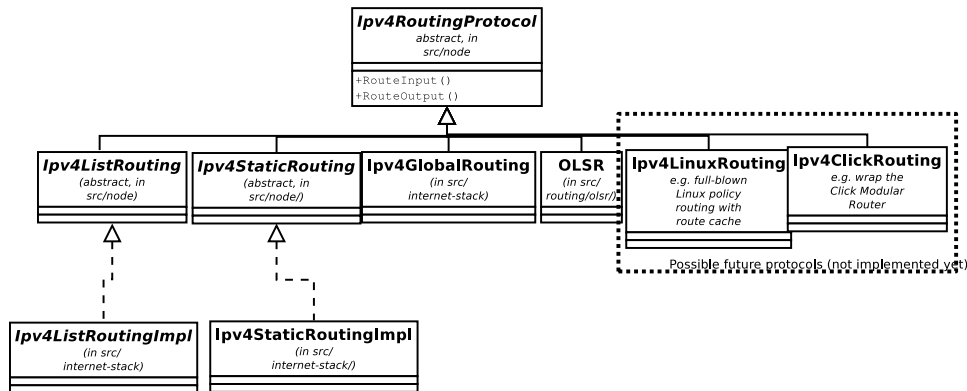
Figure 17.4: Ipv4Routing specialization.
