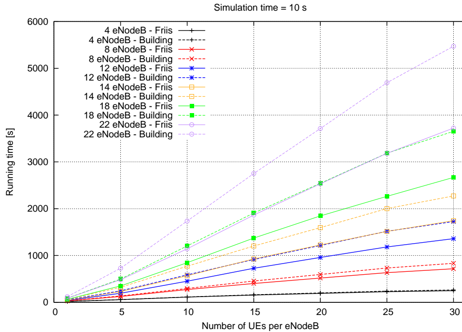
Figure 19.81: Propagation Model
