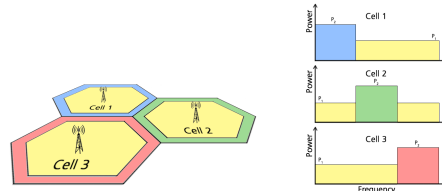
Figure 19.51: Soft Frequency Reuse scheme version 2
