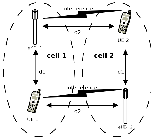
Figure 19.67: Topology for the inter-cell interference test
