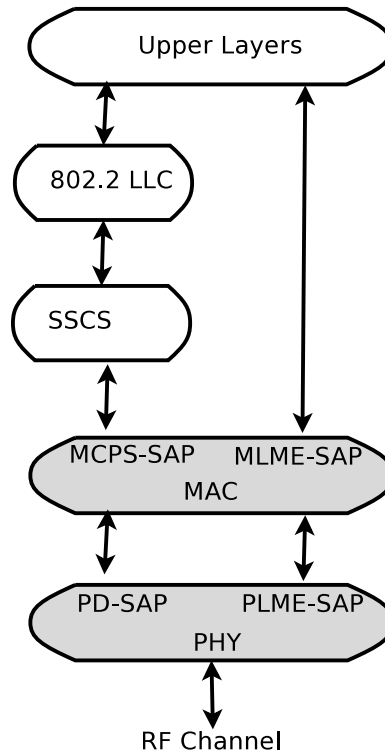
Figure 18.1: Architecture and scope of Ir-wpan models
