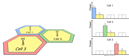
Figure 19.53: Enhanced Fractional Fractional Frequency Reuse scheme
