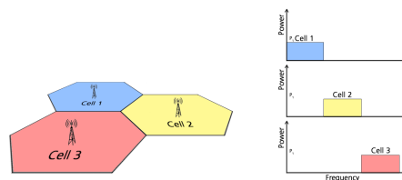
Figure 19.48: Hard Frequency Reuse scheme
