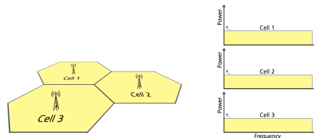
Figure 19.47: Full Frequency Reuse scheme
