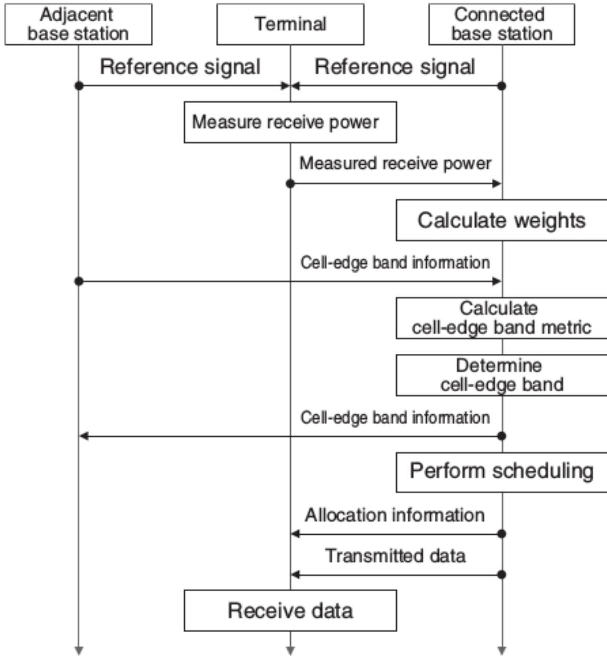
Figure 19.54: Sequence diagram of Distributed Frequency Reuse Scheme
