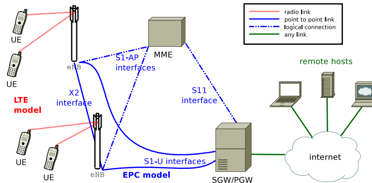
Figure 19.1: Overview of the LTE-EPC simulation model
