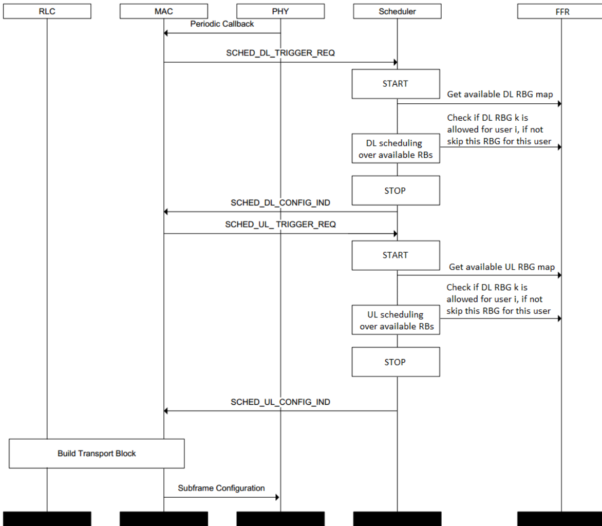
Figure 19.46: Sequence diagram of Scheduling with FR algorithm
