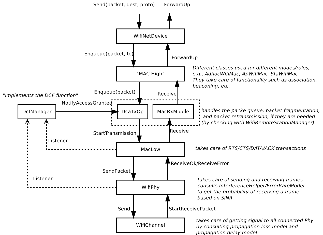
Figure 33.1: WifiNetDevice architecture.
