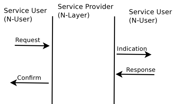
Figure 18.2: Service primitives
