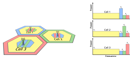
Figure 19.52: Soft Fractional Fractional Frequency Reuse scheme
