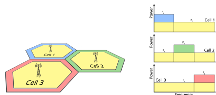
Figure 19.50: Soft Frequency Reuse scheme version 1
