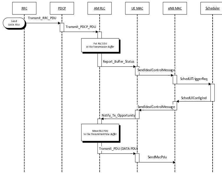
Figure 19.28: Sequence diagram of data PDU transmission in uplink
