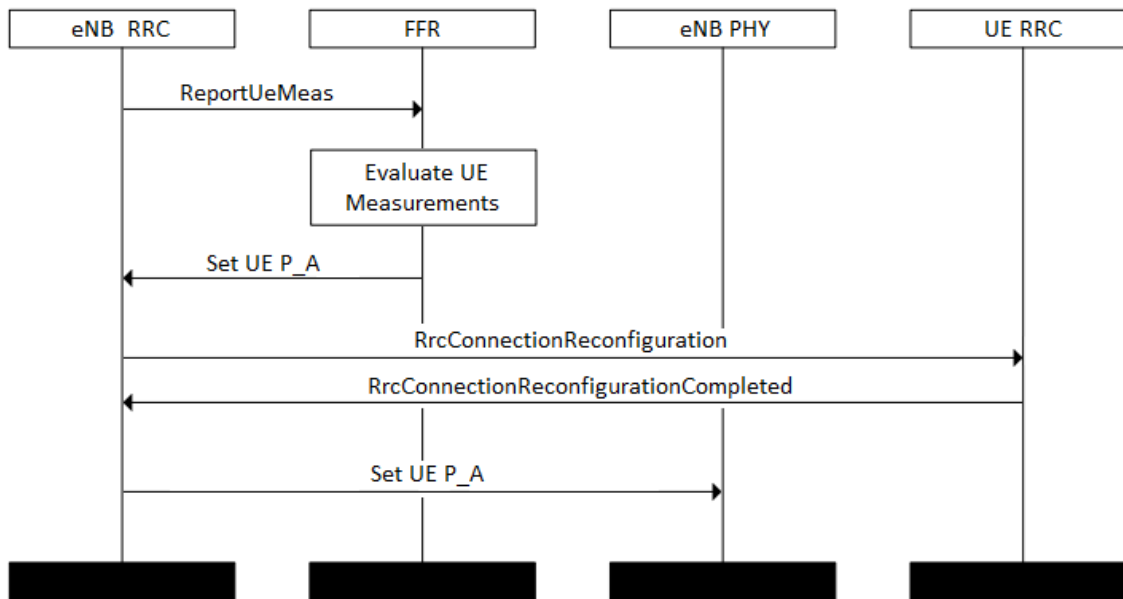
Figure 19.45: Sequence diagram of Downlink Power Control
