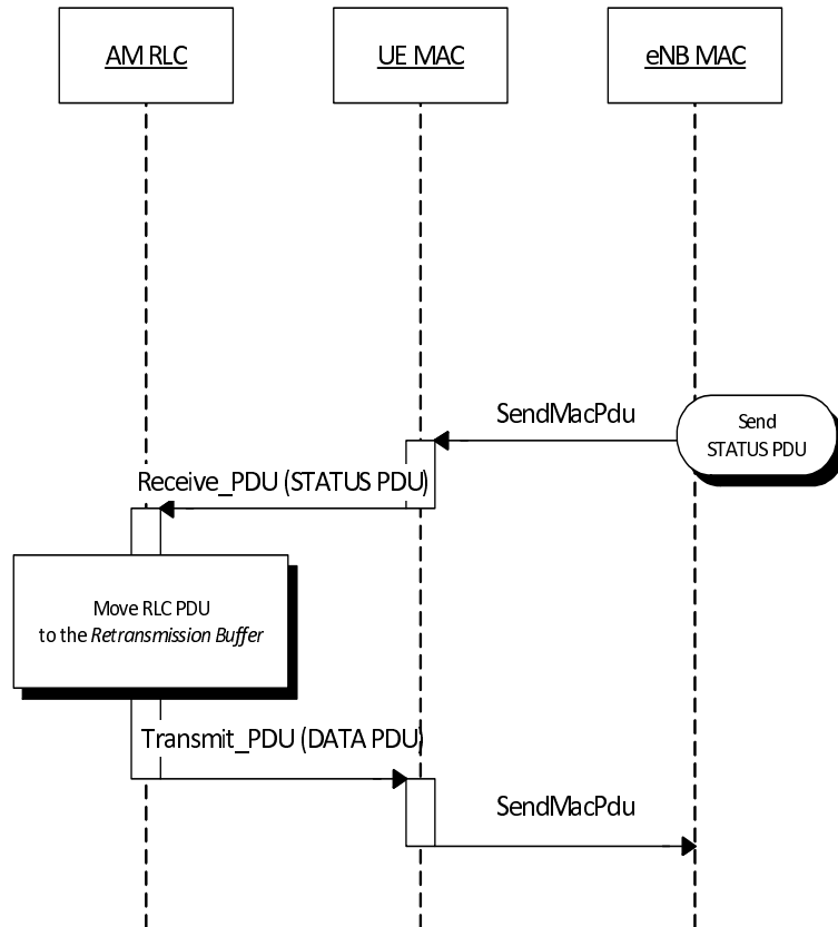
Figure 19.29: Sequence diagram of data PDU retransmission in uplink
