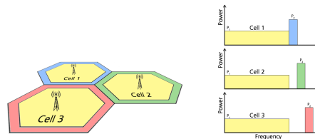
Figure 19.49: Strict Frequency Reuse scheme
