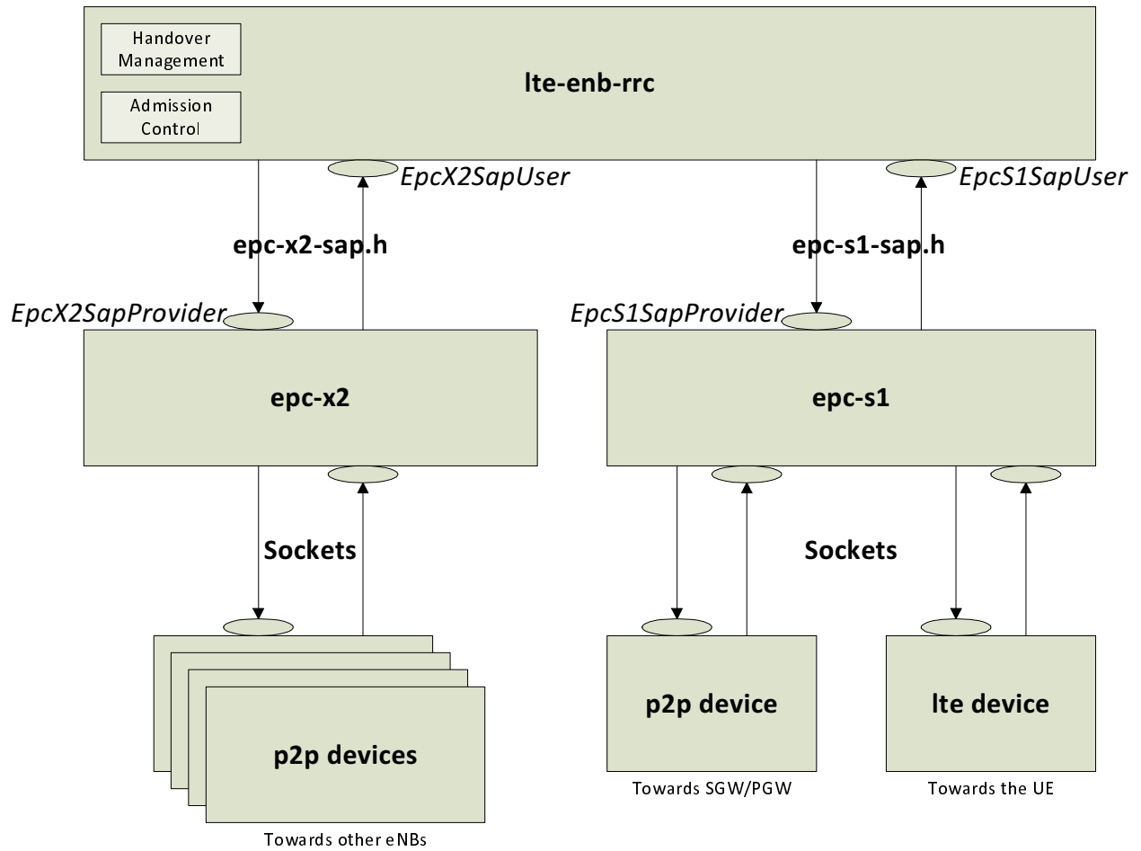
Figure 19.43: Implementation Model of X2 entity and SAPs
