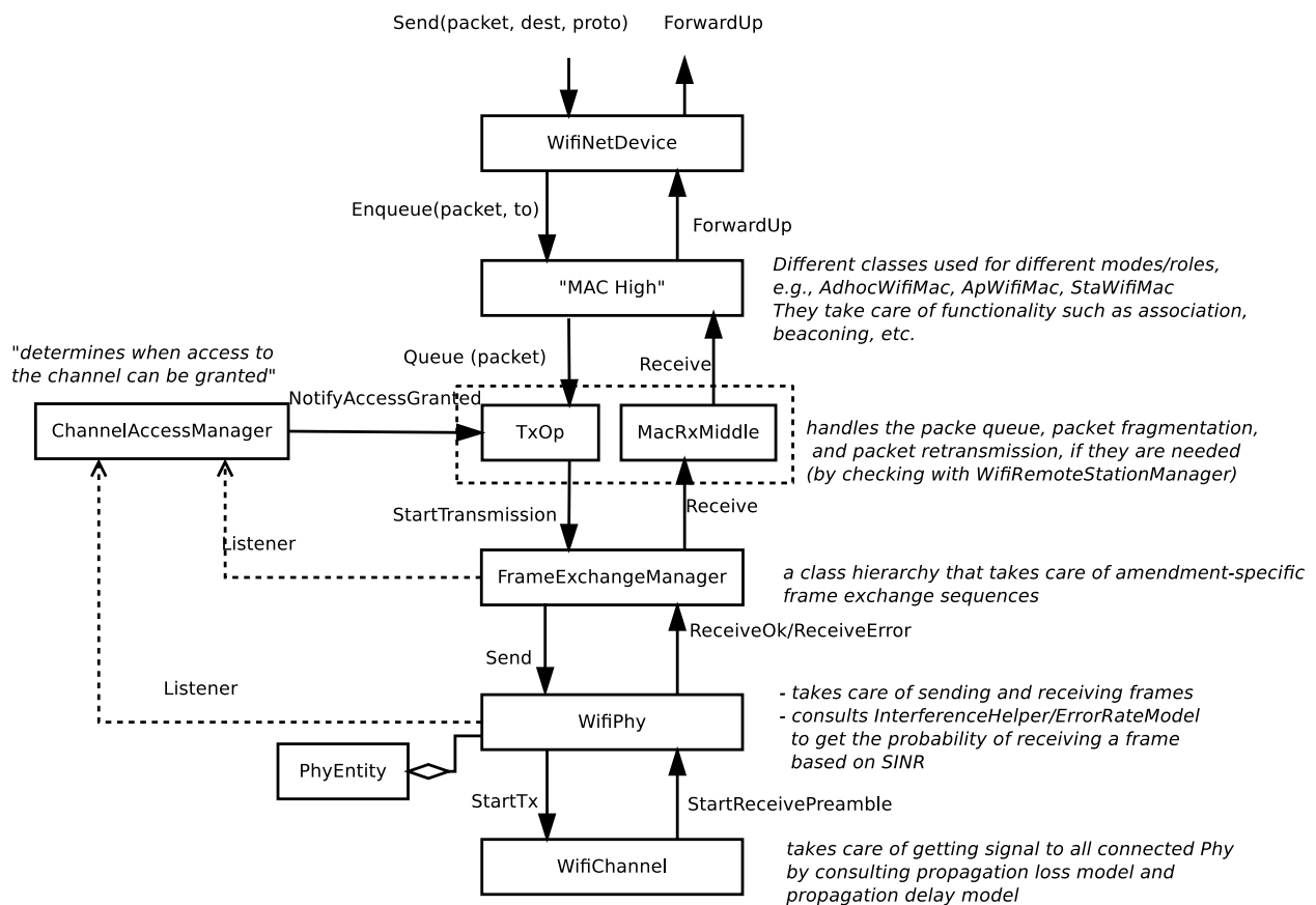
Fig. 1: WifiNetDevice architecture
