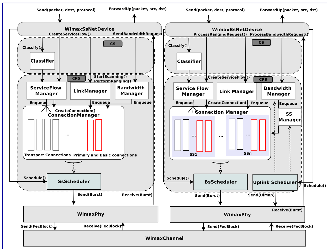
Fig. 1: WiMAX architecture
