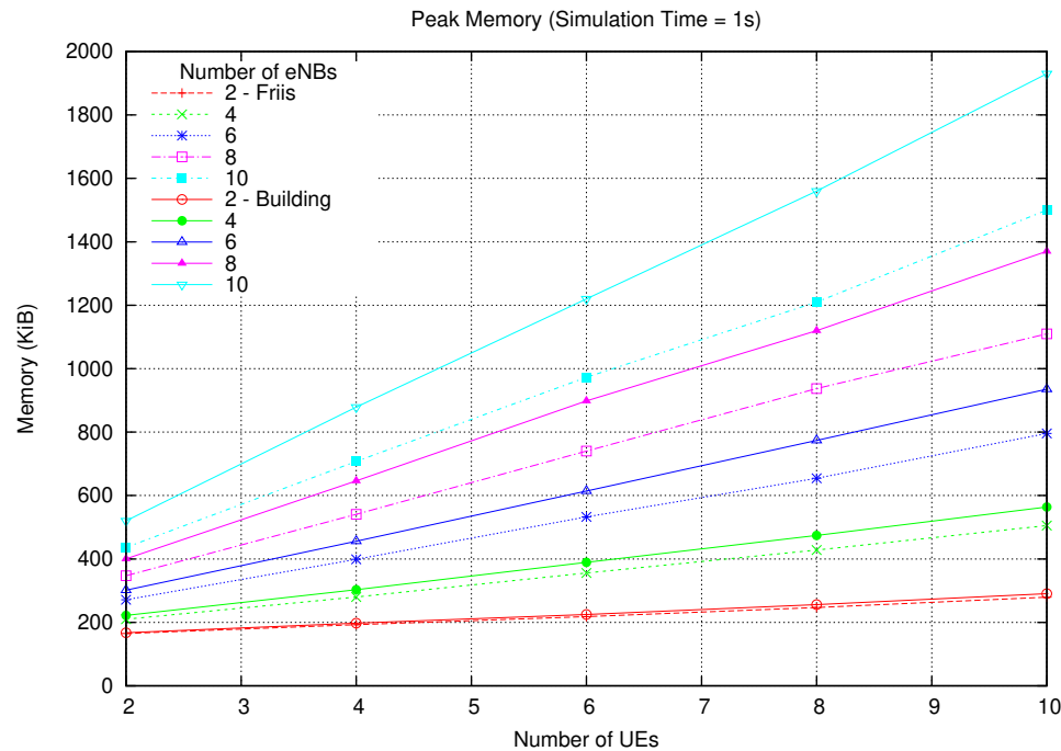
Fig. 106: Memory profile
